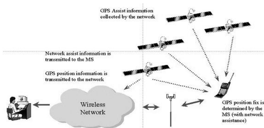
Figure 2.3. Assisted-GPS Technique
