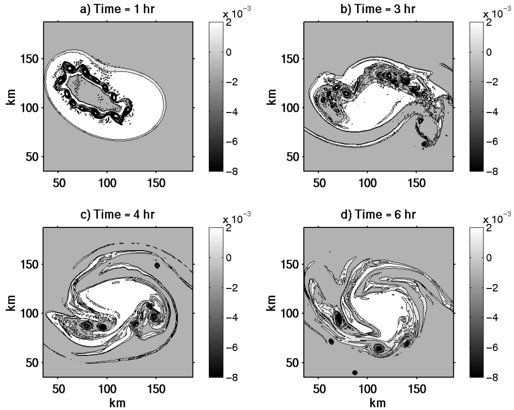
Figure 9. Vorticity fields for Experiment B at a) one hour, b) three hours, c) four hours, and d) six hours.
