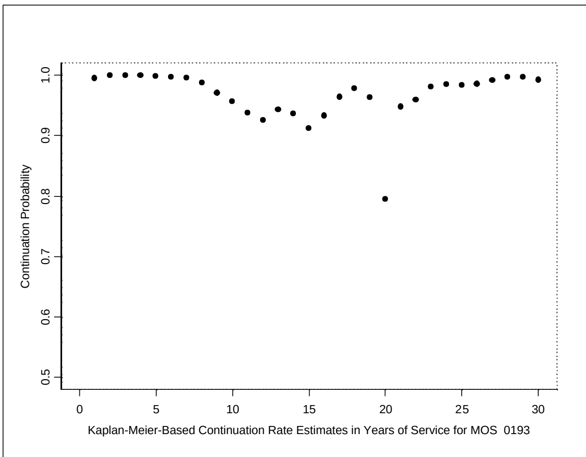
Figure 10. MOS 0193 Continuation Rate Estimates
