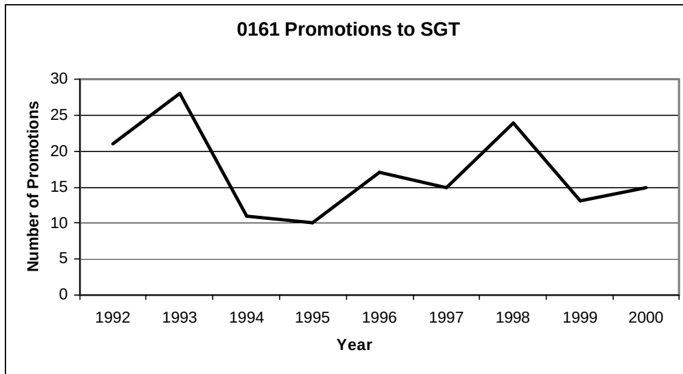
Figure 3. Sgt Promotions 1992-2000 for MOS 0161
