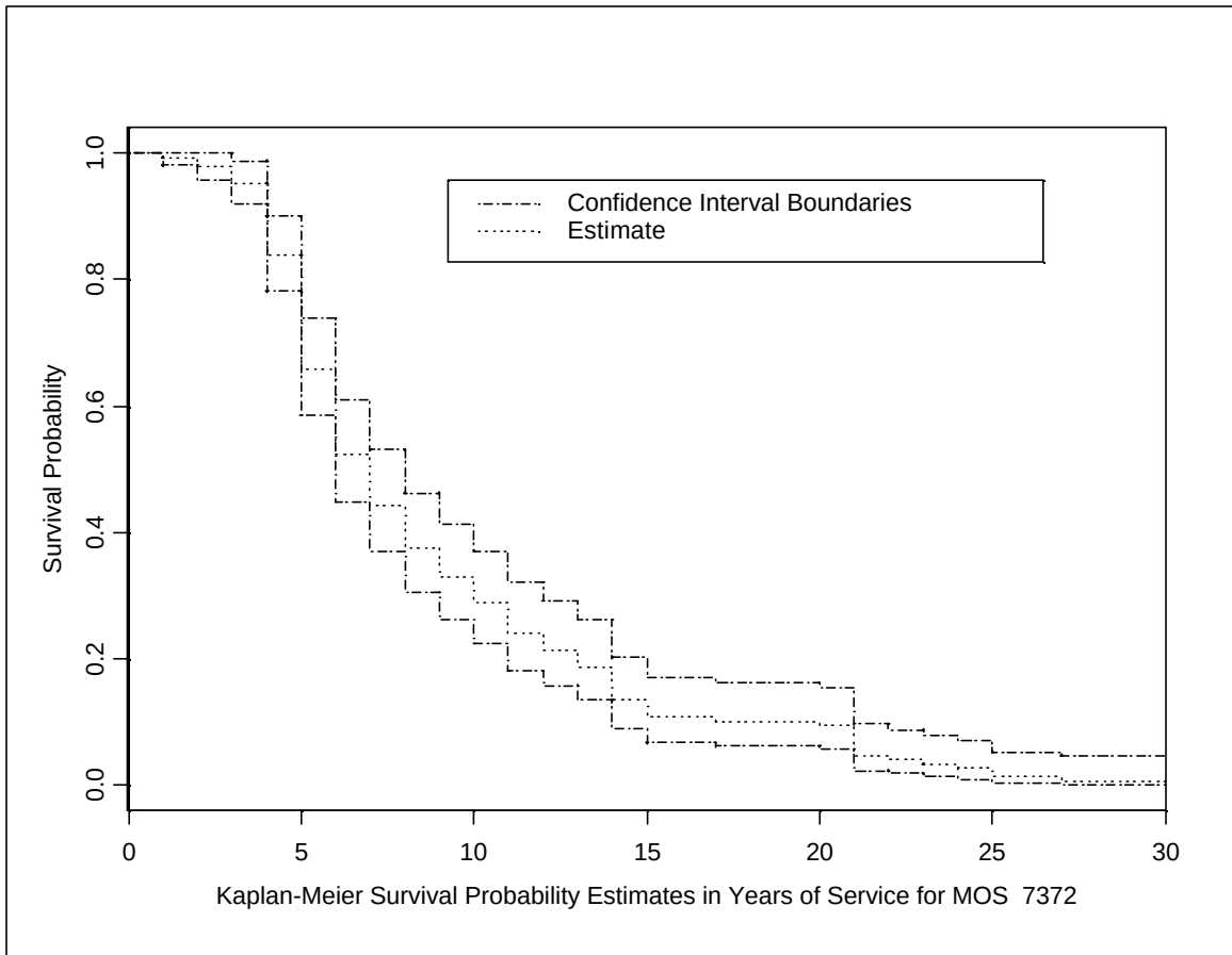
Figure 5. MOS 7372 Survival Probability Estimates
