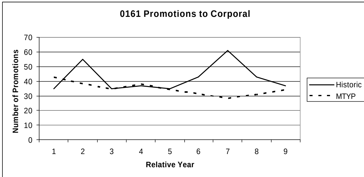
Figure 14. MOS 0161 Corporal Promotions
