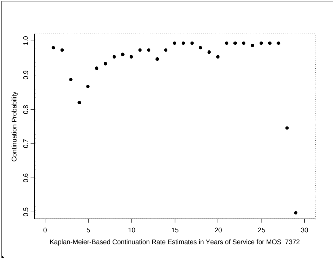
Figure 6. MOS 7372 Continuation Rate Estimates
