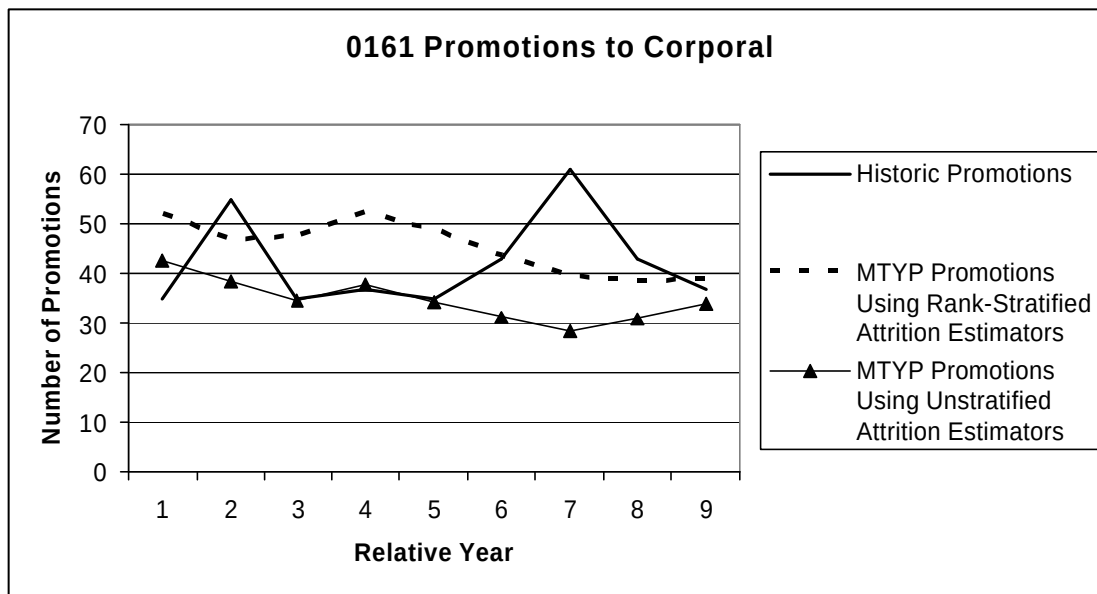
Figure 17. Rank-Stratified and Unstratified 0161 Corporal Promotions
