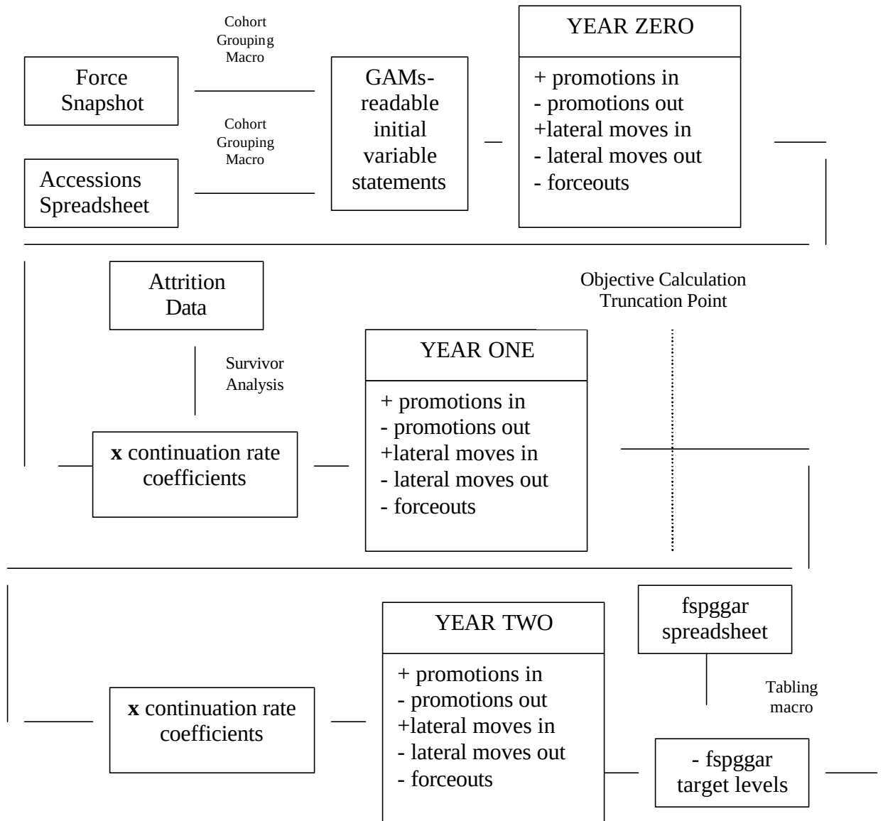
Figure 19. Data flow and Calculation Architecture
