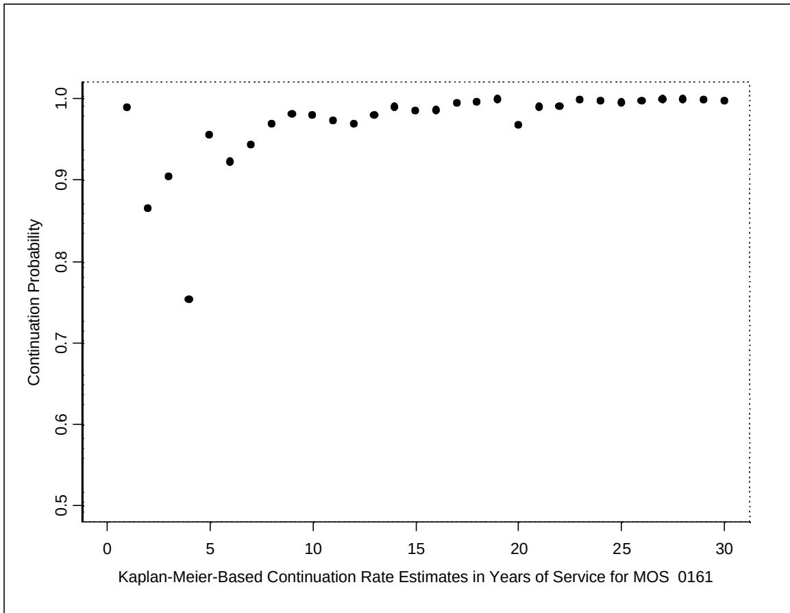
Figure 8. MOS 0161 Continuation Rate Estimates
