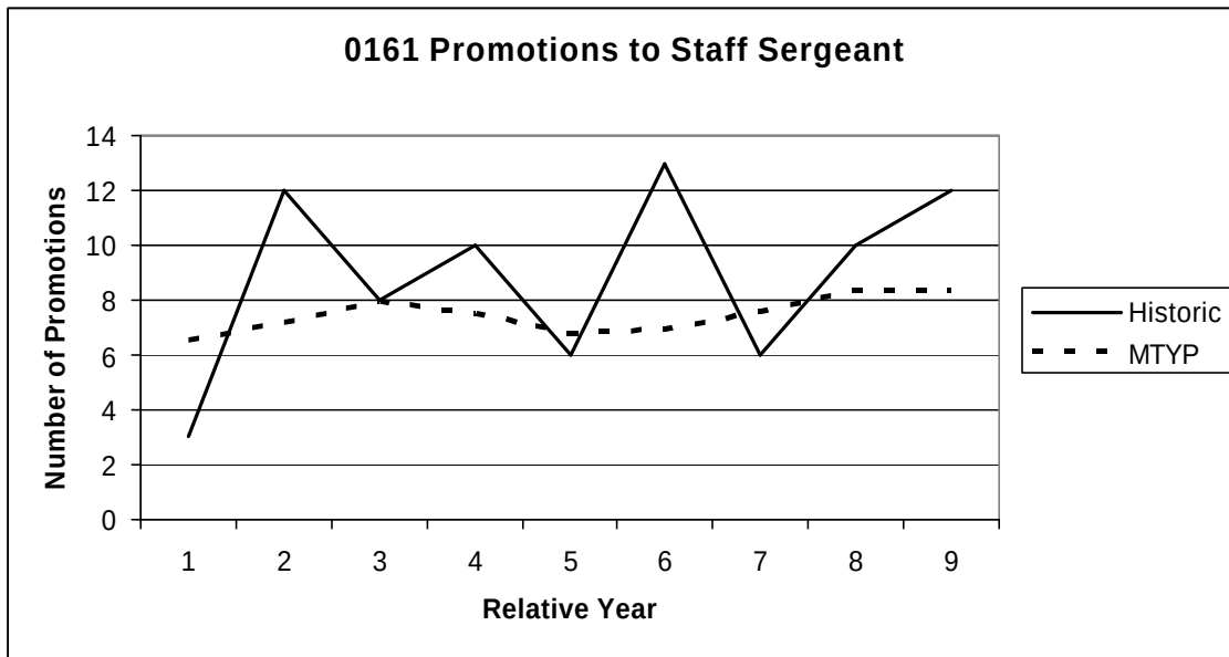
Figure 16. MOS 0161 Staff Sergeant Promotions
