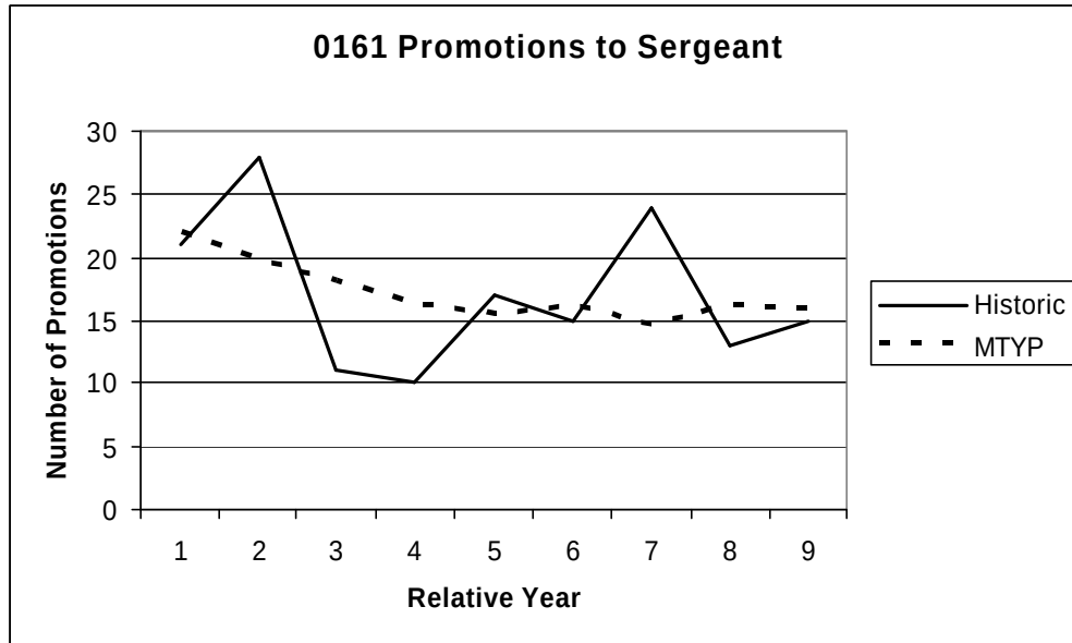
Figure 15. MOS 0161 Sergeant Promotions
