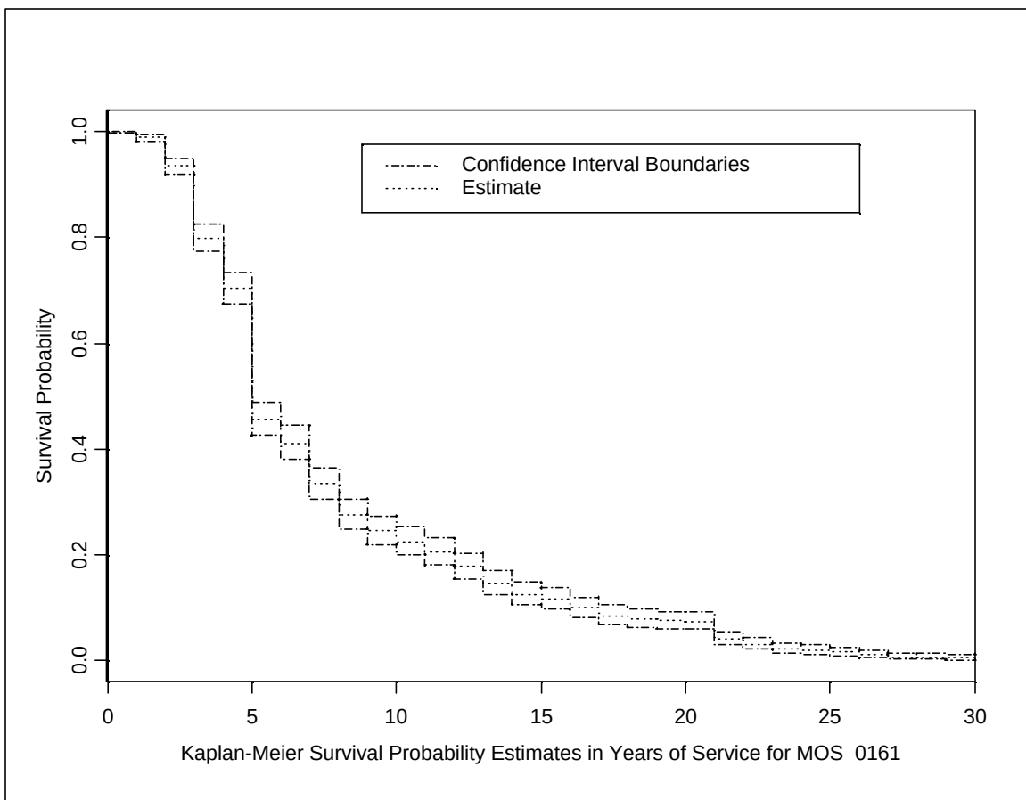
Figure 7. MOS 0161 Survival Probability Estimates
