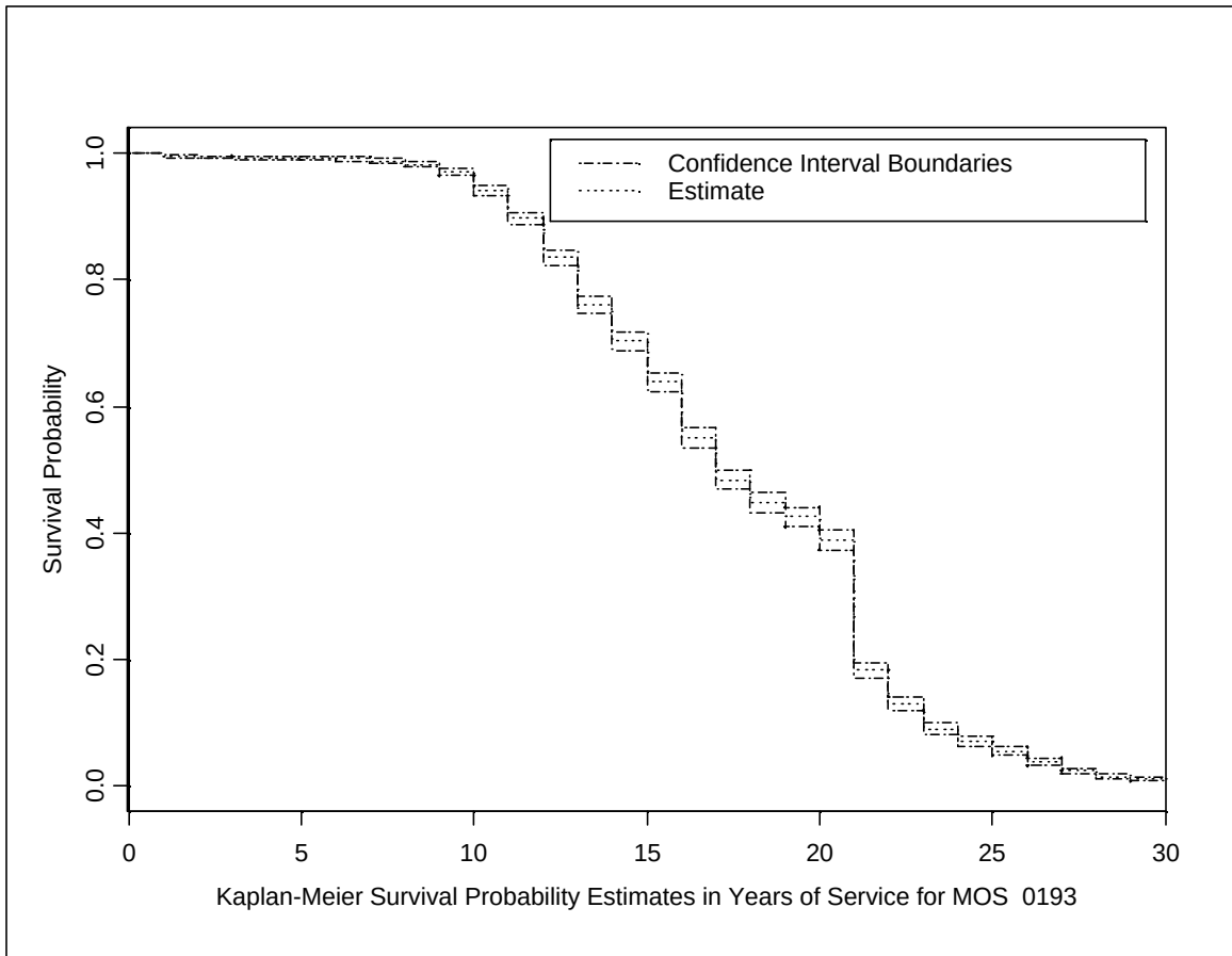
Figure 9. MOS 0193 Survival Probability Estimates
