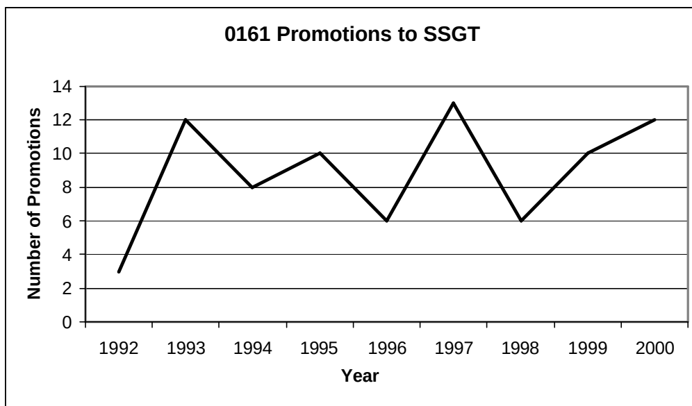
Figure 2. SSgt Promotions 1992-2000 for MOS 0161
