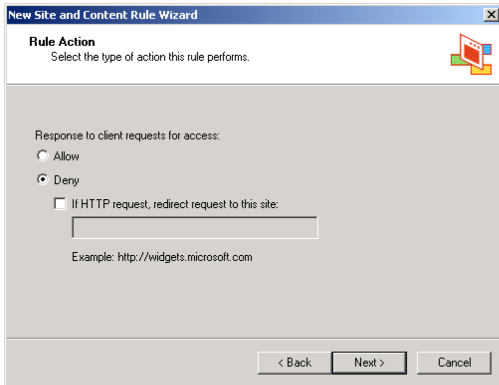
Figure 19 -- Allow And Deny Rules
