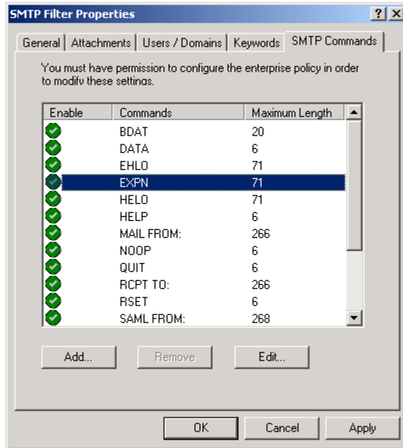
Figure 41 -- SMTP Commands
