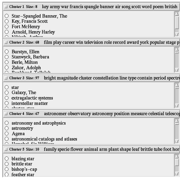
Figure 8. Scatter/Gather Interface
