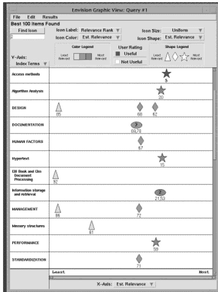
Figure 14. Envision Interface
