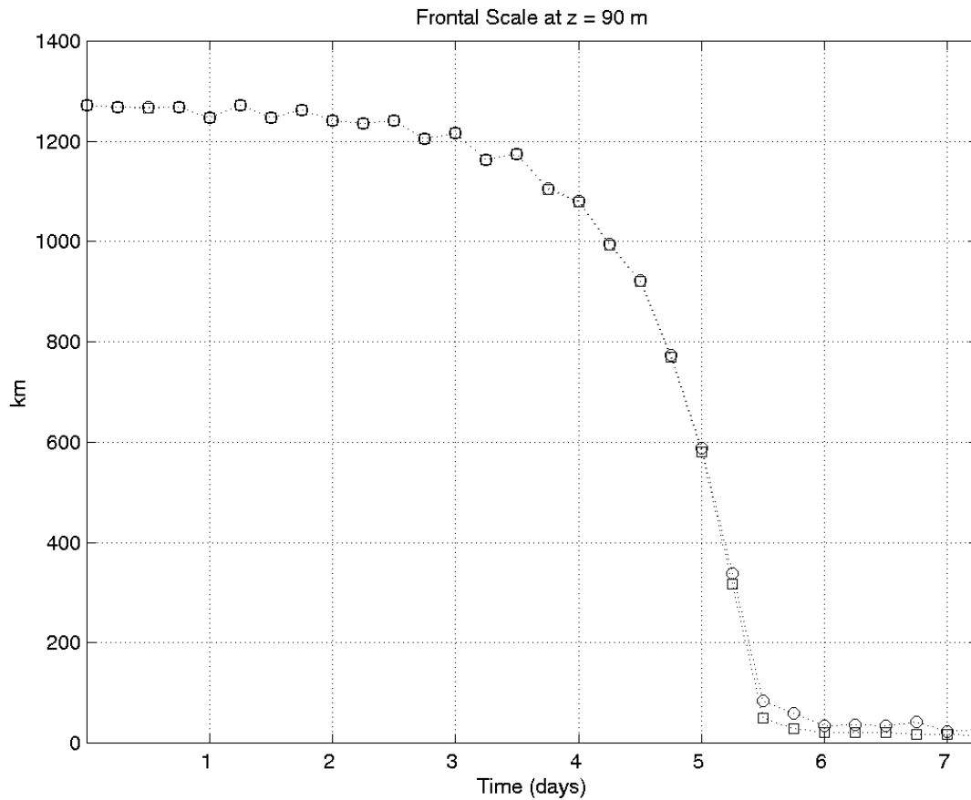
Figure 8. Frontal scale at z = 90 m: black dotted with o: \Delta x = 10 km; black dotted with □: \Delta x = 5 km.
