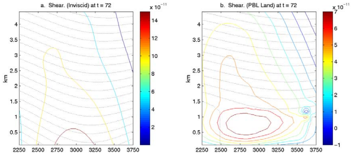
Figure 11. F_{sh} at t = 72 h: (a) inviscid simulation; (b) PBL land simulation.
