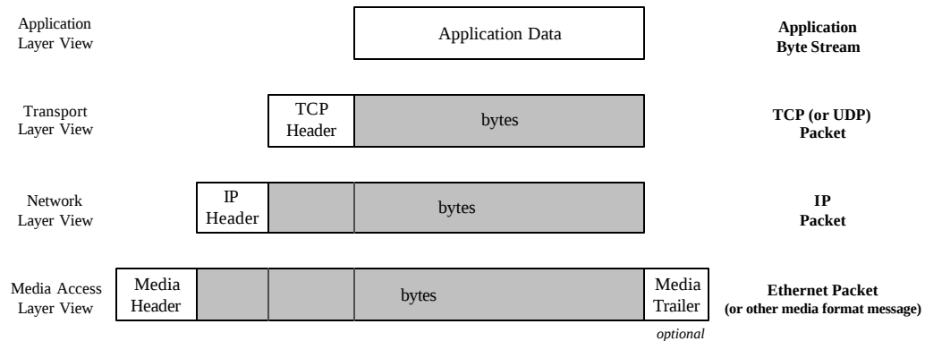
Figure 2-3: Wrapping Lower Level Headers around Data
