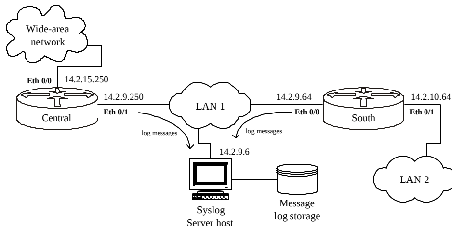
Figure 4-7: A Small Syslog Configuration
