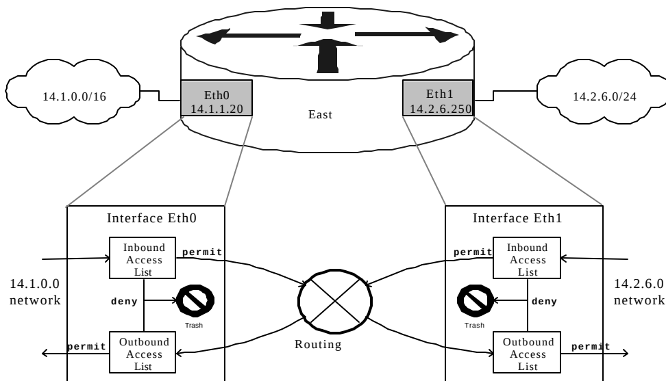
Figure 4-2: Conceptual Model for Access Lists on Interfaces
