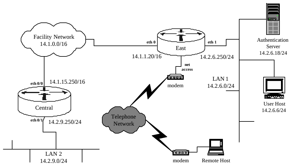
Figure 4-10: Router East in the Network
