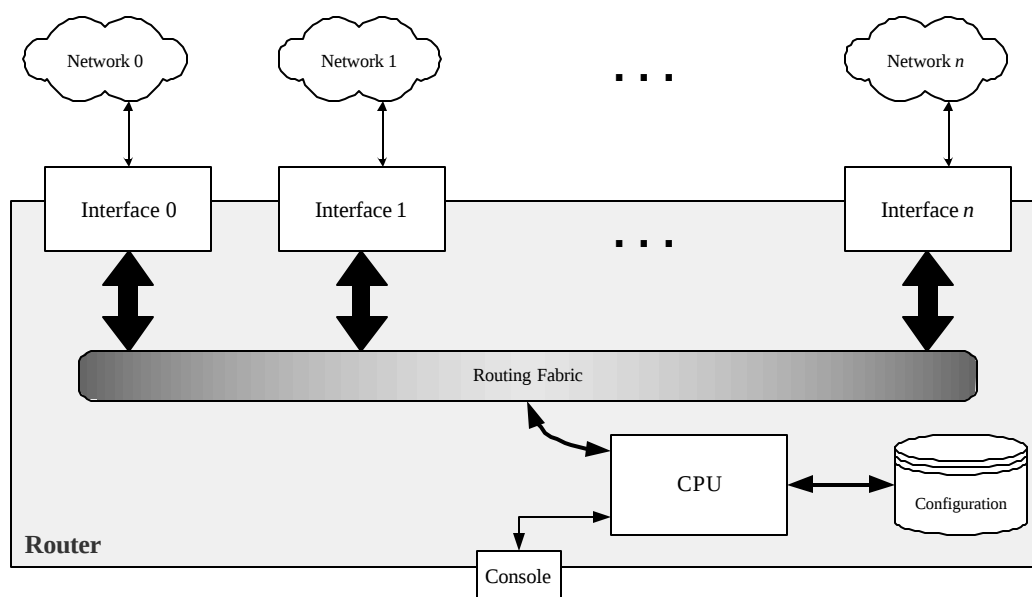
Figure 2-4: A Notional Router's Hardware
