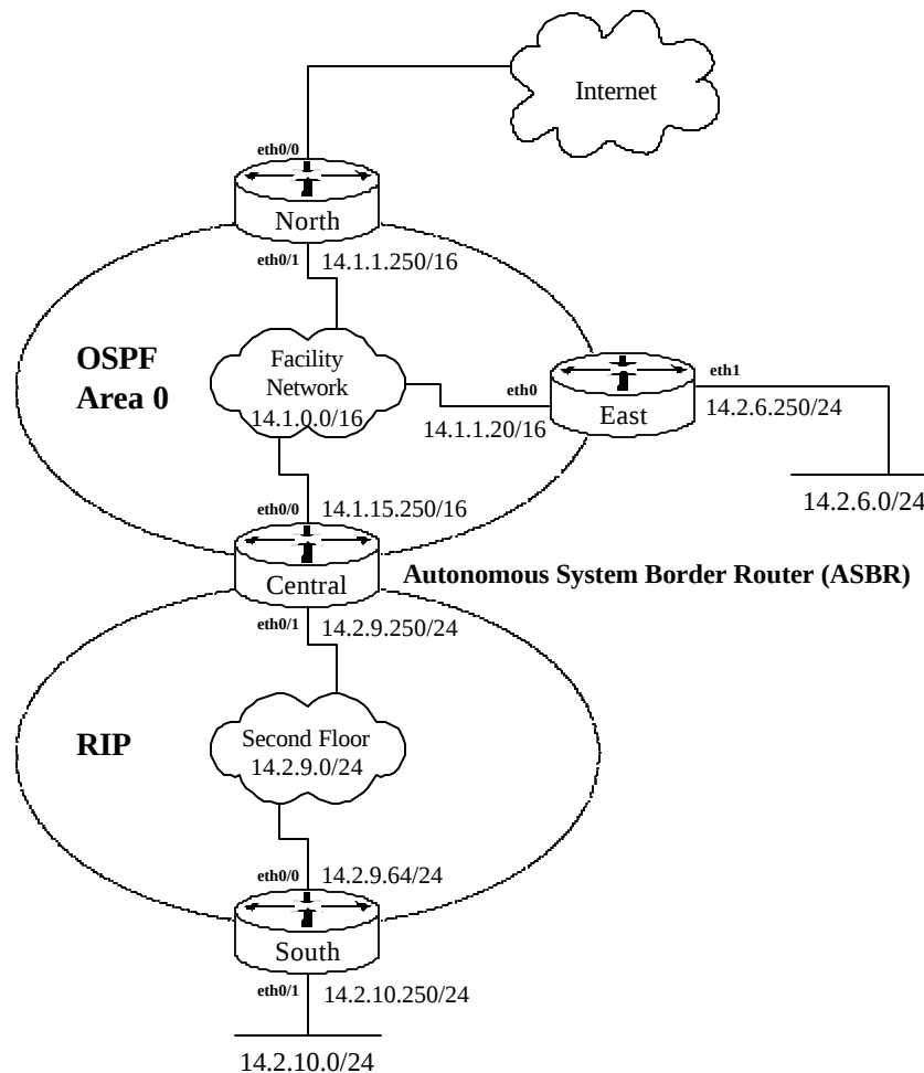
Figure 4-3: A Simple OSPF Routing Architecture
