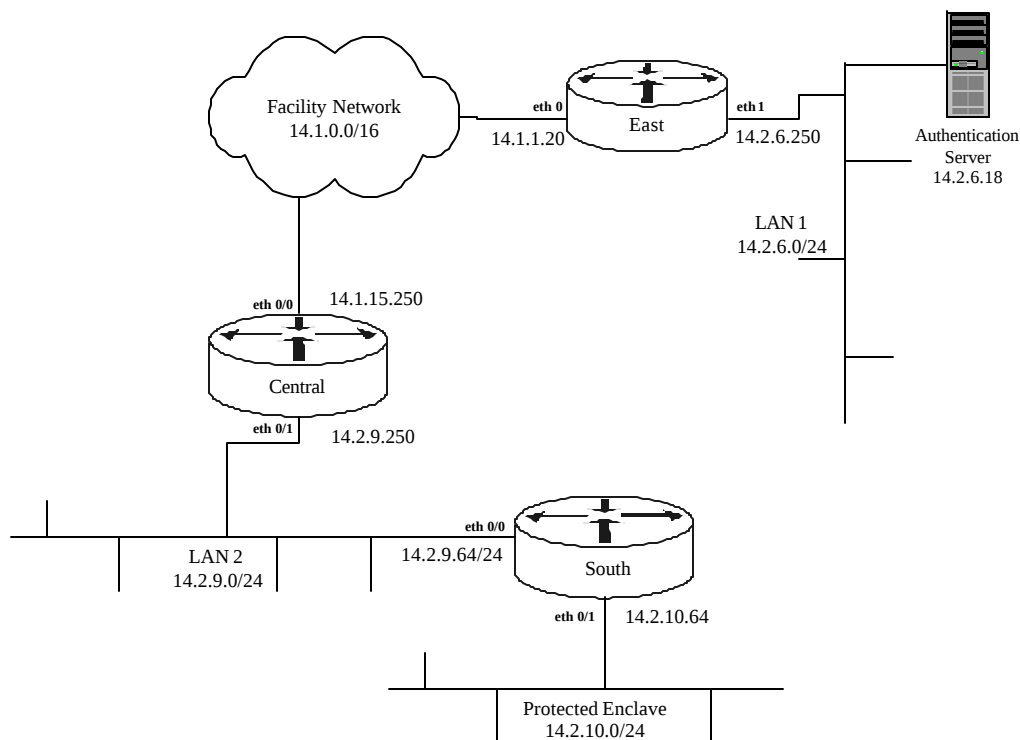
Figure 4-9: Routers and their Authentication Server
