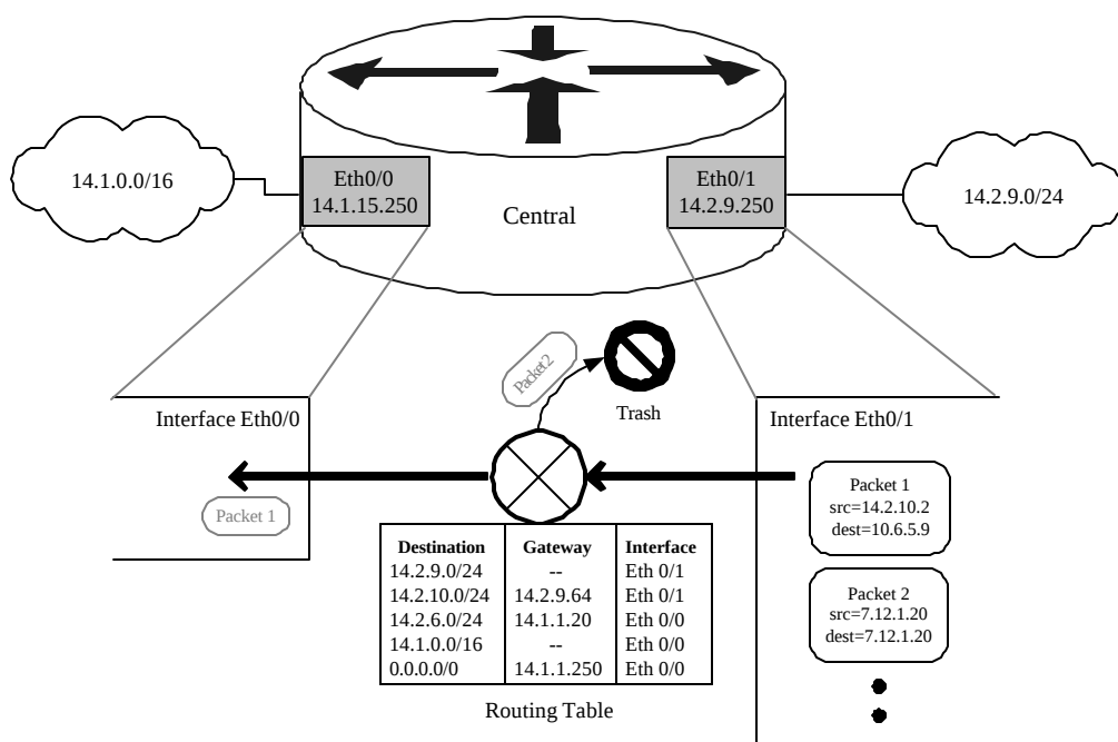
Figure 4-5: IP Unicast RPF Verification
