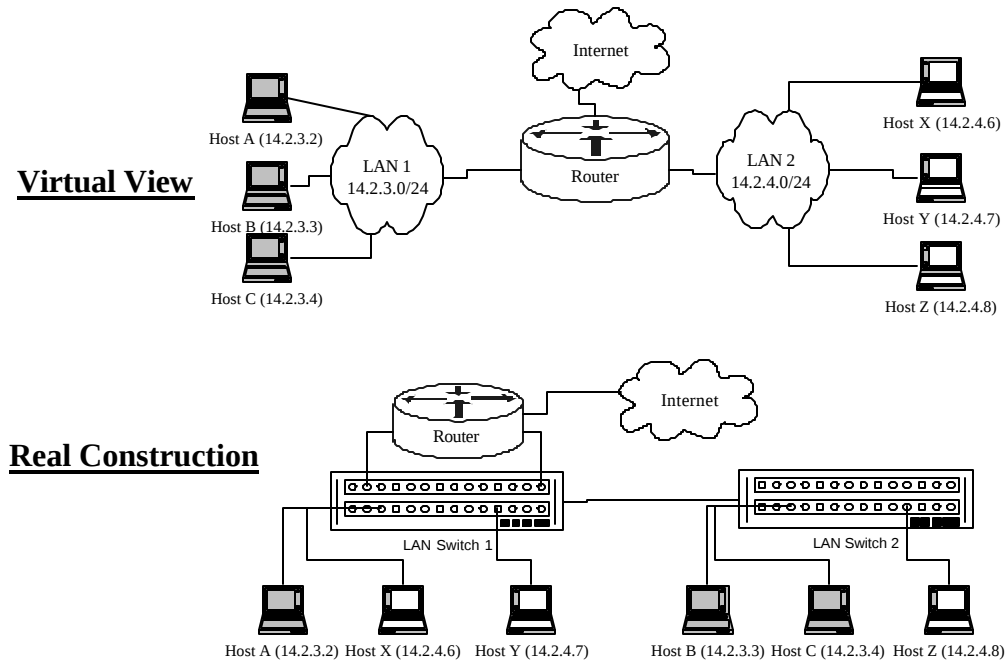
Figure 7-1: Virtual LAN Switching
