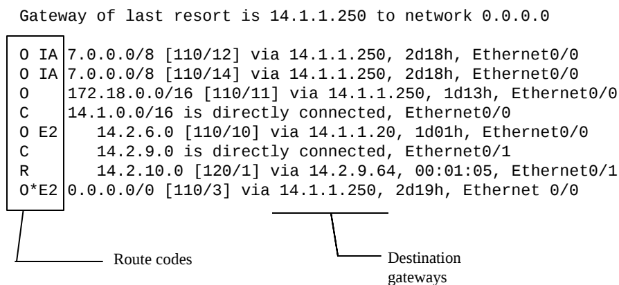
Figure 4-8: Interpreting Route Table Output
