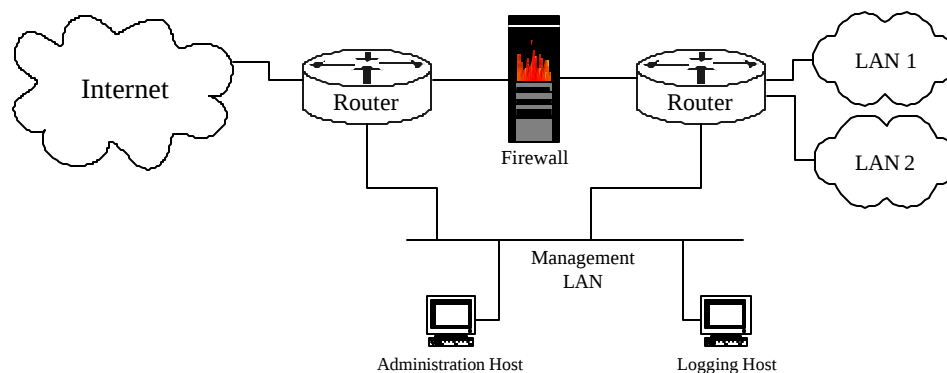
Figure 3-3: Using a Management LAN for Administration
