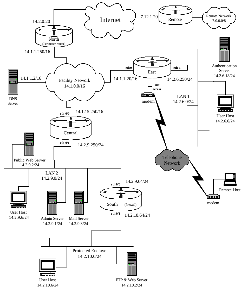
Figure 4-1: Network Diagram for Examples
