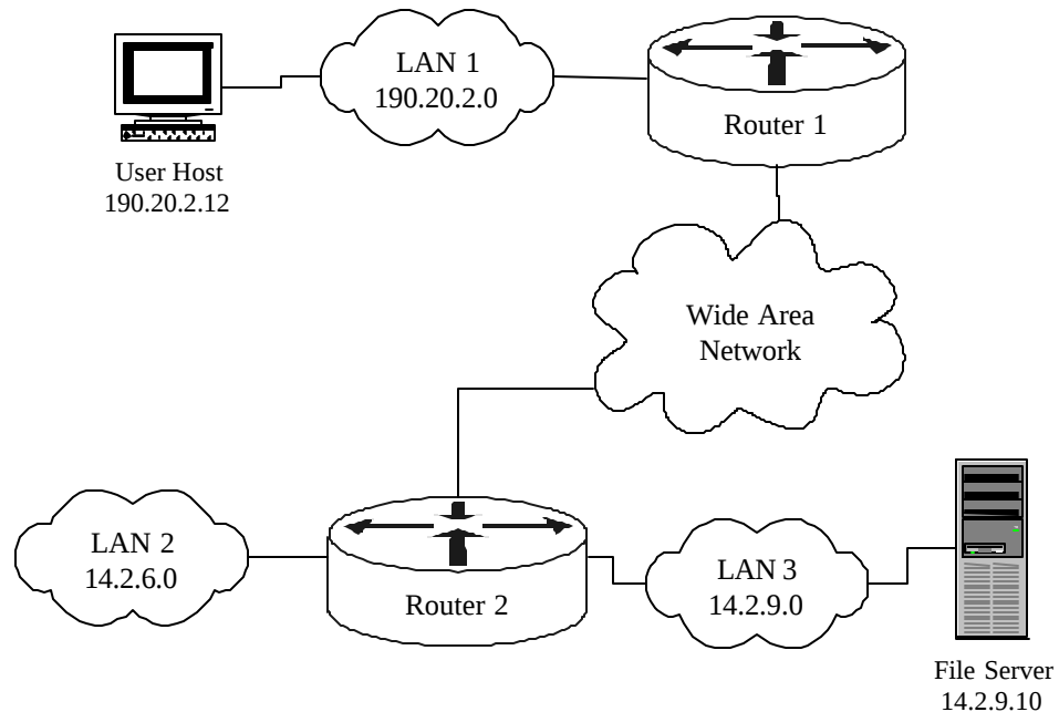
Figure 1-1 – A Simple Network with Two Routers
