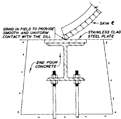
TAINTER VALVE BOTTOM SEAL
