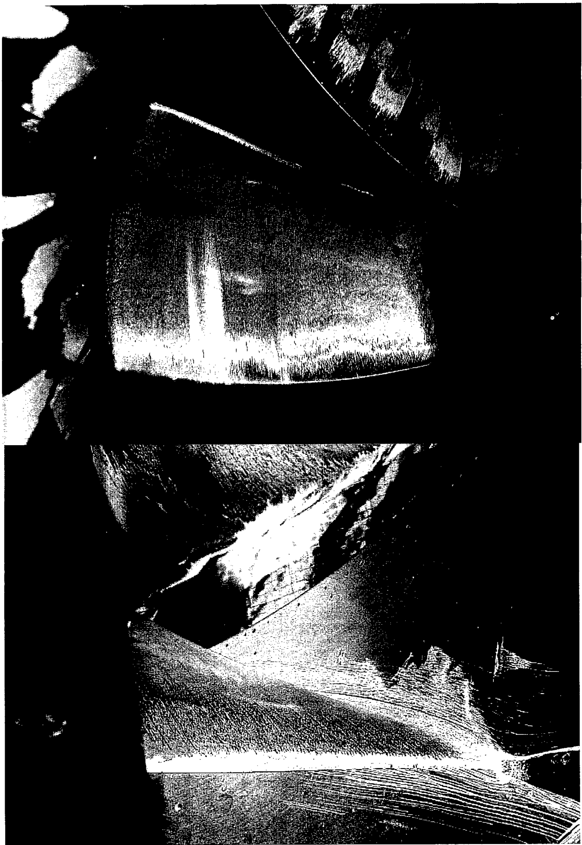
Figure C-4. Paint Flow on the Suction Side of the Rotor Blade, 0 degrees pitch
