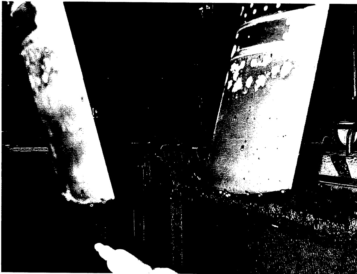
Figure 6. Photographs of the Strut Fairing End Caps
