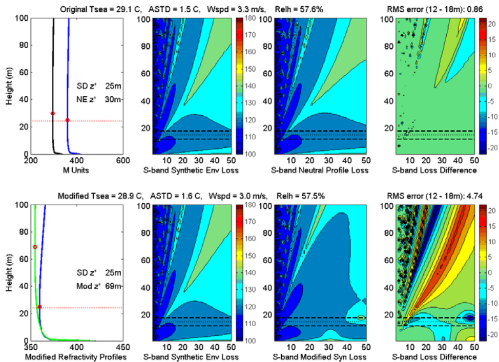
Figure 5. Stability Dependence of the Traditional Method with Measurement Errors
