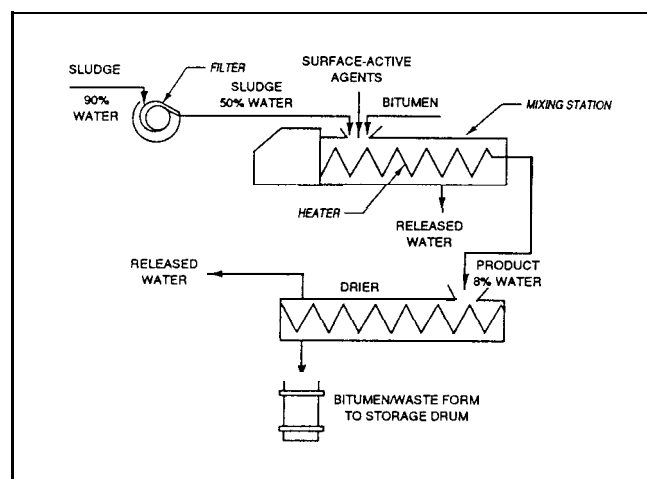
Figure 8-18. Two-step extrusion process (Source: IAEA 1983)
