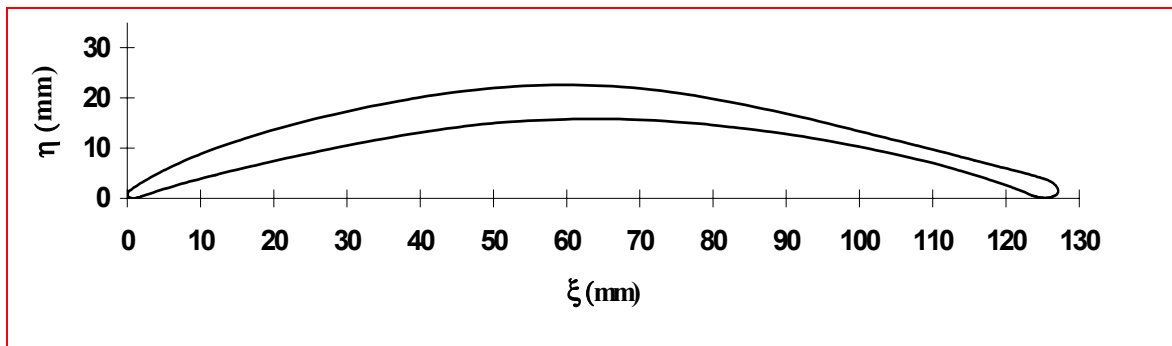
Figure 3. Blade Profile
