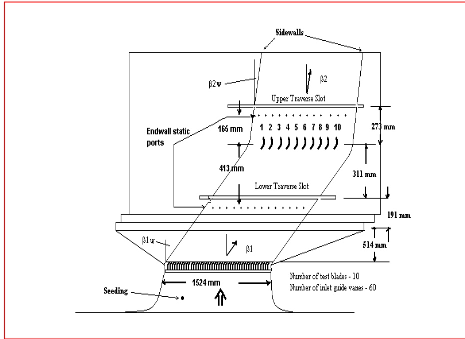
Figure 2. Test Section Schematic
