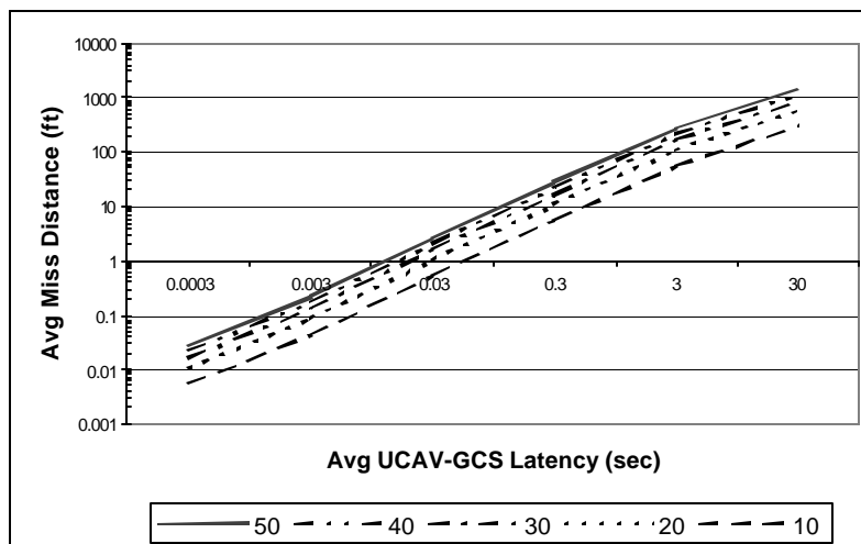
Figure 15. Maneuvering Target with Constant Velocity
