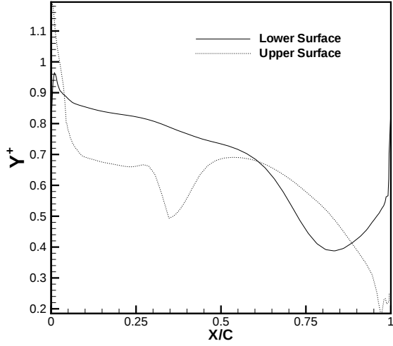
FIG. 3.3. Computed y^+ on wing surface at span break section on baseline grid for Mach=0.75, C_L = 0.6 , Re = 3 million
