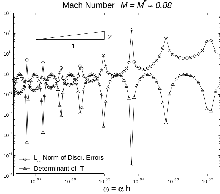
FIG. A.1. L_\infty norms of discretization errors (circles) and the history of the determinant of \mathbf{T} (triangles) for the basic discrete scheme with the overspecified boundary conditions.
