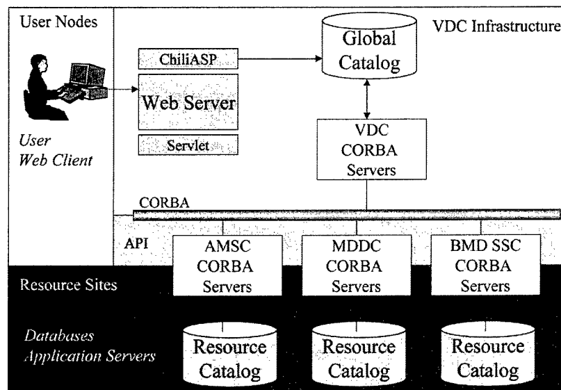
FIGURE 14 VDC high-level architecture.
