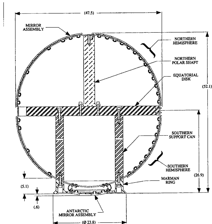
FIGURE 5 Starshine structural assembly (cm).
