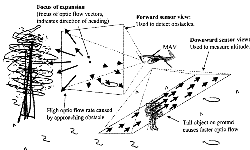
FIGURE 3 Use of optic flow for small-scale navigation.
