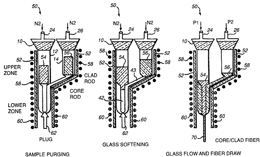
FIGURE 6 Double crucible technique for making chalcogenide glass fibers.
