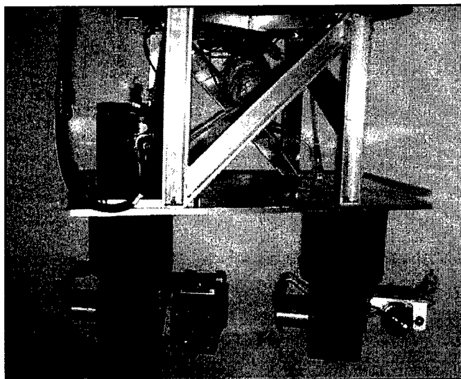
FIGURE 8 Optical bench assembly. RLG is at top left. Imaging camera is on left gimbal; laser communication aperture is on right gimbal. Large lens on right gimbal is cobe-sighted camera for fine laser steering.
