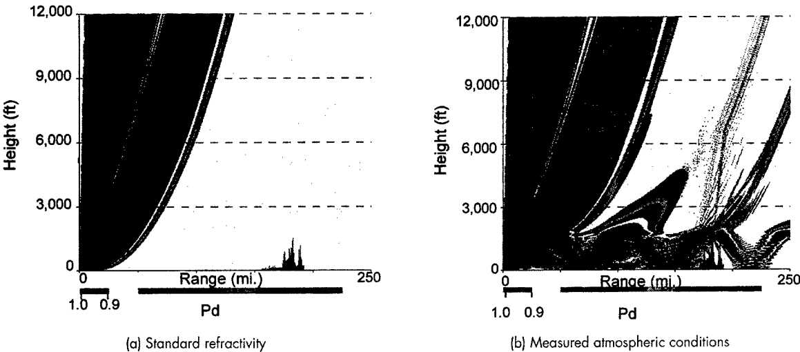
FIGURE 3 Predicted vertical plane coverage.
