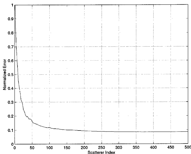
FIGURE 9 Normalized mean-squared error.
