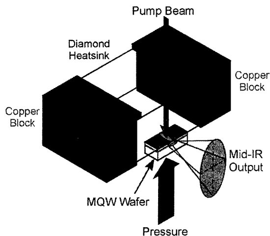
FIGURE 10 NRL diamond pressure bonding (DPB) heat sink.
