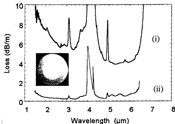
FIGURE 7 Optical loss of fibers made using (i) old technology and (ii) new technology developed at NRL. Insert shows a fiber cross-section.
