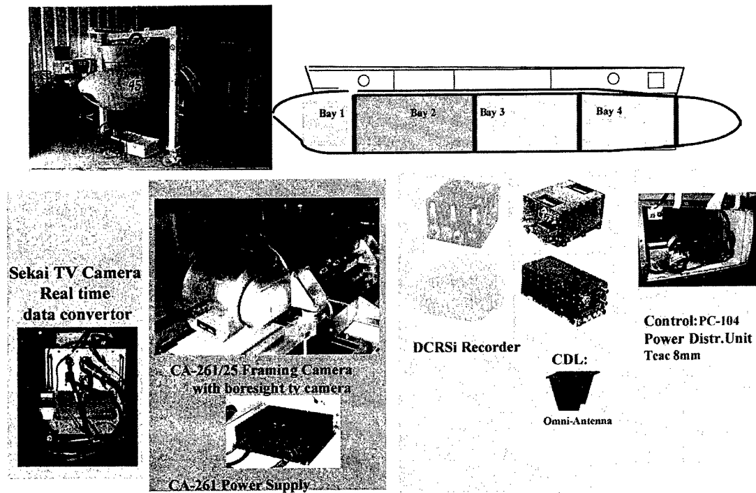
FIGURE 7 Pod payload and locations within the pod.
