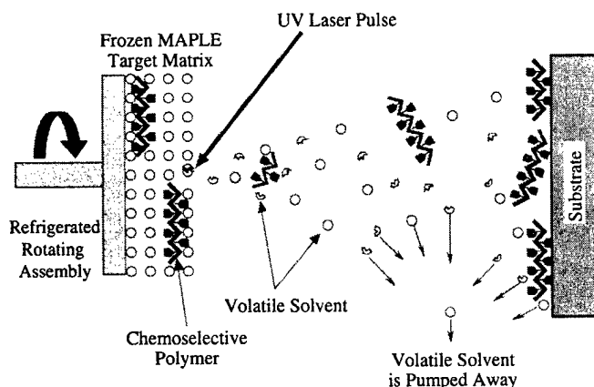
(a) Basic elements of the MAPLE process. The UV laser interacts with the volatile solvent in the frozen matrix releasing the polymer molecules, which form a film over the substrate. The solvent is pumped in the process.
