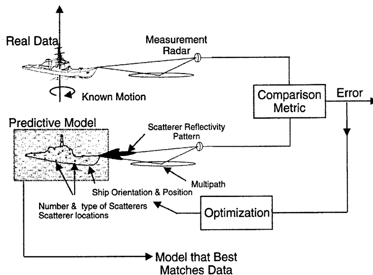
FIGURE 7 Framework for constrained optimization approach.
