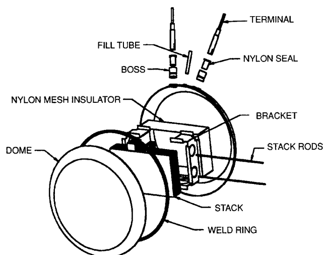
FIGURE 13 90 Ah DPV \text{NiH}_2 battery cell design.
