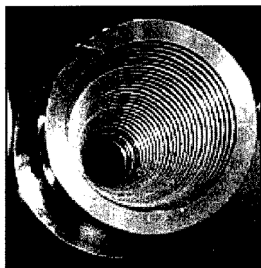
FIGURE 5 Conical corrugated feed horn.
