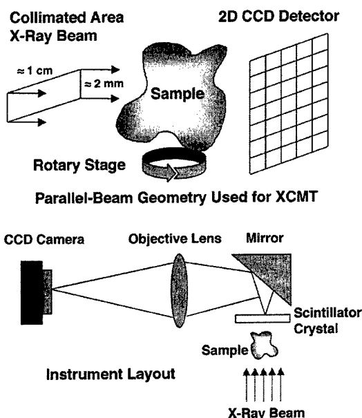
FIGURE 1 Schematic of the data collection geometry and instrument layout used for XCMT.
