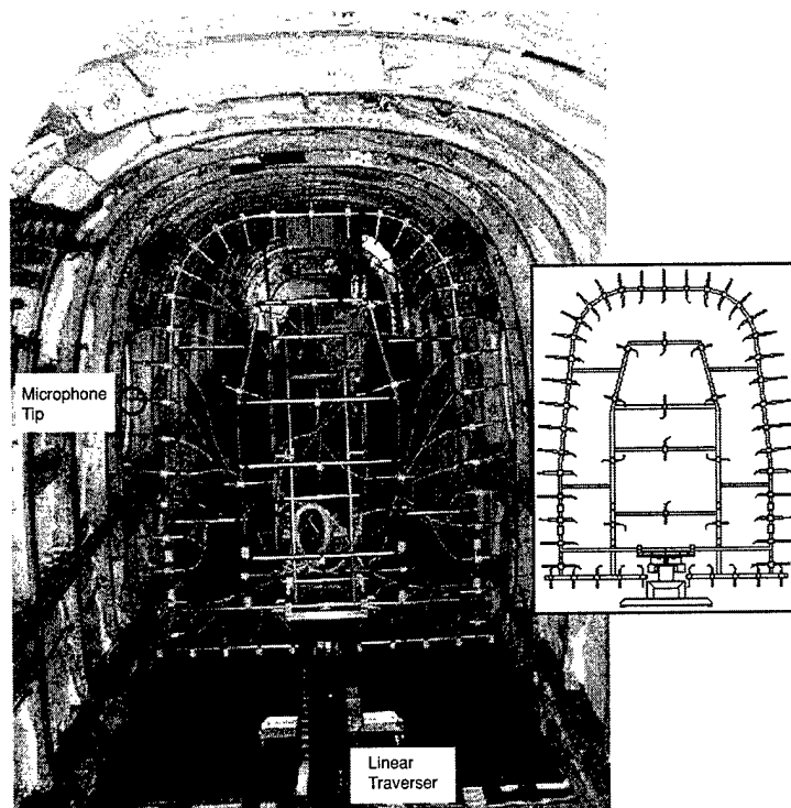
FIGURE 2 Microphone boom consisting of 43 microphones on the outer ring and 12 spaced evenly in the internal region, all located in the same vertical plane. The boom was moved on a linear traverser to 32 different axial locations during the experiment (5.12 m total scan length). Time domain data were sampled at 5 kHz and were processed at the BPF and its harmonics. The total acquisition time for the data scan was 66 minutes.
