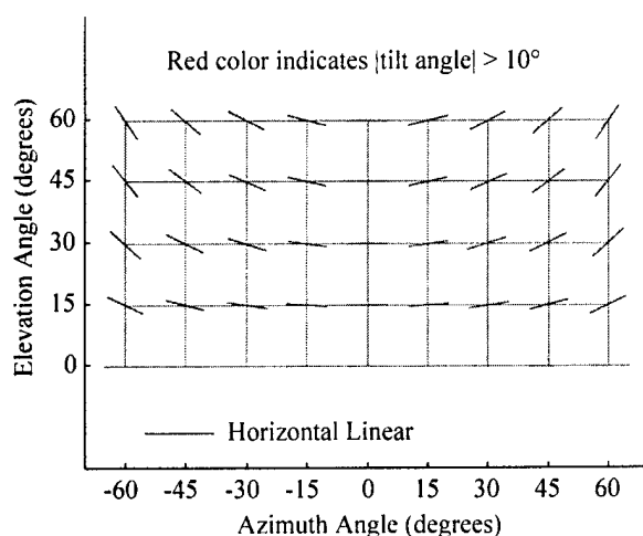
FIGURE 3 Polarization states for horizontally polarized dipole element.
