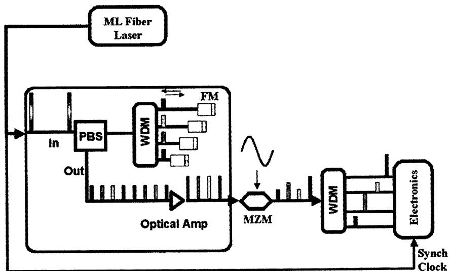
FIGURE 1 Photonic analog-digital converter architecture.
