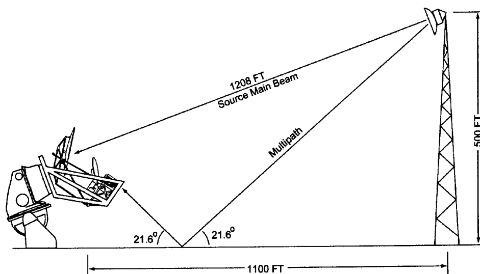
FIGURE 6 Range geometry used to calibrate the system.
