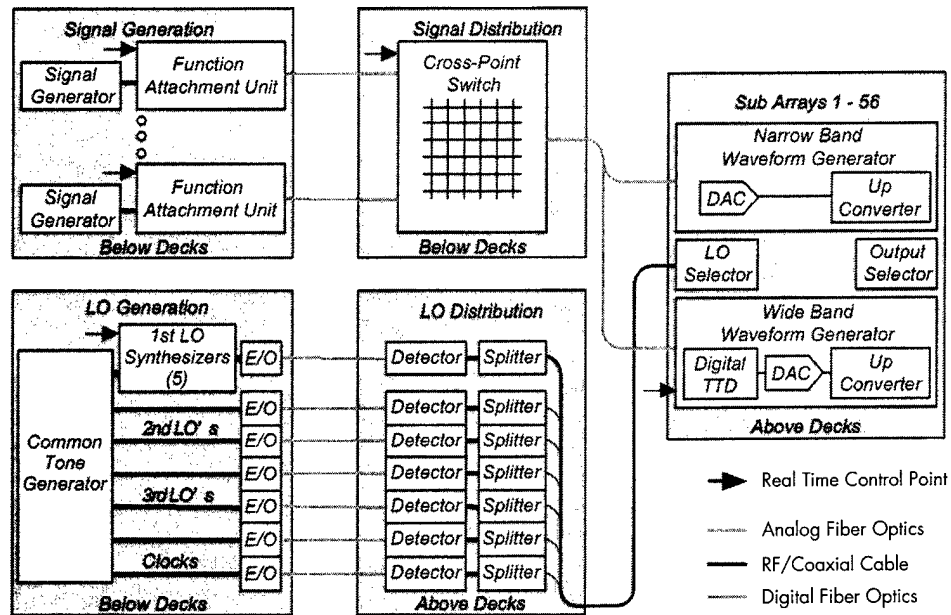
FIGURE 4 Transmit Signal and Local Oscillator Distribution.
