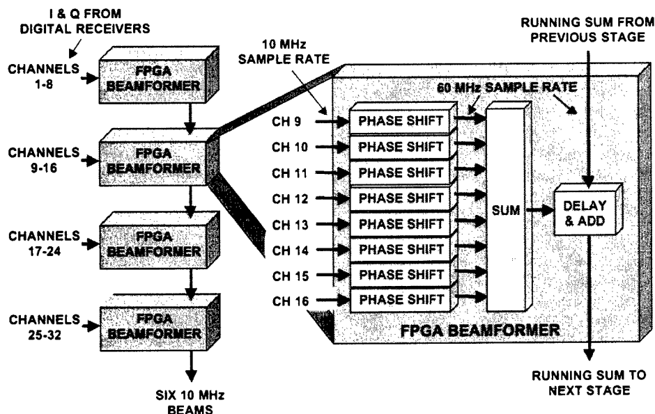
FIGURE 8 32-Channel digital beamformer implementation using FPGA technology.
