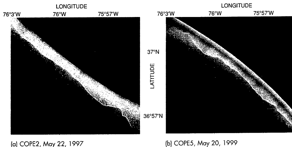
FIGURE 8 NRL RAR images of the plume front collected during the late flood portion of the tidal cycle.
