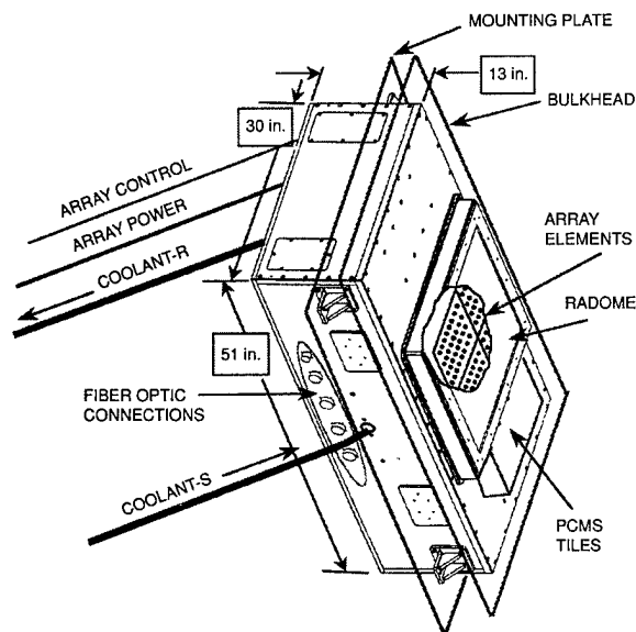
FIGURE 1 EA transmitter array.
