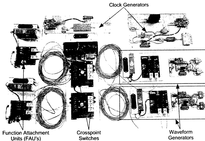
FIGURE 5 Distributed waveform generator breadboard hardware.
