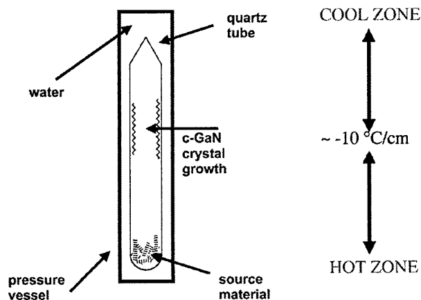
FIGURE 7 Diagram of apparatus used.
