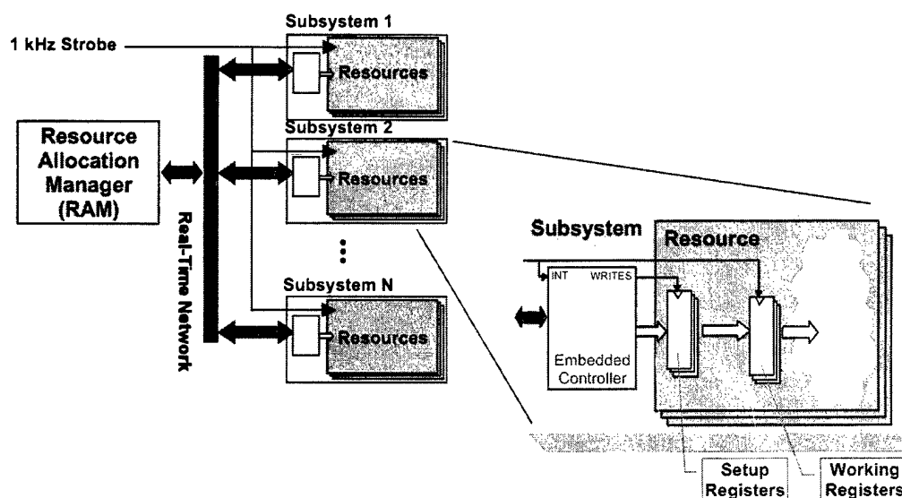
FIGURE 9 Distributed real-time control synchronization strategy.
