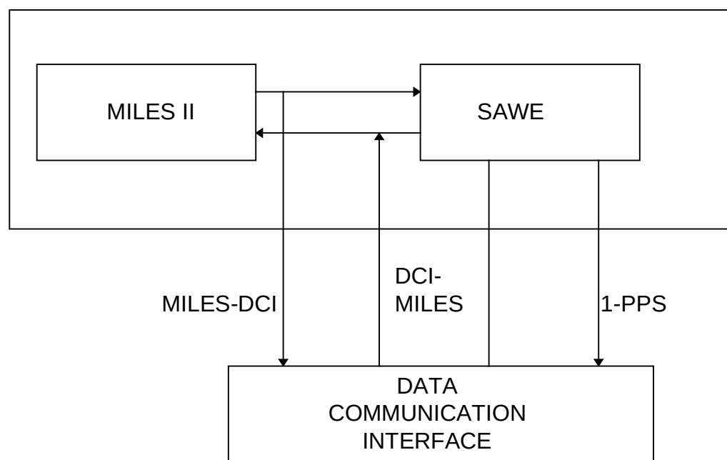
Figure 4.2.1-1. NTC-IS DCI/DD Interface Diagram for SAWE/MILES II
