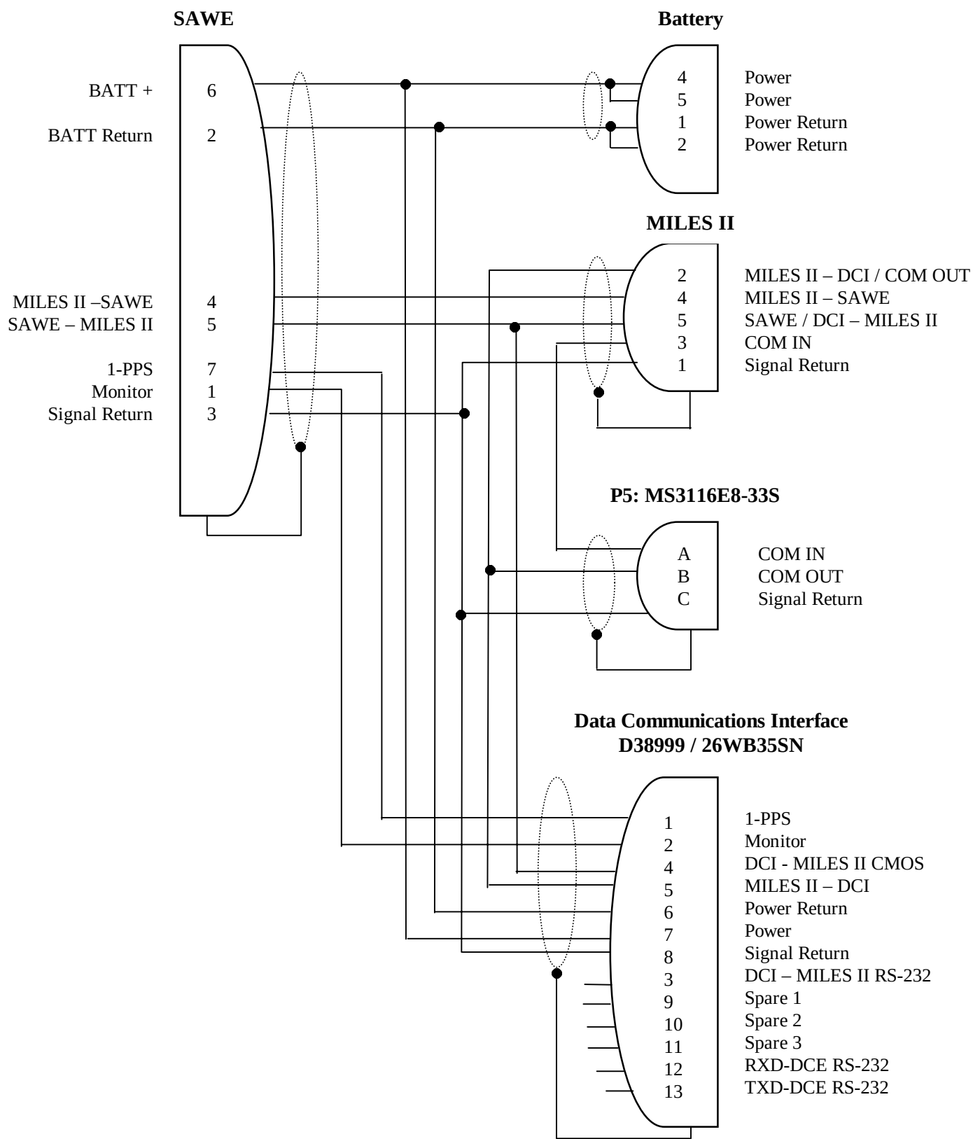
Figure 3.2.2-1. CMTC-IS DCI/PDD Interconnection Diagram
