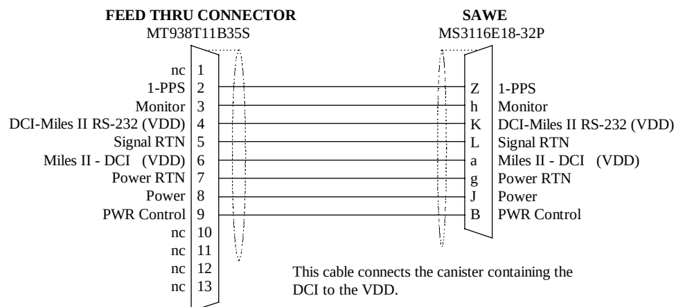
Figure 4.2.2-2 NTC RDMS Upgrade DCI/VDD Interconnection Diagram
