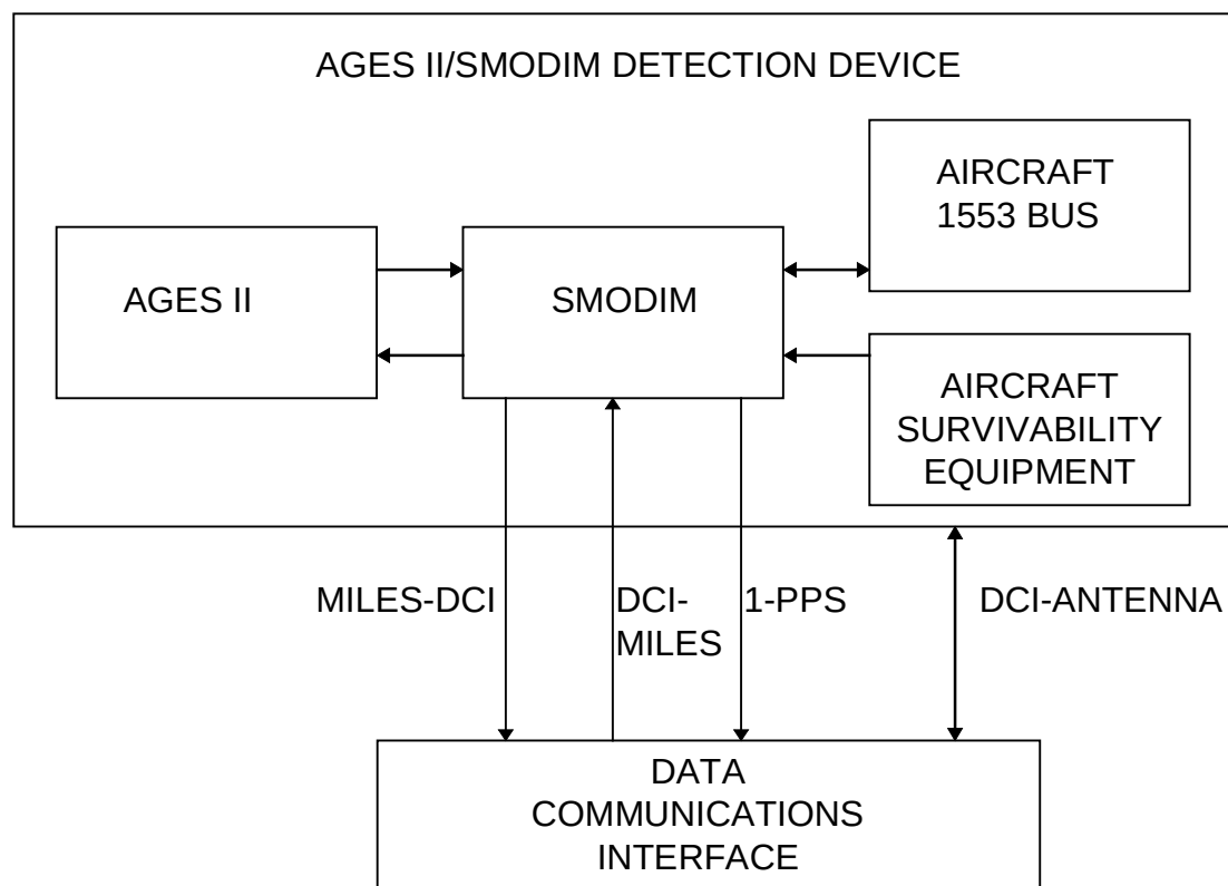
Figure 3.2.1-2. CMTIC-IS DCI/DD Interface Diagram for AGES II/SMODIM
