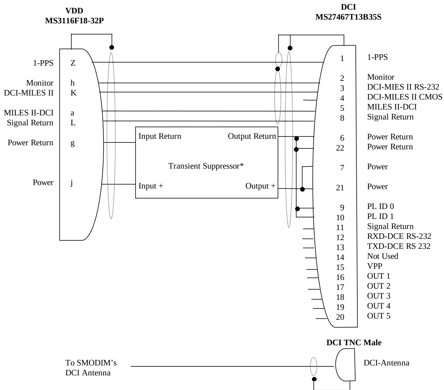
Interface Cable with Integral Transient Suppressor (*For compliance with CS06 requirement of PMT-91-S008, paragraph 3.2.6.11.1.3)
