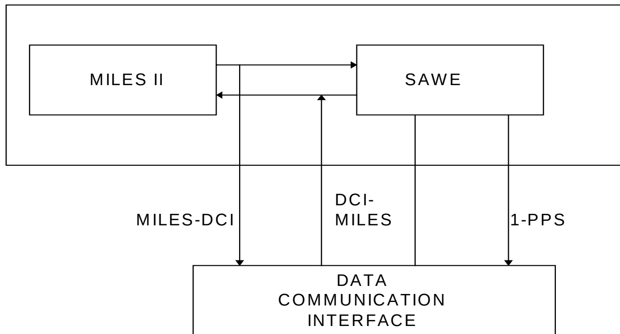
Figure 5.2.1-1. JRTC-IS DCI/DD Interface Diagram for SAWE/MILES II
