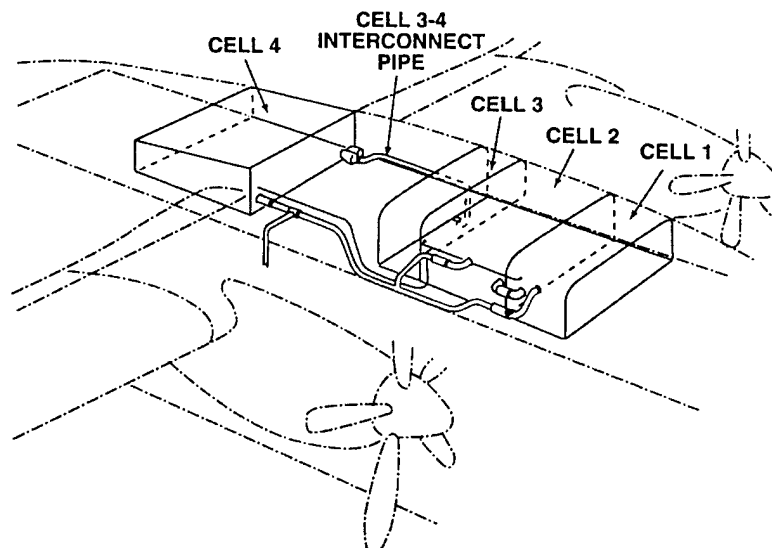
FIGURE 3-12. SHORTS 3-30 FUEL SYSTEM
