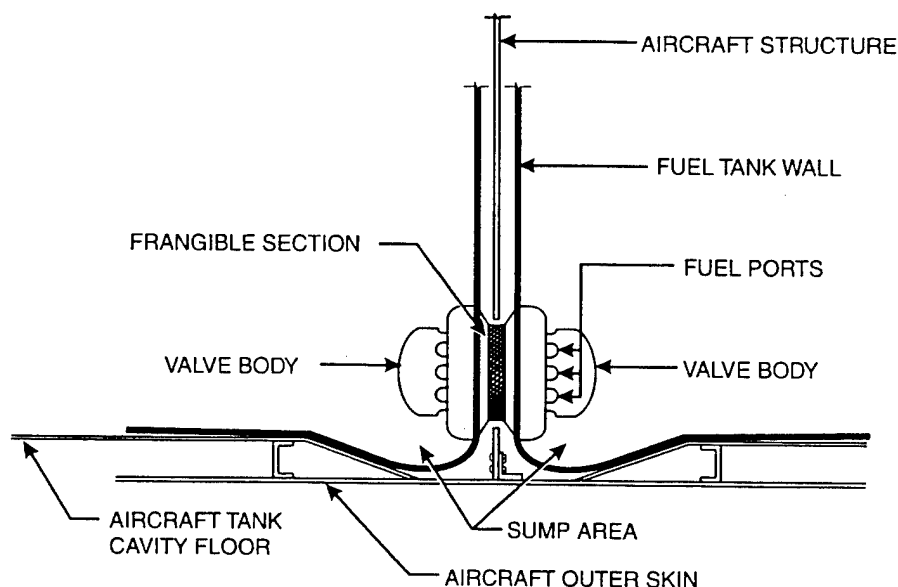
FIGURE 6-11. SELF-SEALING BREAKAWAY VALVE USED AS A TANK-TO-TANK INTERCONNECT
