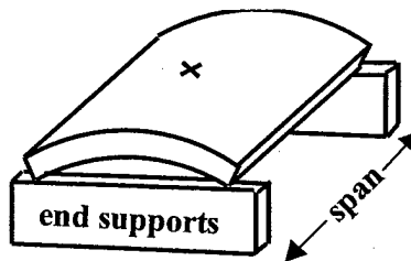
FIGURE 3. POSITION OF CURVED SPECIMENS
