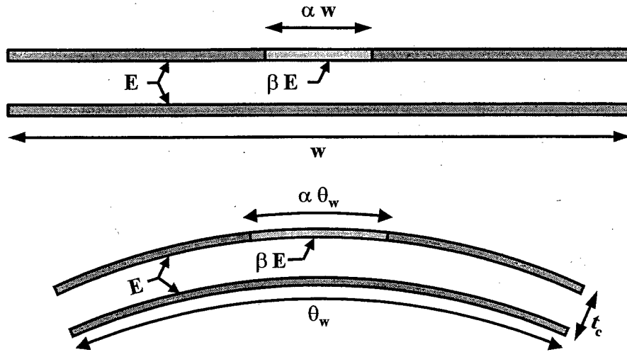
FIGURE 31. SECTION PROPERTY MODELS
