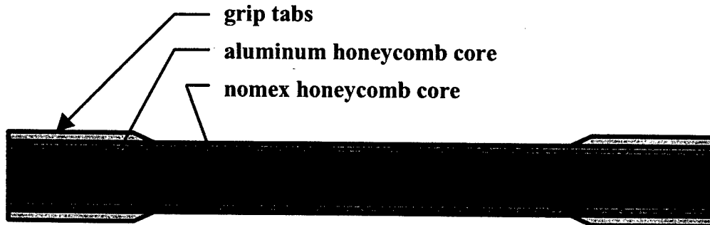
FIGURE 22. GRIPPED SPECIMEN
