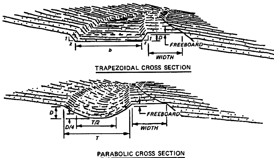
Figure 3-26. General Design Features of Diversions
