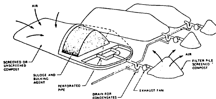
b. Typical aerated static pile composting system.
