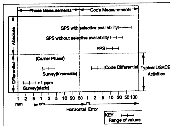
Figure 2-1. GPS operating modes and accuracies
