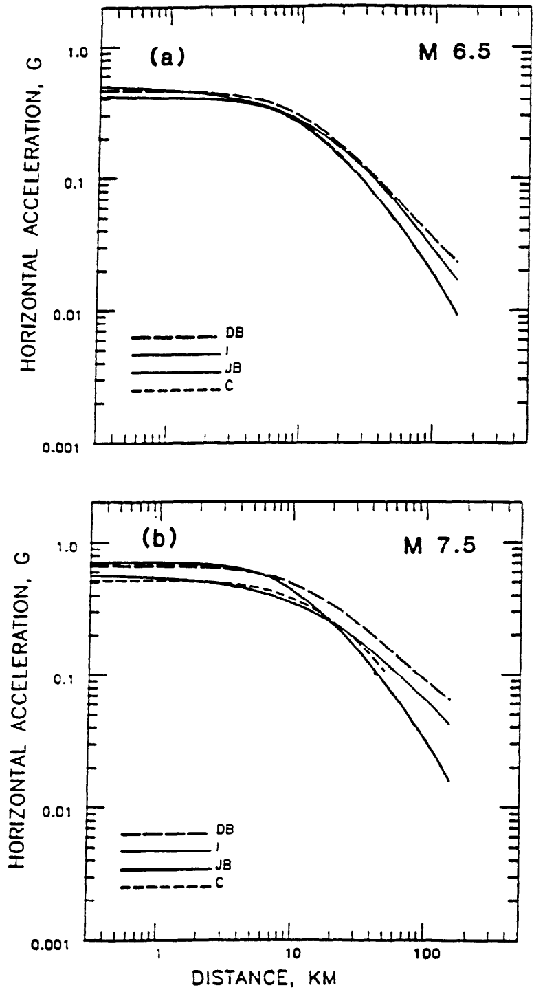
Figure 4. Comparison of different relationship for peak horizontal acceleration at Magnitude 6.5 and 7.5 Reprinted from Joyner and Boore (1988) with permission from American Society of Civil Engineers
