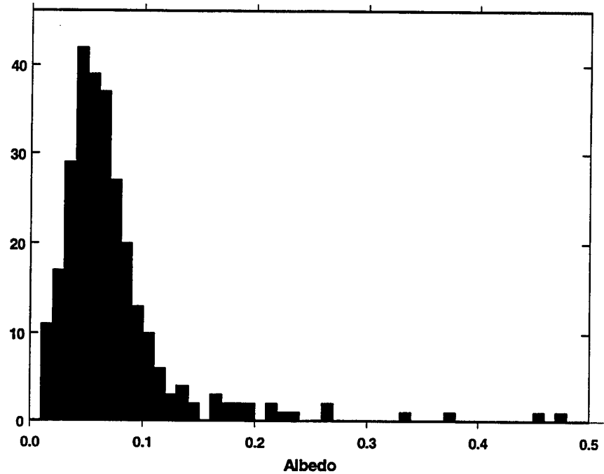
Figure 11. Albedo histogram for new SIMPS asteroids.
