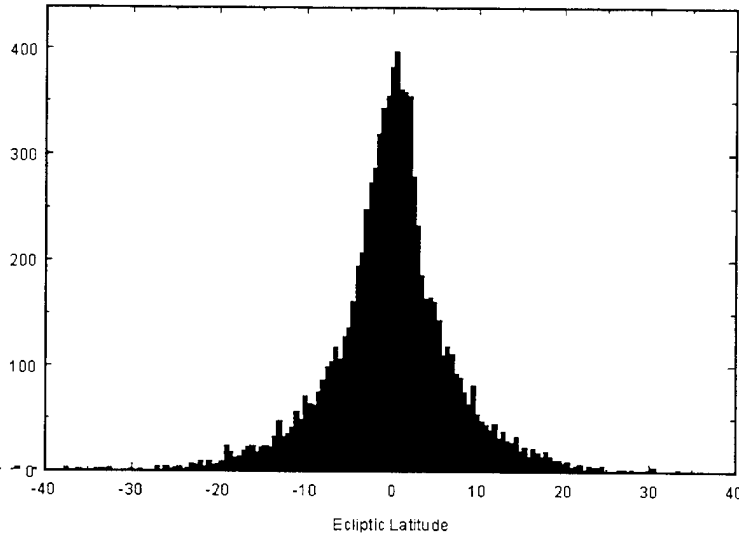
Fig. 18. Distribution of Numbered Asteroids in Ecliptic Coordinates.
