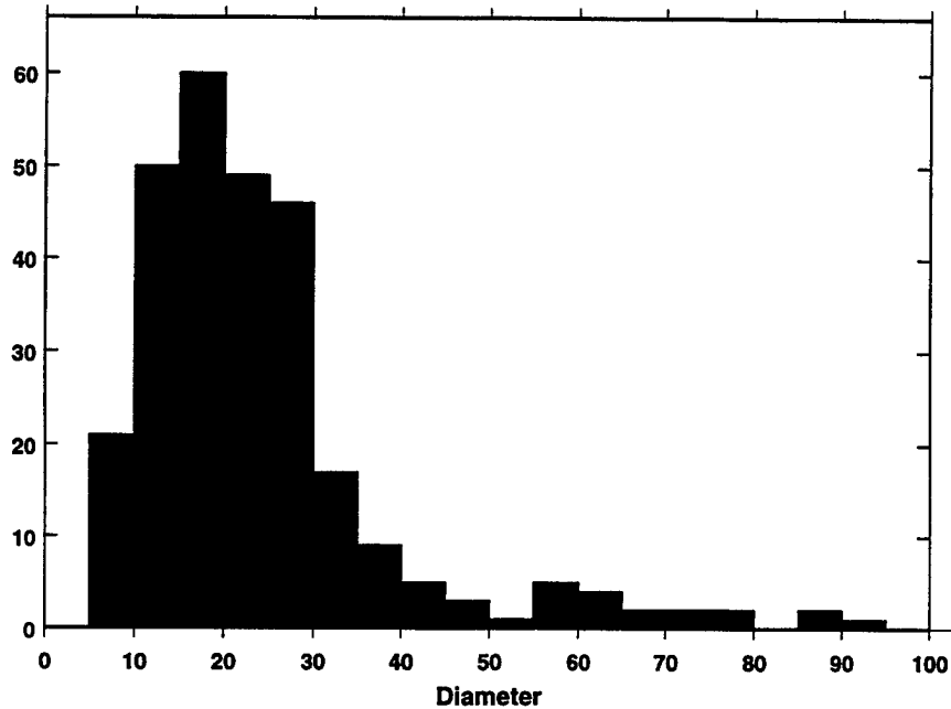
Figure 12. Diameter (km) histogram for new SIMPS asteroids.
