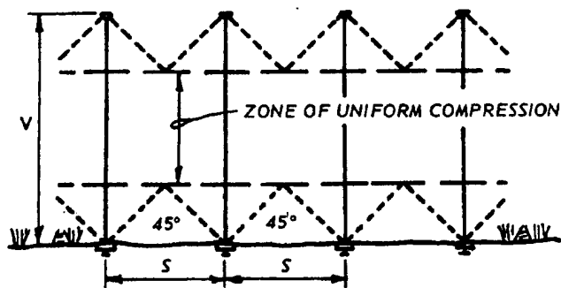
Figure 2-6. Structural member concept.
