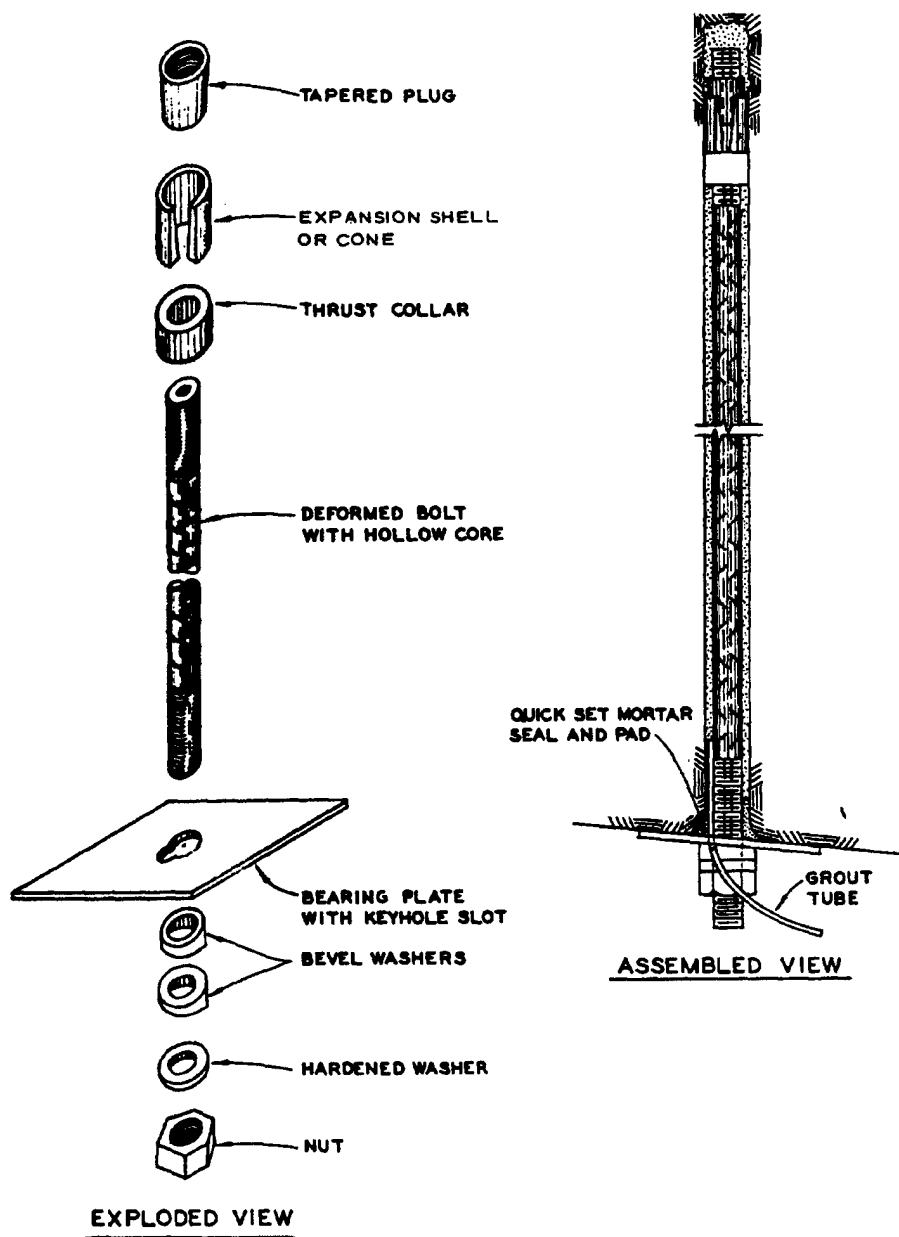
Figure 3-5. Hollow groutable deformed bar rock bolt.
