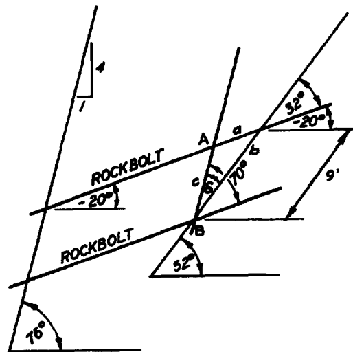
Figure 3-16. Calculation of actual bolt spacing for FS = 1.1.
