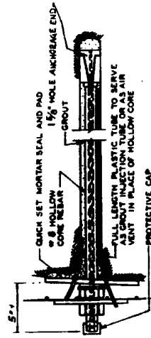
Figure B-2. Rock bolt deformer.
