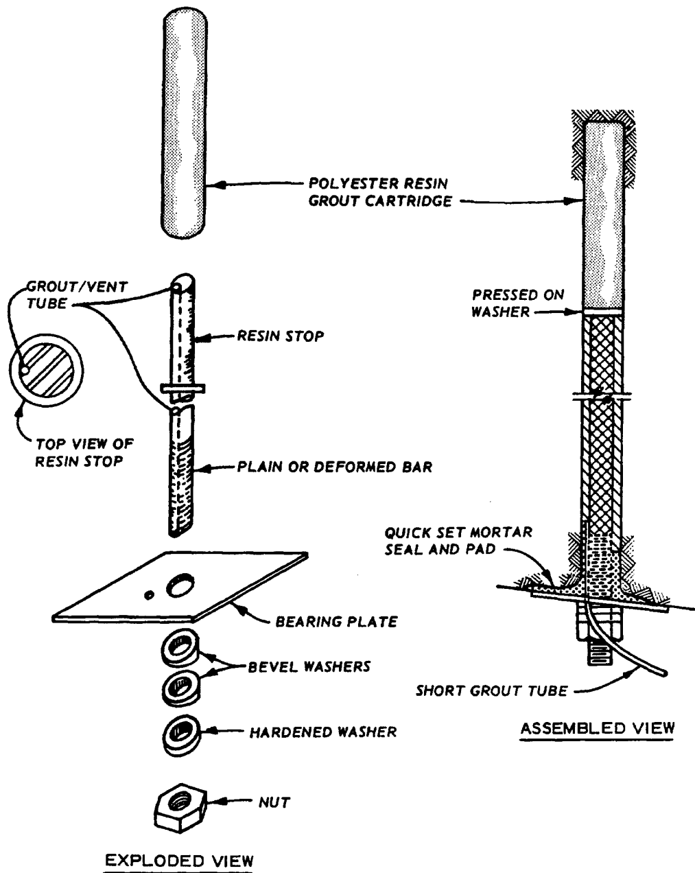
Figure 3-10. Cement groutable rock bolt with resin anchor stop and integral grout tube.
