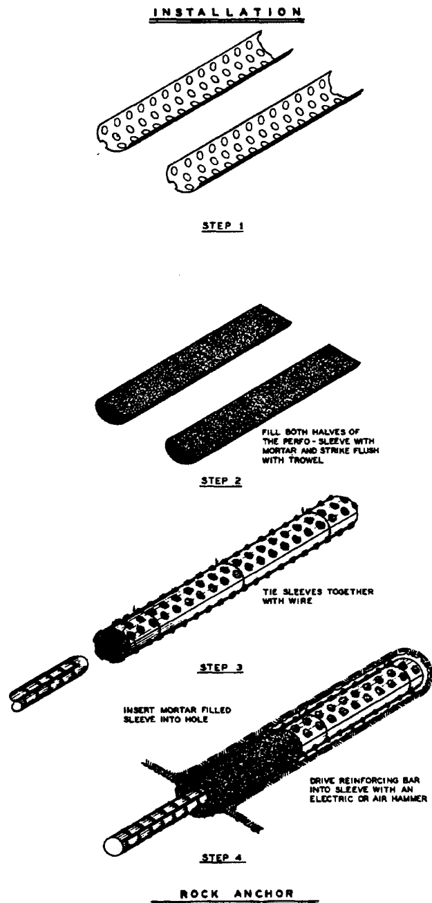
Figure 4-1. Rock anchor, perforated sleeve and mortar type.
