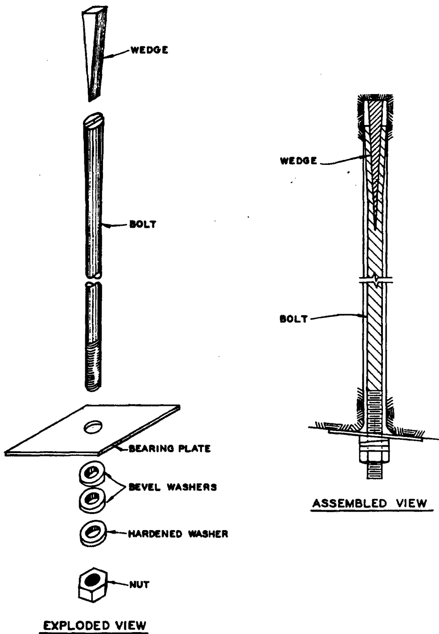
Figure 3-1. Slot and wedge rock bolt.
