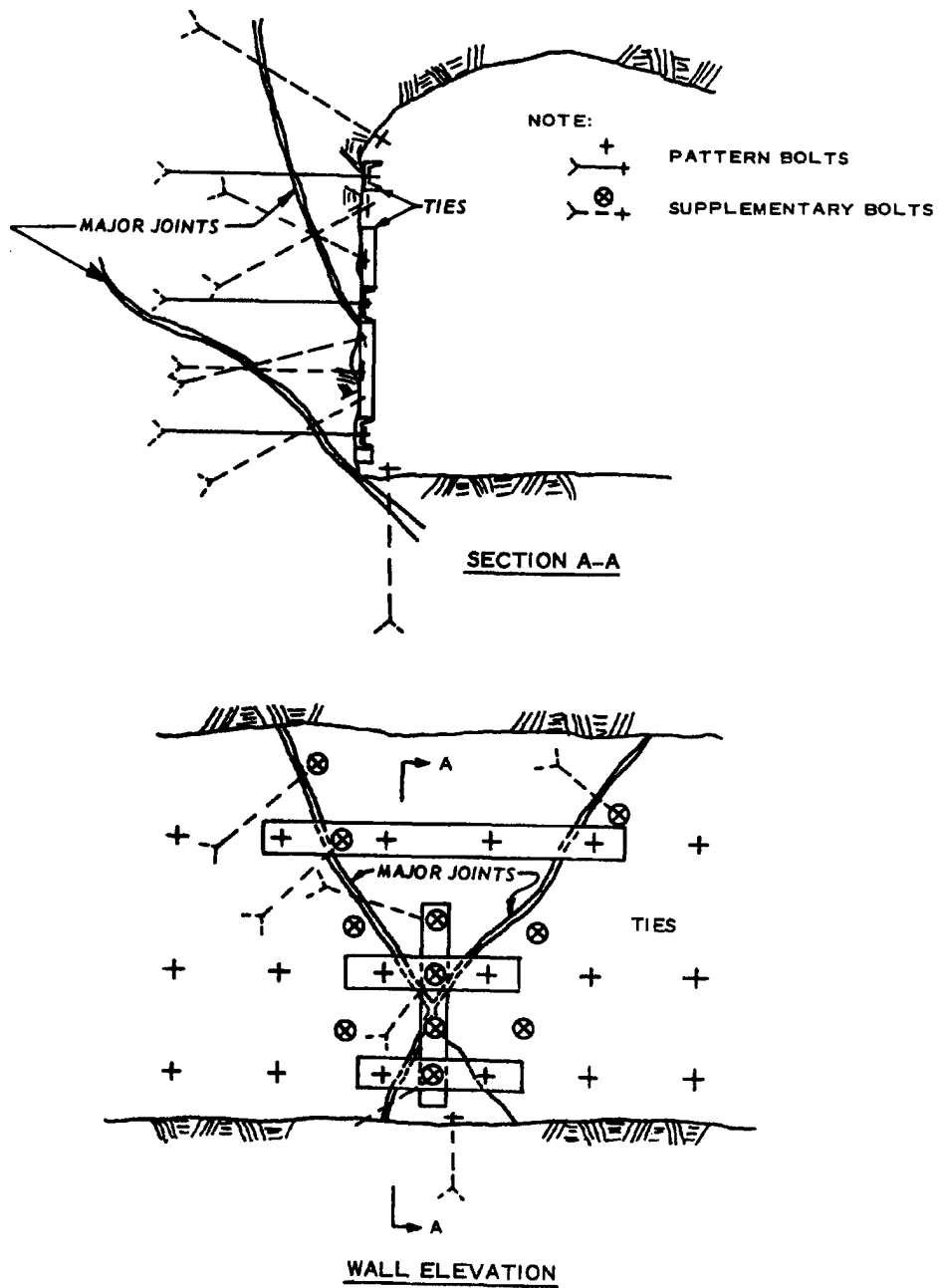
Figure 6-3. Typical use of ties and supplementary bolts.
