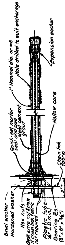
Figure B-1. Grouted rock bolt (with chain link fabric).
