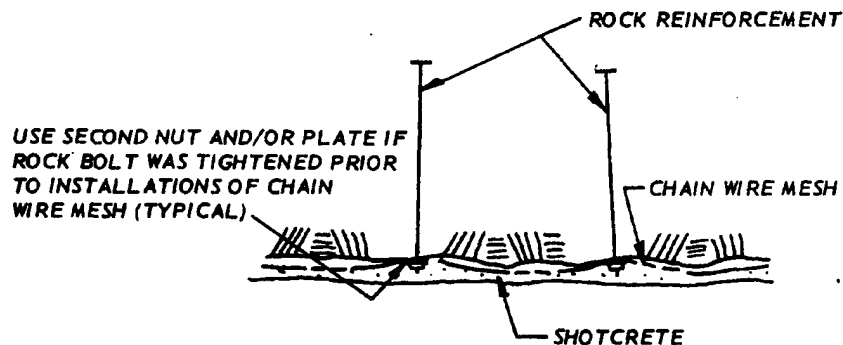
Figure 6-1. General surface treatment-wire mesh and shotcrete.
