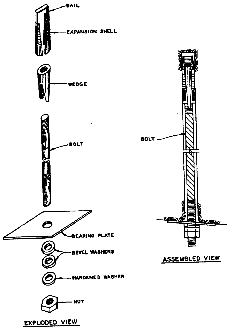
Figure 3-3. Bail expansion anchorage--solid bolt.
