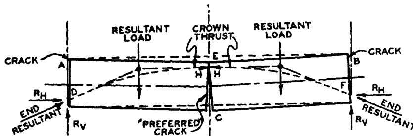
Figure 2-5. Idealized sketch of beam behavior.
