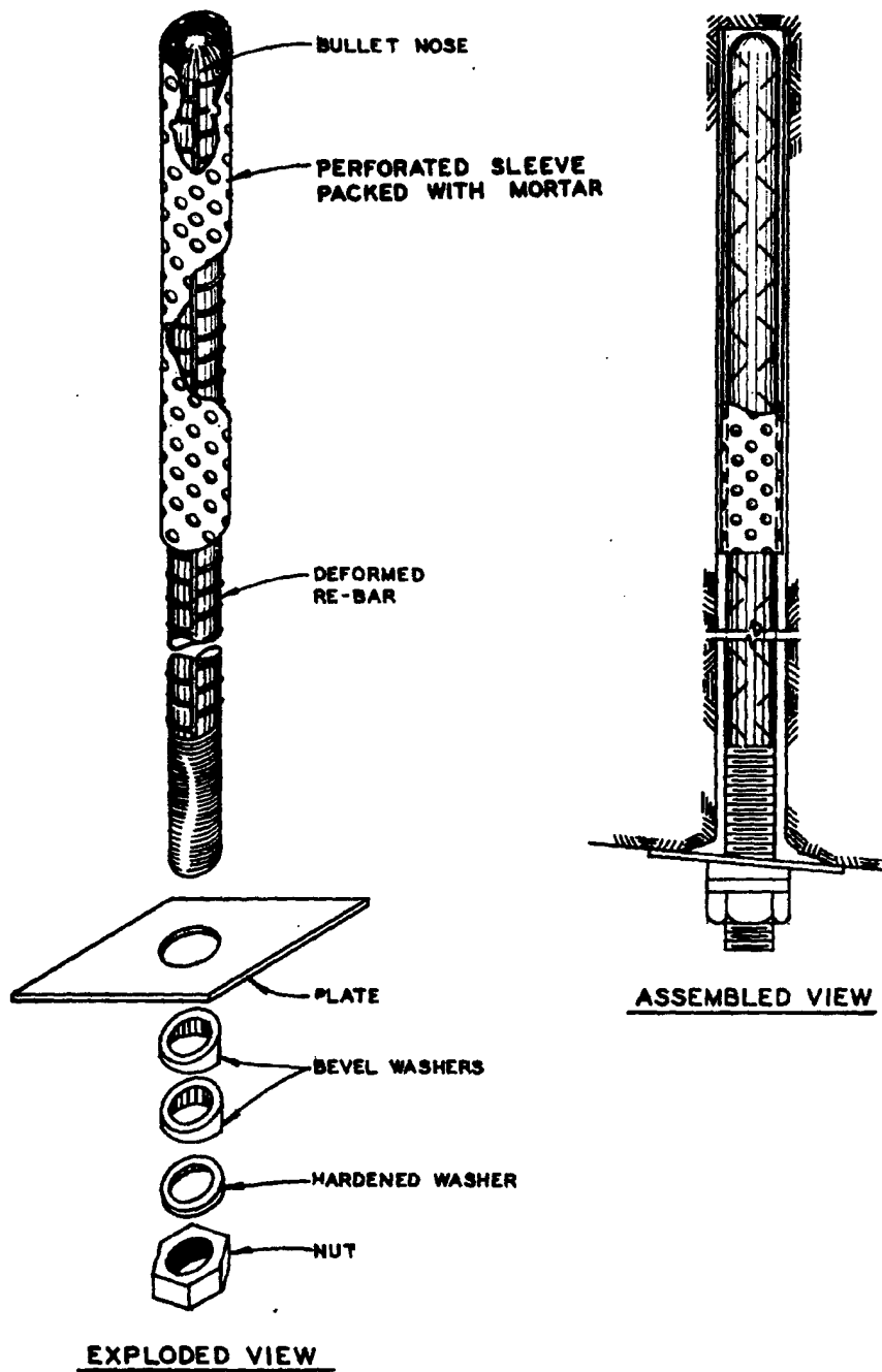
Figure 3-7. Grouted end anchorage, perforated sleeve and mortar type.
