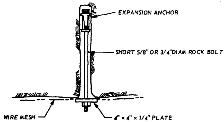
a. SHORT EXPANSION ANCHOR.
