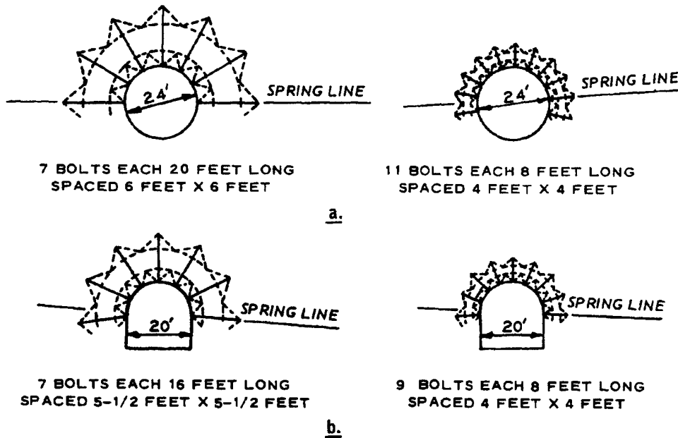
Figure 2.8. Arch concept of rock reinforcement.
