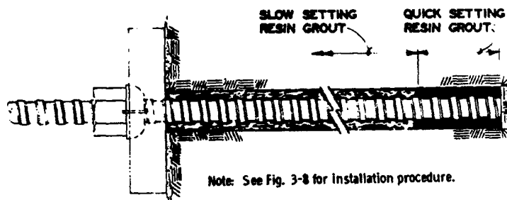
Figure 3-9. "Thread bar" rock bolt with polyester resin grouted anchorage.
