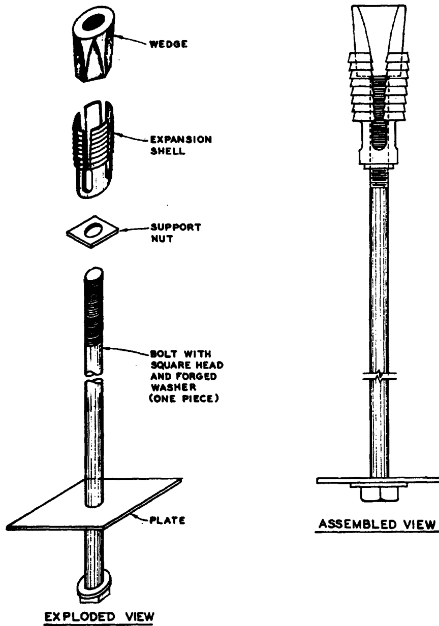
Figure 3-2. Regular expansion anchorage--headed bolt.
