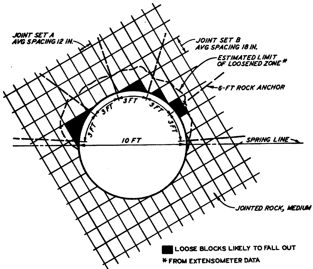
Figure 3-13. Example of underground reinforcement.
