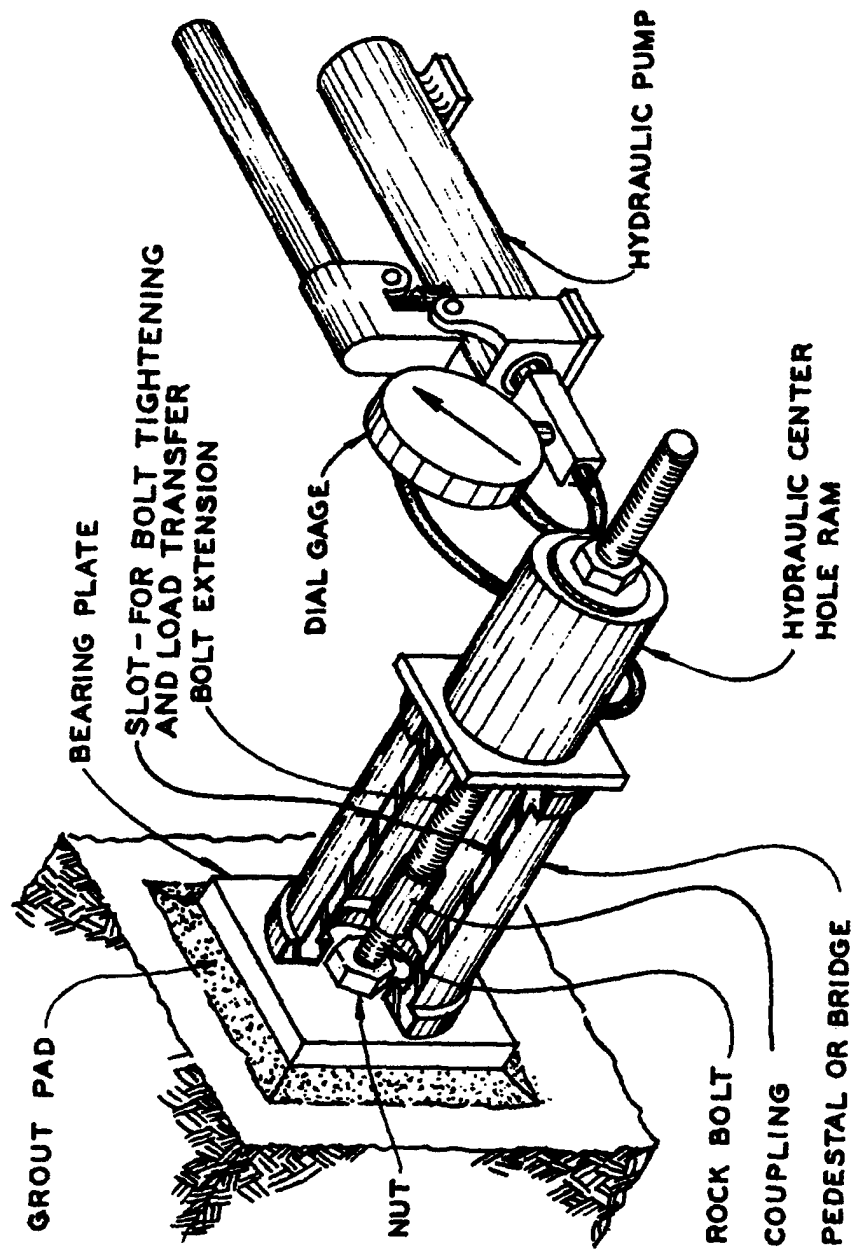
Figure 3-11. Center hole ram for direct tensioning of rock bolts.
