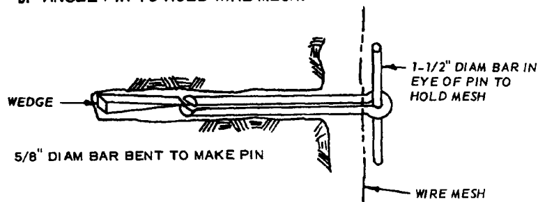
b. ANGLE PIN TO HOLD WIRE MESH.
