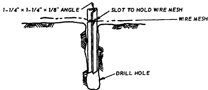
b. ANGLE PIN TO HOLD WIRE MESH.
