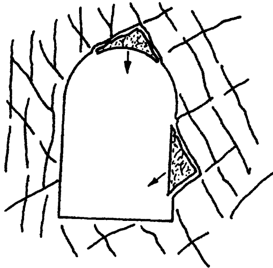
(a) Fallout of blocks isolated from rock mass due to failure along joints.
