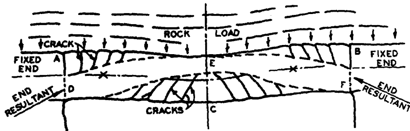
Figure 2-4. Mode of failure of uniform material beam.
