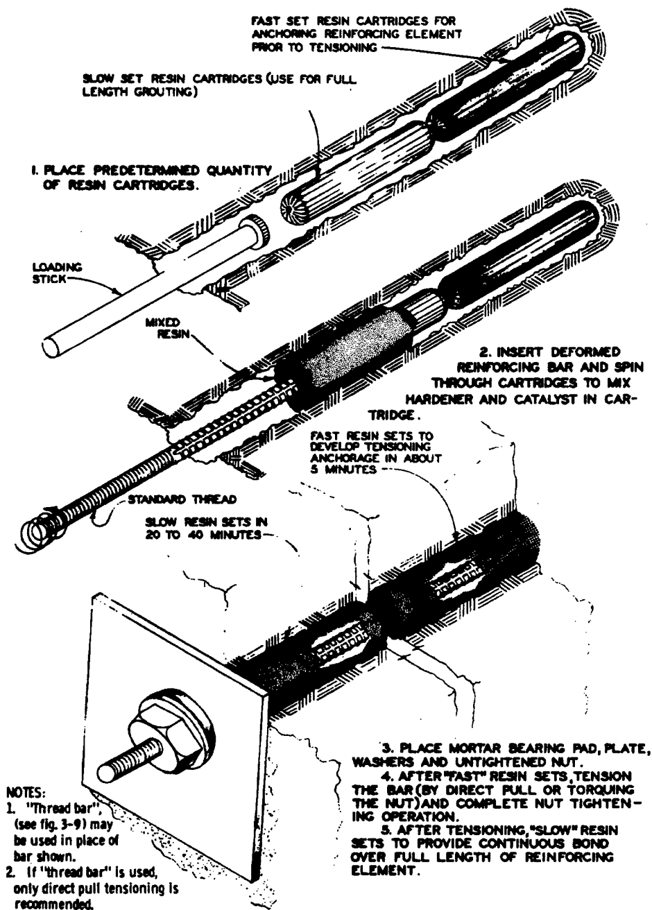
Figure 3-8. Grouted end anchorage, polyester resin (includes full-length bonding technique).
