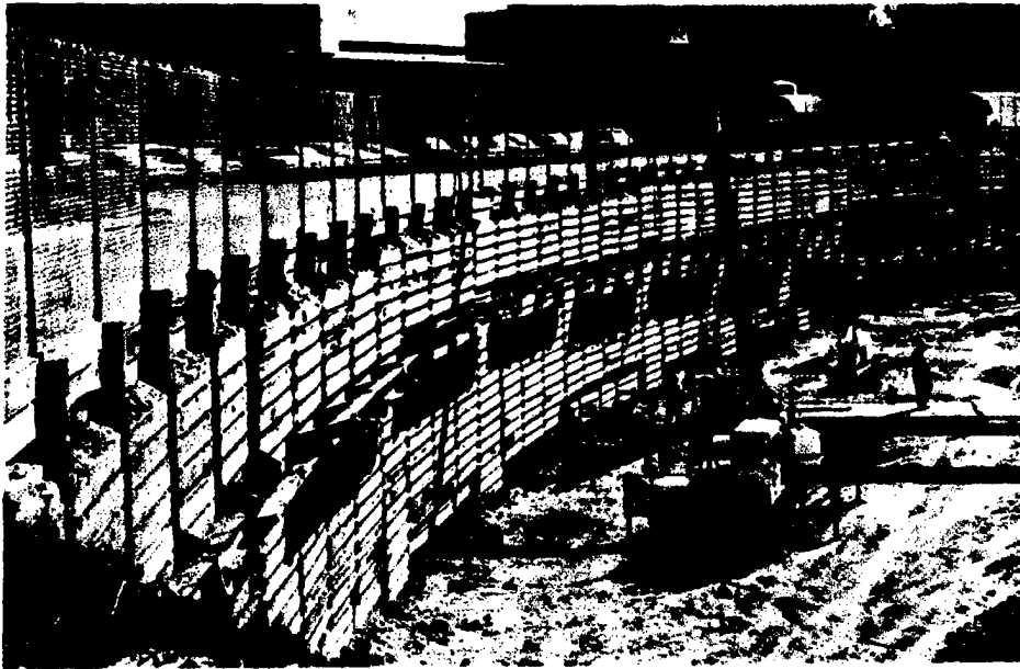
Figure A-1 — Prestressed Soil Anchors used to tie-back a wall of soldier piles with wooden lagging.
