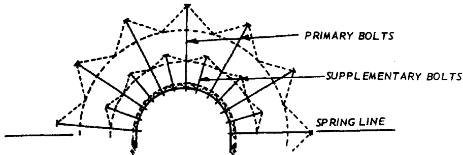
Figure 2-9. Supplementary rock reinforcement.
