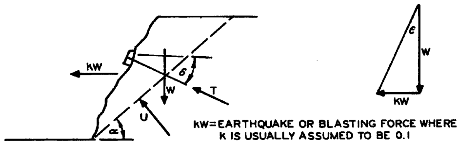
Figure 3-15. Force polygon for earthquake or blasting force.
