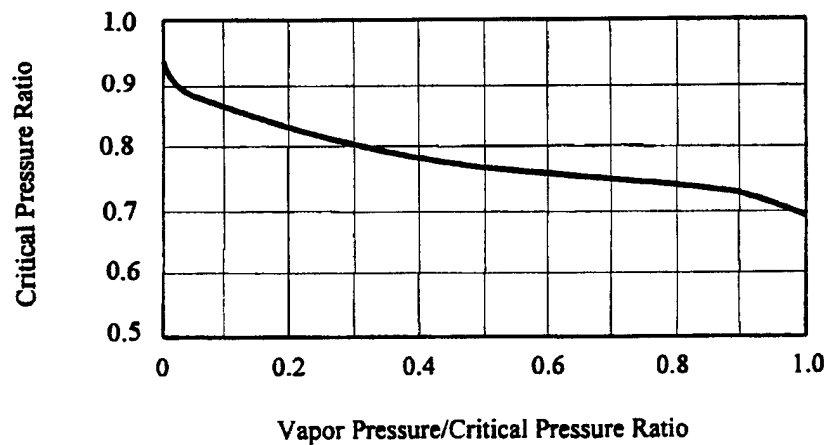
b. Curve for Liquids Other Than Water
