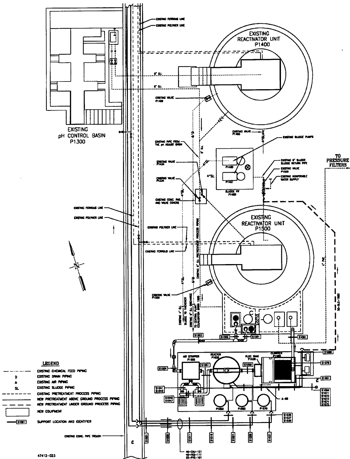
Figure C-4. Piping Layout Plan with Support Locations
