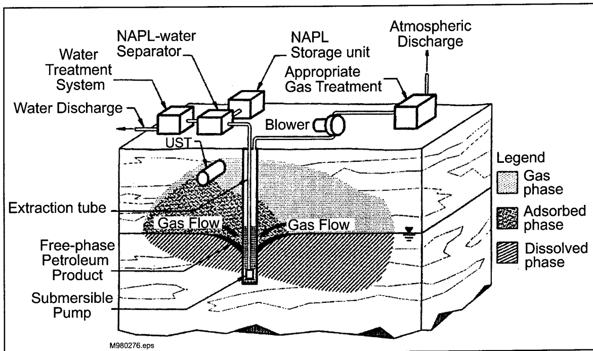
Figure 3-7. Typical Dual-Phase Extraction System. (After USEPA 1995)
