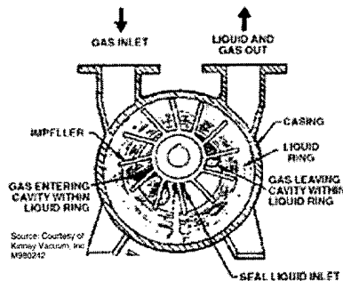
FIGURE 5-5(a): Typical Liquid Ring Pump
