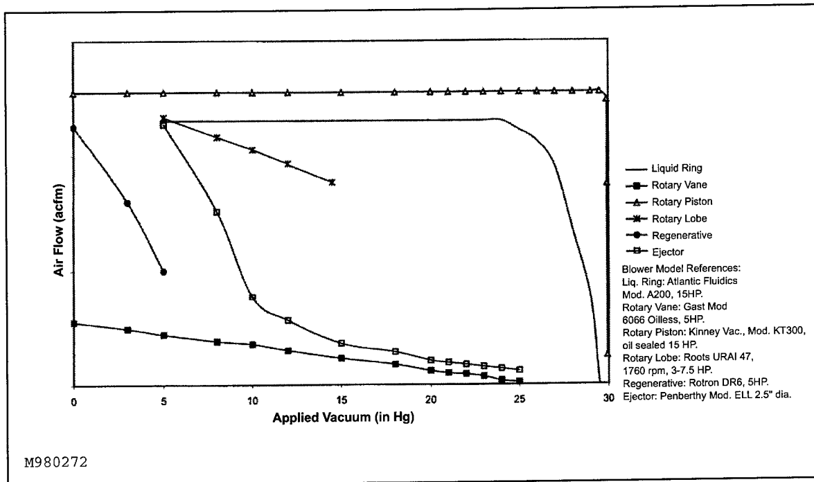
Figure 5-12. Comparison of Air Flow vs. Vacuum for Various Types of Vacuum Pumps.
