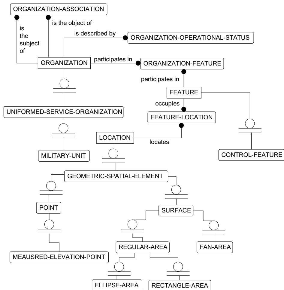
Figure A-2. AICDM Organizations and Locations
