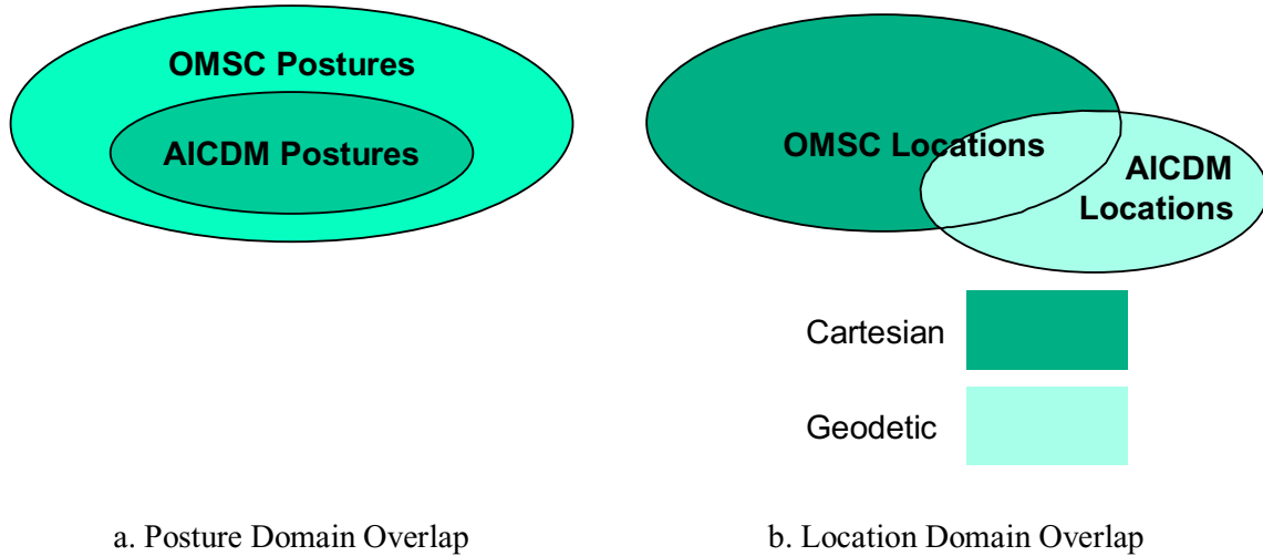
Figure 8. Examples of Value Level Domain Overlap
