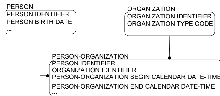
Figure 3. AICDM Representation of Many-to-Many Relationship
