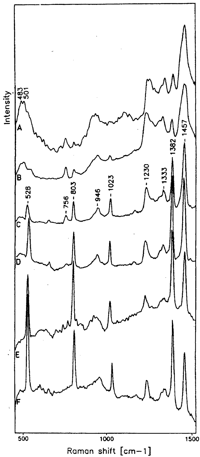
Figure B-5. Raman spectra of phosphate excited with different wavelengths of laser light. (A) 468.0, (B) 476.2, (C) 530.9, (D) 568.2, (E) 632.8, and (F) 647.1 nm laser light.
