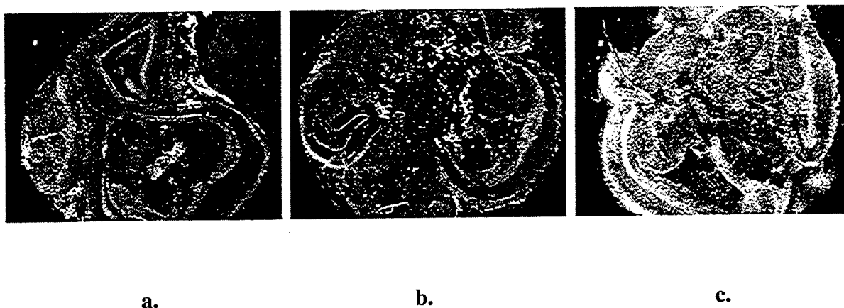
Figure 3-4. 2-DG activity in the brains of bluegills. a. Control. b. Solvent control. c. Brevetoxin-exposed.
