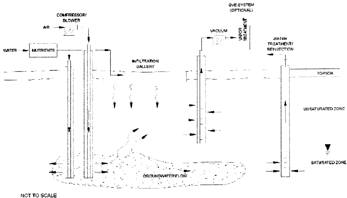
FIGURE 10-1. AIR SPARGING/BIOSPARGING
