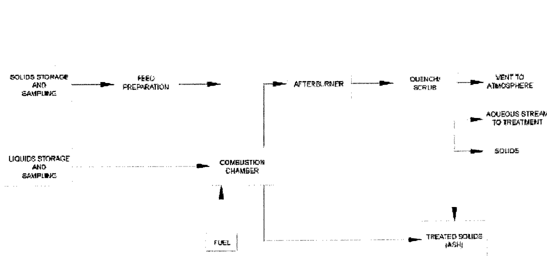
FIGURE 23-1. TYPICAL PROCESS FLOW FOR INCINERATION
