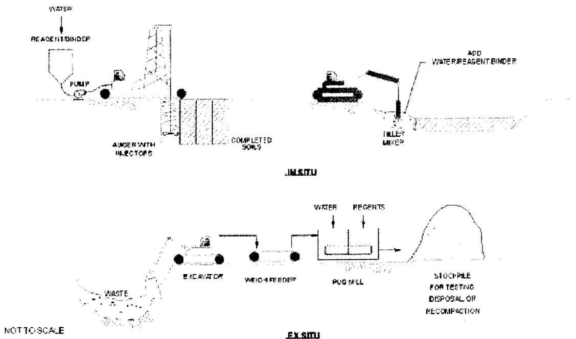
FIGURE 4-1. SOLIDIFICATION/STABILIZATION (IN SITU/EX SITU)
