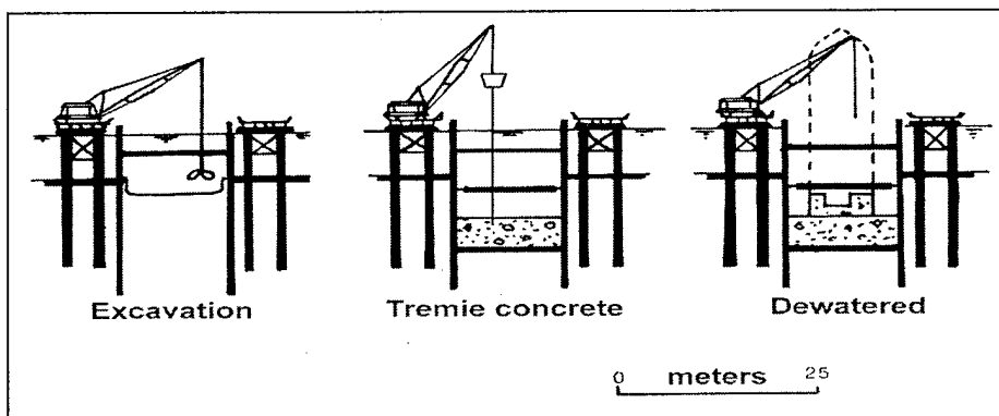
Figure 3. Underwater foundation construction sequence (after Gilbert and Horner 1984)
