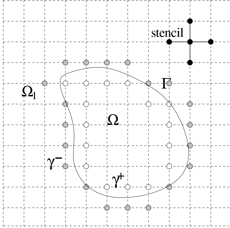
FIG. 3.1. Schematic geometry of the domains, the stencil, and the grid boundary \gamma = \gamma^+ \cup \gamma^- : Hollow bullets — \gamma^+ , filled bullets — \gamma^- .
