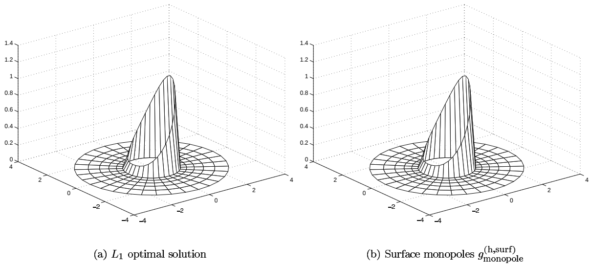
FIG. 4.1. Control sources for L = 32 , J = 7 , k = 0.5 , excitation \delta(x - x_1) , x_1 = (5, 0) .
