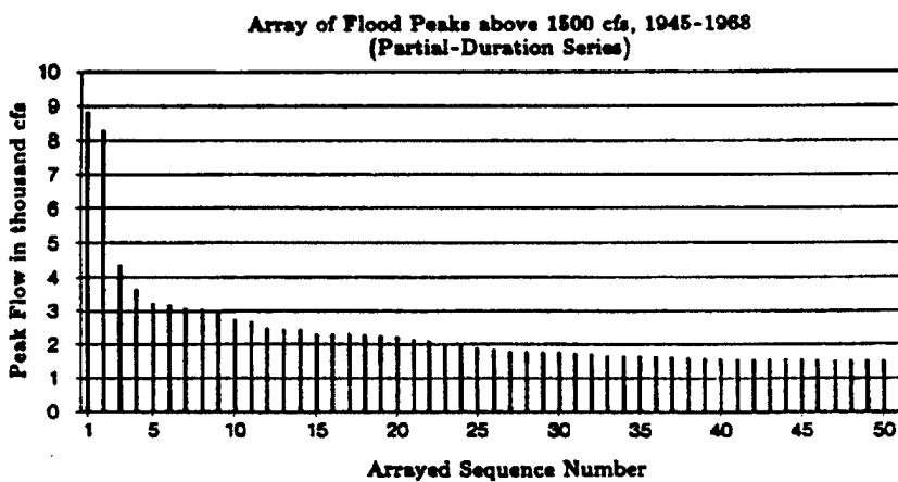
Figure 2-4. Illustration of Chronologic Sequence and Arrayed Flood Peaks.
