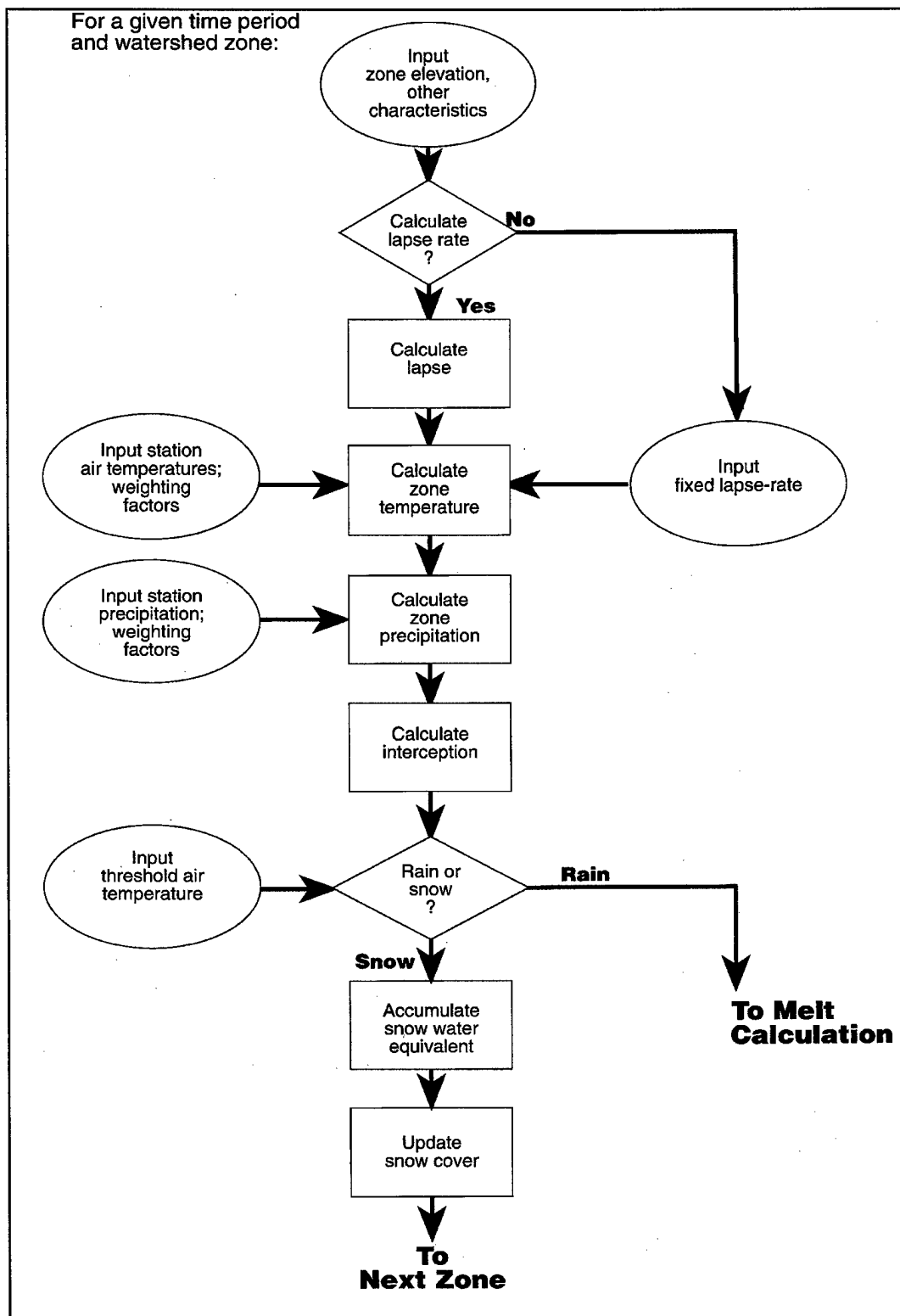
Figure 4-5. Algorithm of snow accumulation variation
