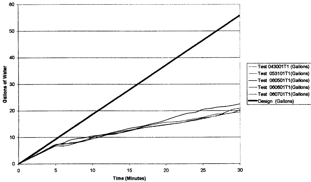
FIGURE 33. WATER MIST SYSTEM WATER FLOW HISTORY DURING THE MPS AEROSOL CAN EXPLOSION TESTS
