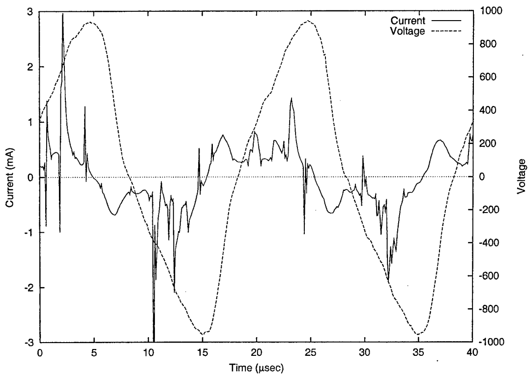
Figure 8: Discharge current and voltage for a glass frit with nominal pore diameter 8 \mu\text{m} in He. The pressure on one side of the frit was 420 Torr, and the pressure on the other side was about 100 Torr.
