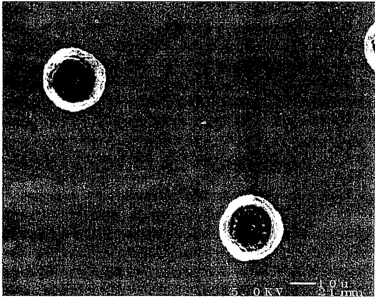
Figure 4: Top view of two of the holes etched in a silicon wafer.
