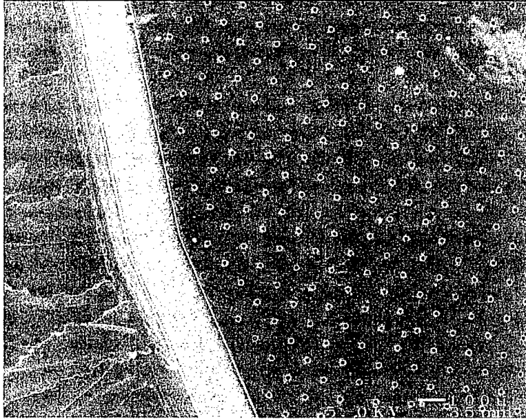
Figure 3: SEM photomicrograph of the etched pattern on a silicon wafer.
