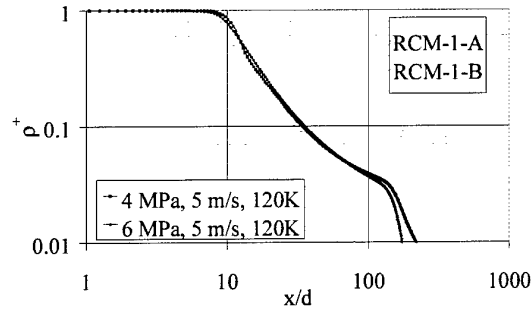
Figure 19: Density; 5 m/s, 120 K
