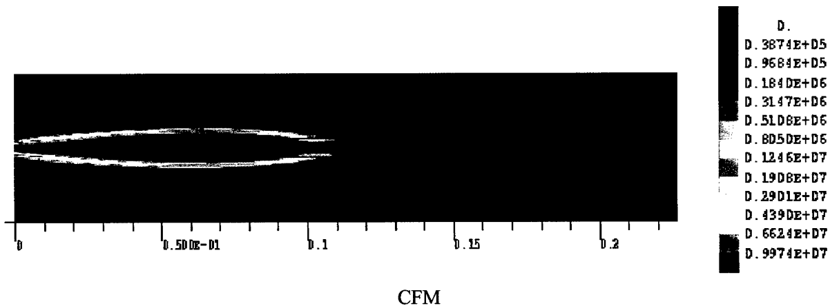
Figure 10 : Reactive rate (mol/kg/s) : Gas – Liquid (~1:1), k - ε, oxygen (injection)
