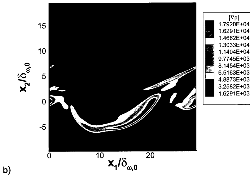
Figure 8: Density gradient magnitude (in \text{kg/m}^4 ) for R750 at t^* = 150 , a) in the braid plane ( x_3 = L_3/16 ) and b) in the between-the-braid plane ( x_3 = L_3/2 ).
