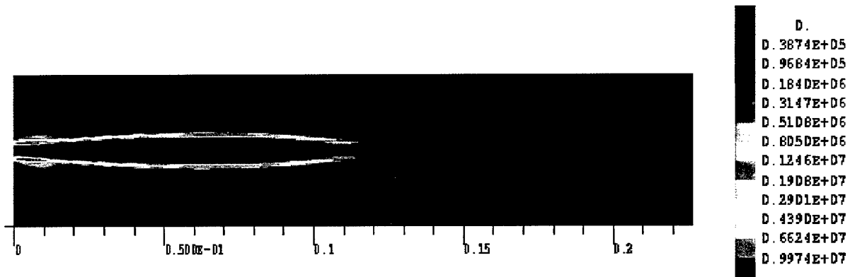
Figure 14 : Reactive rate (mol/kg/s) : Liquid, q - ω, oxygen (injection except \sigma )
