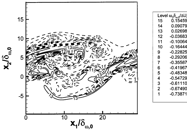
Figure 6: Nondimensional spanwise vorticity for R750 in the braid plane ( x_3 = L_3/16 ) at a) t^*=80 and b) t^*=150 .
