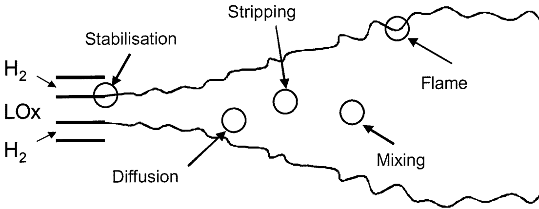
Figure 3 : Physical phenomena in supercritical condition.
