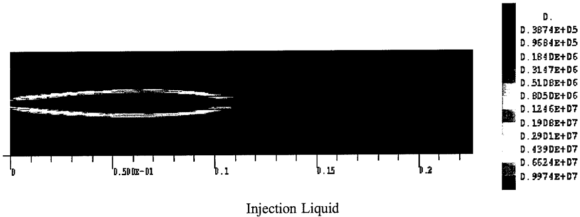
Figure 6 : Reactive rate (mol/kg/s) : CFM, q - \omega ; oxygen (injection)
