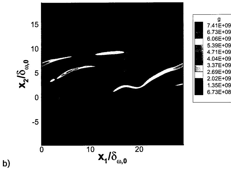
Figure 11: Dissipation (in J/m^3K ) for R750 at t^*=150 , a) in the braid plane and b) in the between-the-braid plane.
