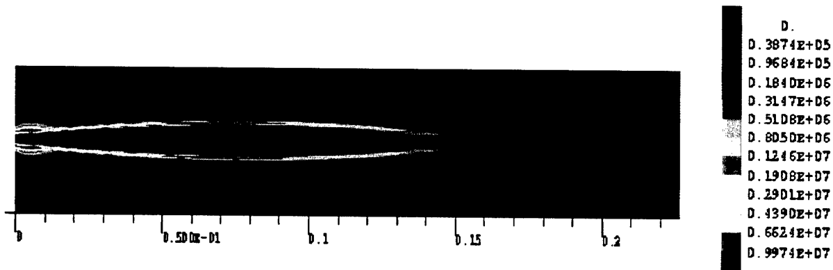
Thermodynamics properties at 85 K (Injection)
