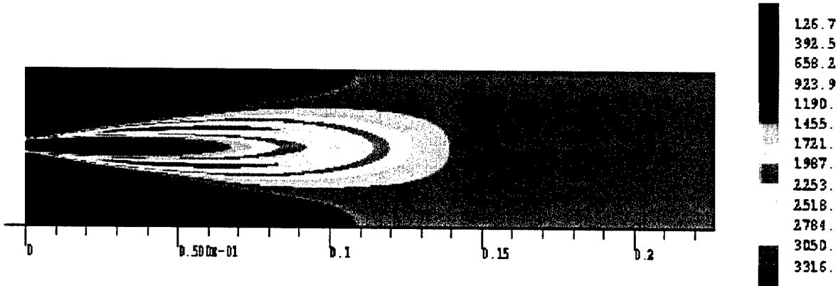
Figure 15 : Temperature (K)
