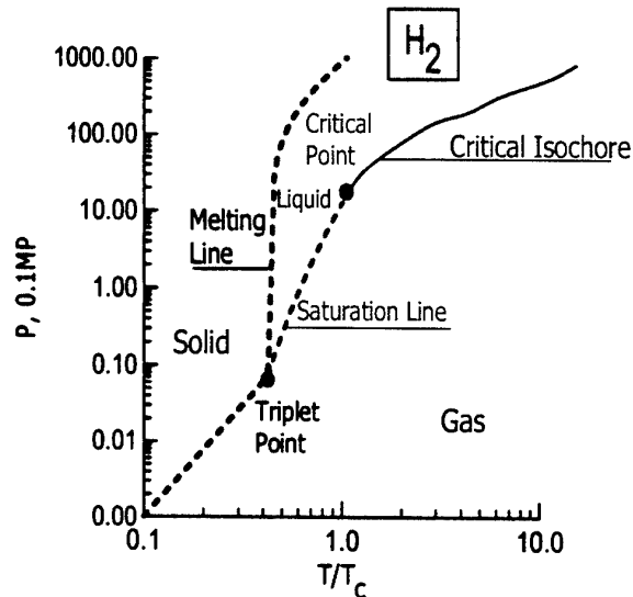
Fig. 2: Phase diagram of H_2
