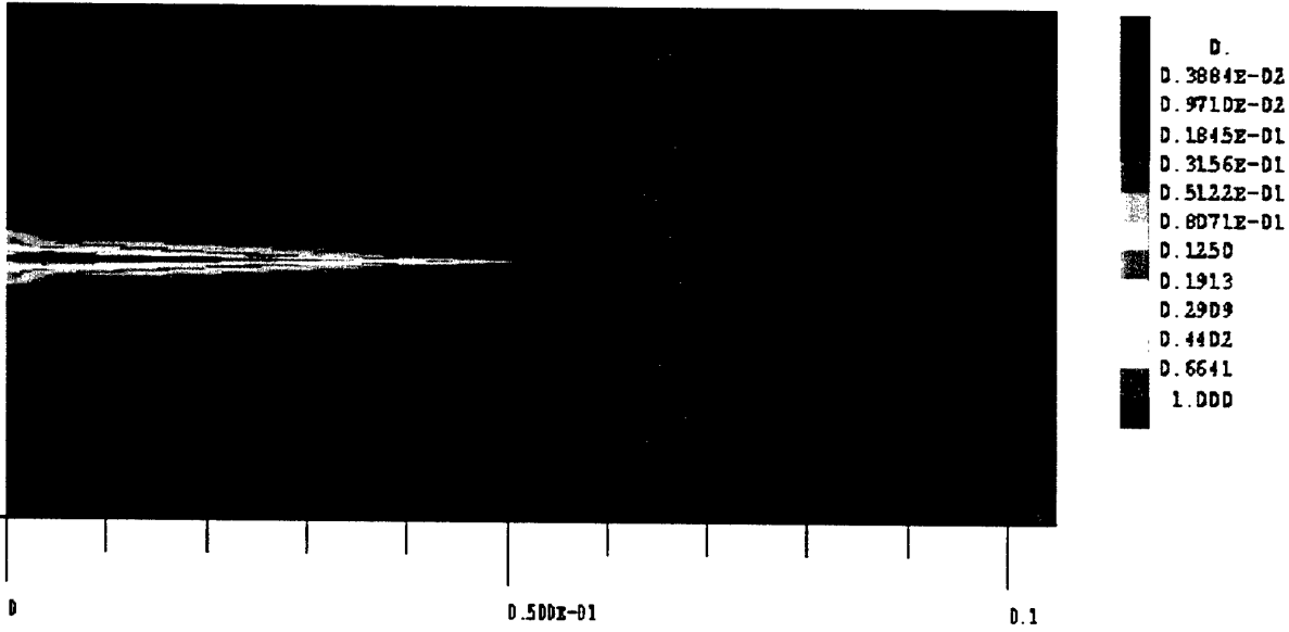
Figure 8 : Liquid oxygen volume fraction
