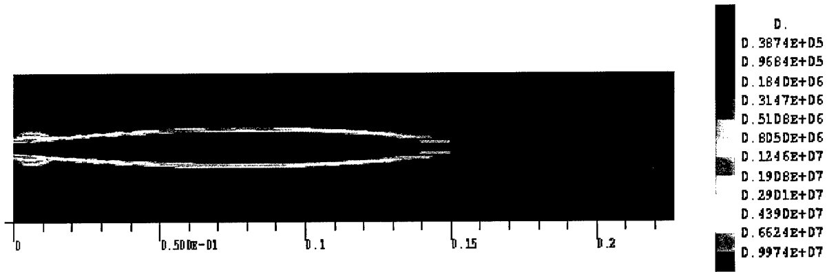
Figure 13 : Reactive rate (mol/kg/s) : CFM, k - ε, Gas – Liquid (~1:1)
