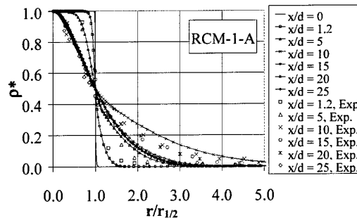
Figure 6: Density; 4 MPa, 5 m/s, 120 K
