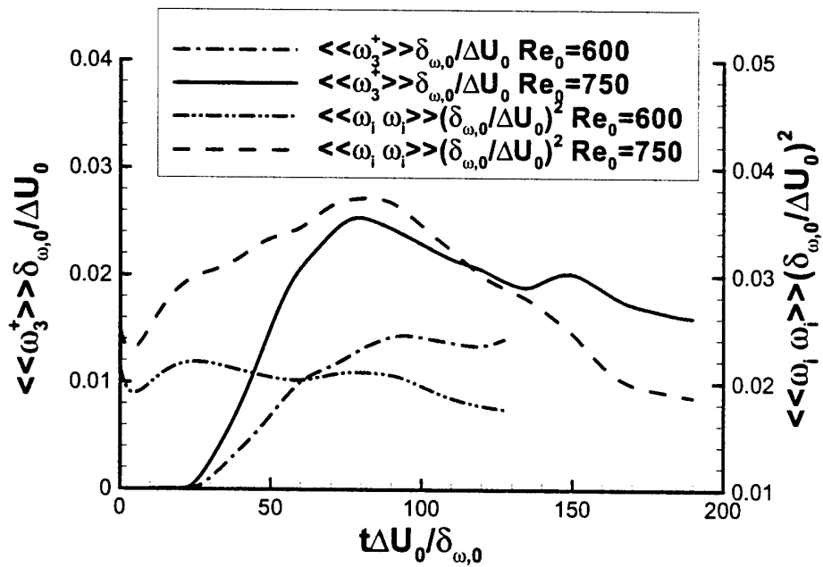
Figure 3: Time evolution of a) momentum and product thicknesses and b) global spanwise vorticity and enstrophy.
