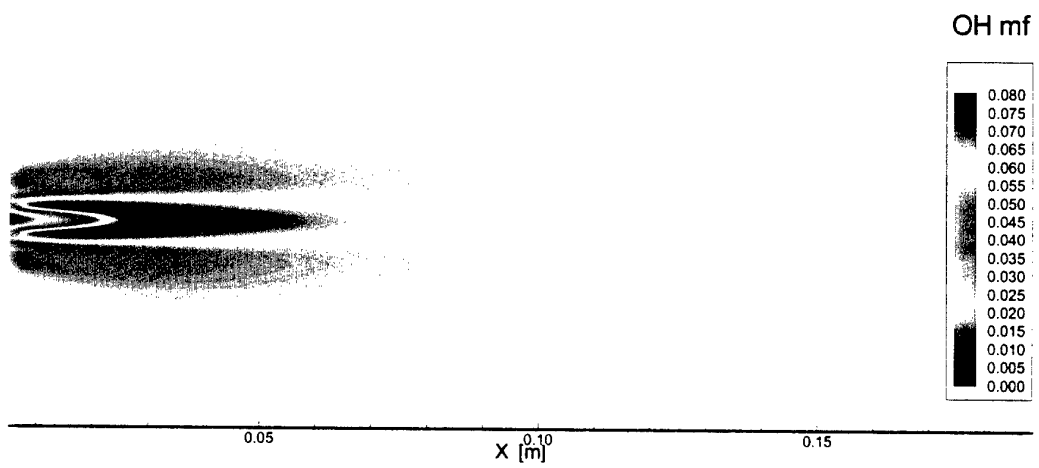
Figure 5: OH Mass Fraction Contours for Concept 1 (top), 2 (middle) and 3 (bottom)
