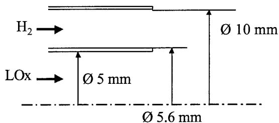
Figure 1 : injector geometry
