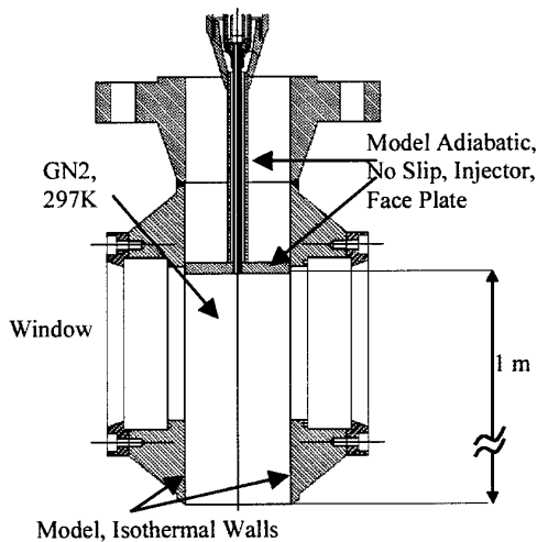
Figure 2: Test chamber
