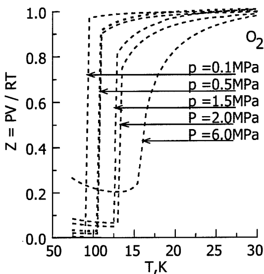
Fig. 3: Compressibility factor Z = \frac{pV}{RT}
