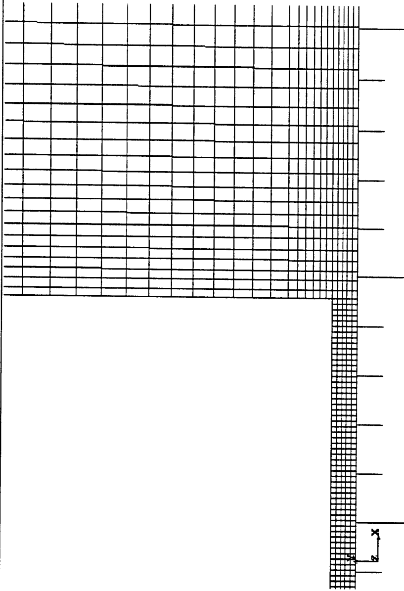
Mesh RCM1 Zoom
