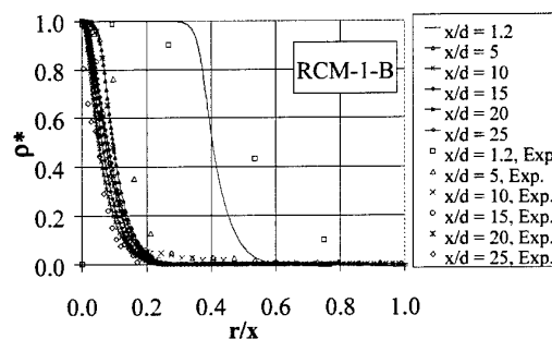
Figure 7: Density; 6 MPa, 5 m/s, 120 K
