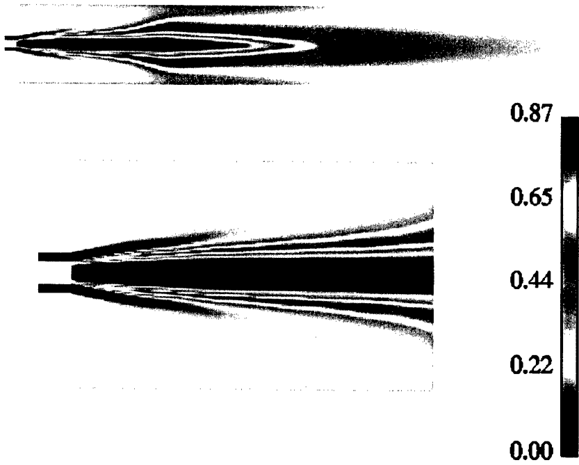
Fig. 7: Water Vapour mass fraction fields
