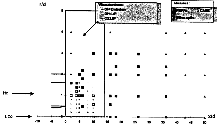
Figure 4: CARS, PDPA, and fiber optic measurement locations
