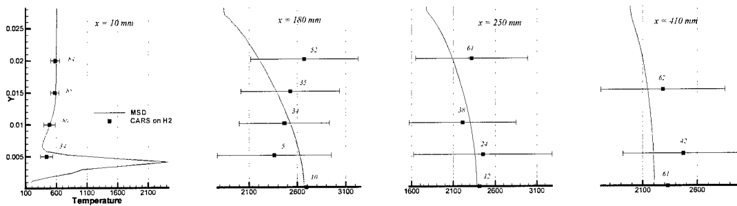
Figure 12 : Temperature radial profiles – Comparison of computations and experimental data
