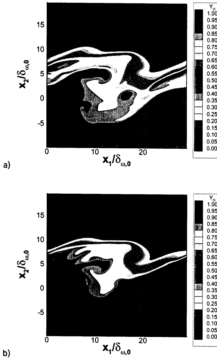
Figure 9: Oxygen mass fraction for R750 at t^* = 150 , a) in the braid plane, b) in the between-the-braid plane and c) in the streamwise mid-braid plane.
