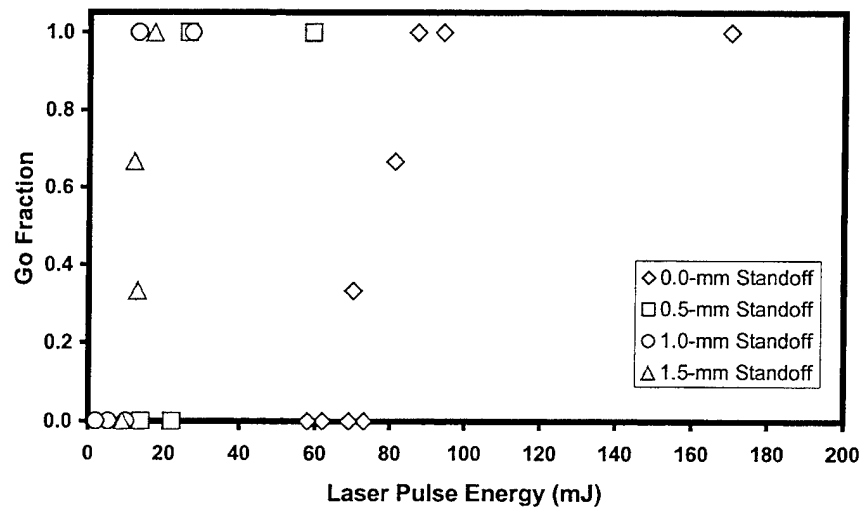
Figure 8. Plot of Go Fraction vs. total incident laser pulse energy for 6-mm bead, 4.76-mm beam diameter.
