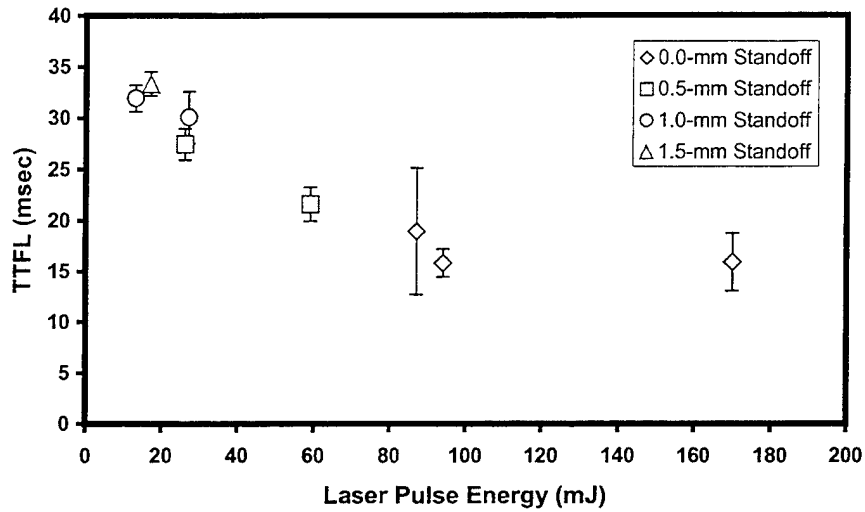
Figure 10. Time-to-first-light vs. estimated laser pulse energy for the ignition of black powder using a 6-mm diameter bead lens and a 4.76-mm diameter laser beam.
