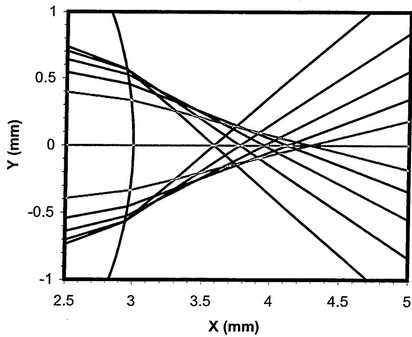
Figure 4. Refraction of 4.76-mm diameter beam passing through 6-mm diameter glass bead.
