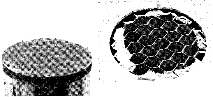
Figure 7 Failure surfaces resulting from tensile testing of the Untreated honeycomb and AF130-2 adhesive conditioned 30 days at 70°C/100%R.H., indicating fillet bond pull-out.
