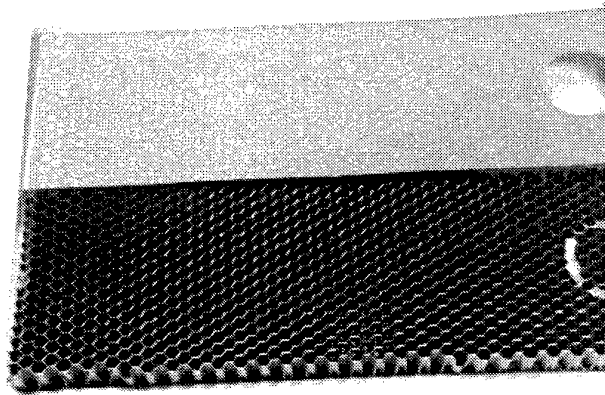
Figure 16 Failure surfaces resulting from peel testing of the Untreated honeycomb and AF130-2 adhesive conditioned 30 days at 70°C/100% R.H., indicating fillet bond pull-out.
