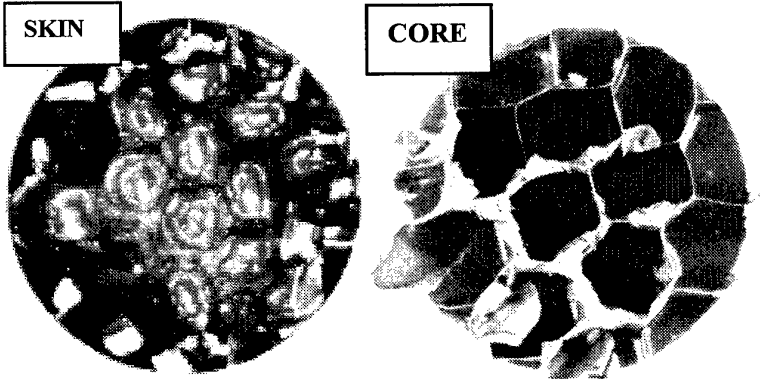
Figure 32 Failure surface images from the tensile test taken in location 3, refer Table 3, of the Sta-Tip Cap, where an ineffective injection repair has degraded the honeycomb panel strength.
