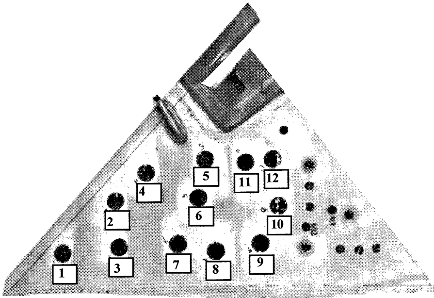
Figure 23 Locations of tensile test measurements taken from the Stab-Tip, prior to conditioning.
