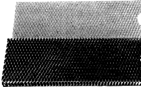
Figure 14 Failure surfaces resulting from peel testing of the Dura-Core honeycomb and JD Lincoln adhesive conditioned 150 days at 70°C/100% R.H., indicating fillet bond pull-out.
