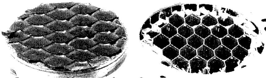
Figure 5 Failure surfaces resulting from tensile testing of the Dura-Core honeycomb and JD Lincoln adhesive conditioned 150 days at 70°C/100%R.H., indicating fillet bond pull-out.
