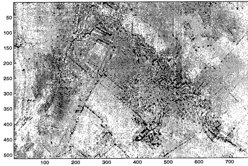
Figure 7.1.4. The result of applying the projection discriminating textural (periodic) information constructed from 2-dimensional idempotents of one of the realizations of (C_N \times C_N) \not\sim C_4 .
