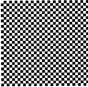
Figure 6.19.1. Image of 32 \times 32 of alternating intensity of 0 and 2.
