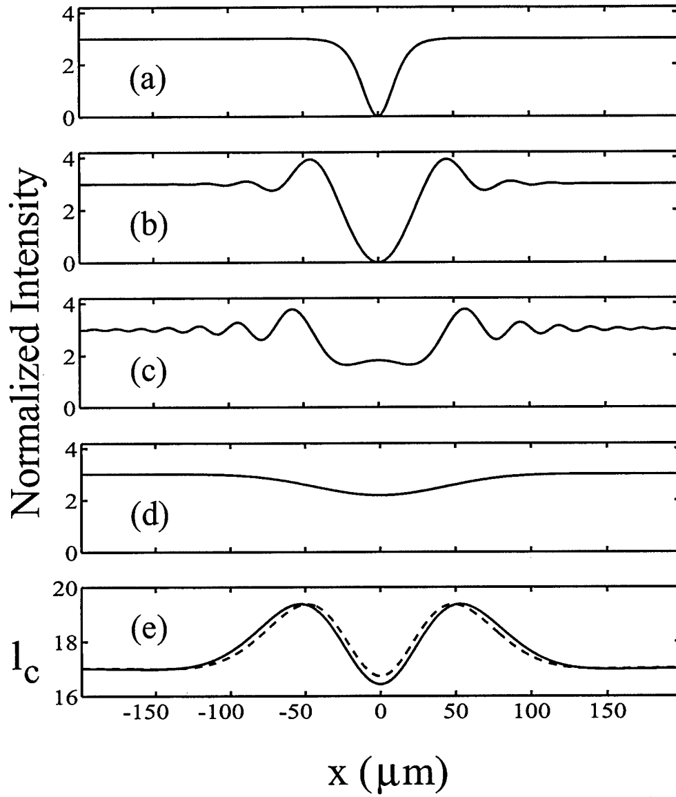
Figure 8.1: (a) Intensity profile of a 25\ \mu\text{m} odd or even dark beam at the input. Diffraction of an (b) odd coherent dark beam, (c) even coherent dark beam, (d) incoherent odd or even dark beam with l_c = 7.3\ \mu\text{m} after 12\ \text{mm} of propagation. (e) l_c in \mu\text{m} as a function of x for the odd (dashed curve) and even (solid curve) diffracted incoherent dark beam shown in (d).
