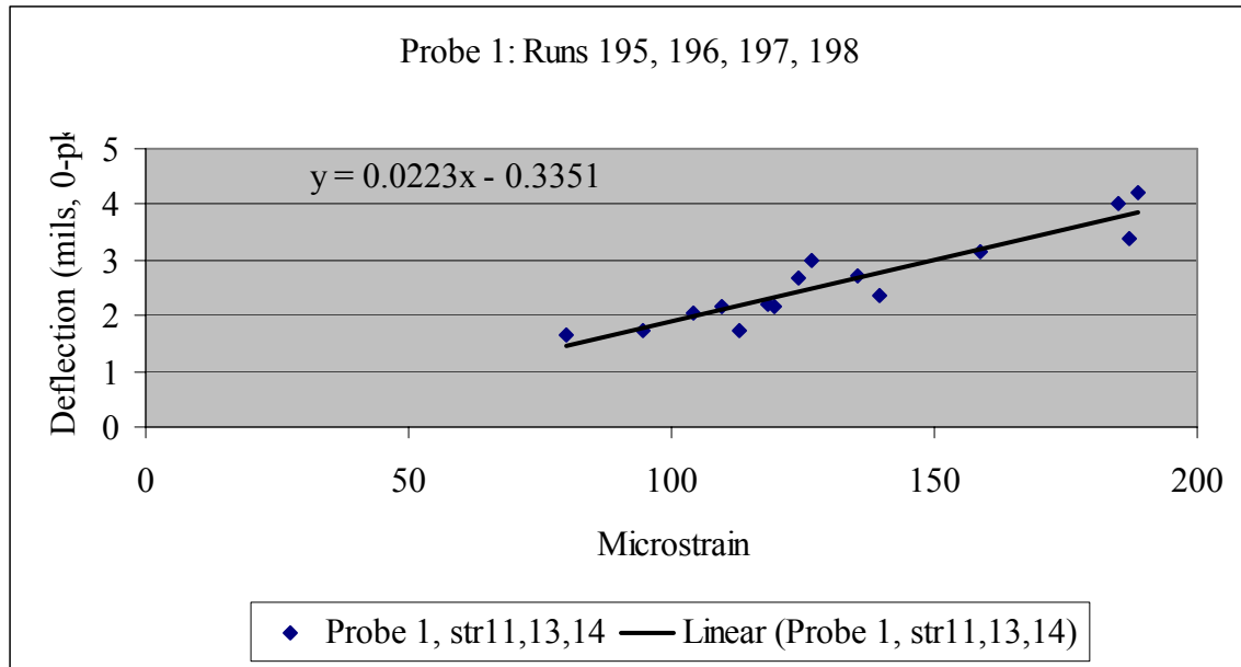
Figure 29 Probe 1 NSMS Correlation to Strain Gauges
