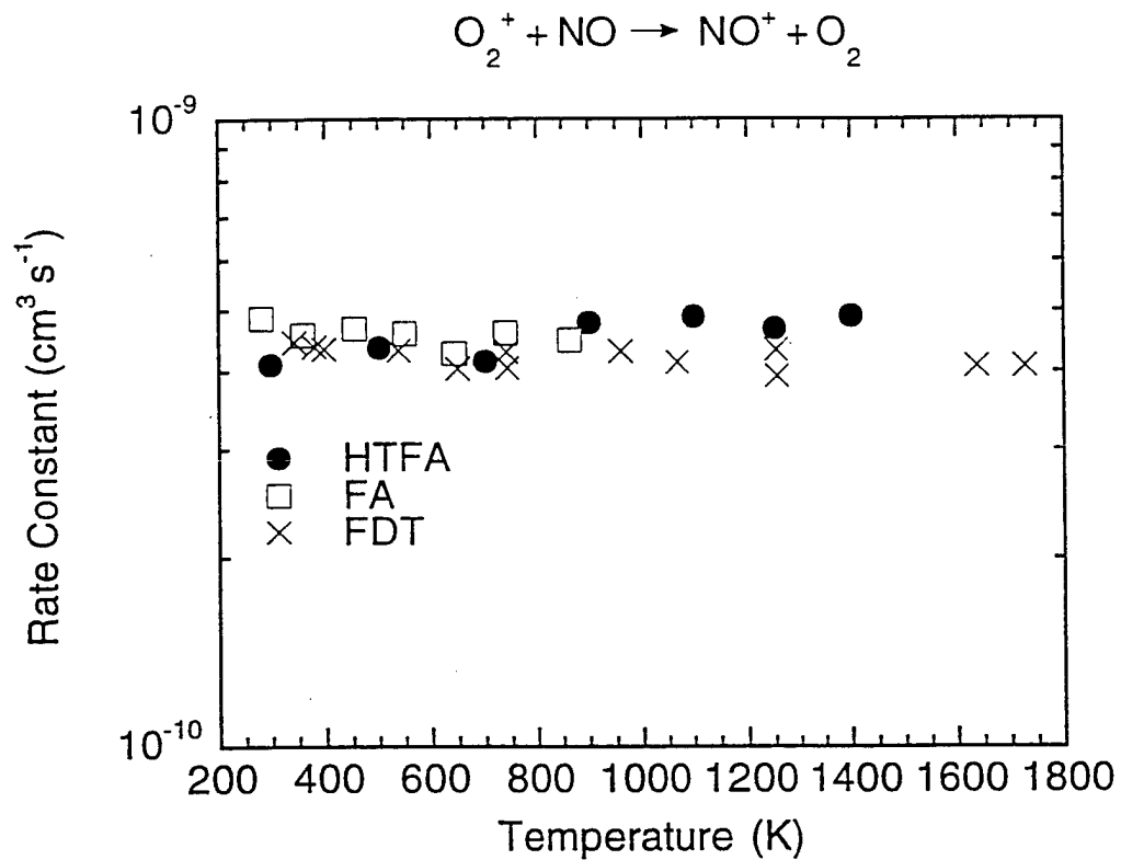
Figure 3: Rate constants for the charge transfer reaction of O_2^+ + NO plotted against the temperature in K. The HTFA results are the current results and the FDT and FA points are the flow drift tube and flowing afterglow results, respectively, of Lindinger et. al. 8,9
