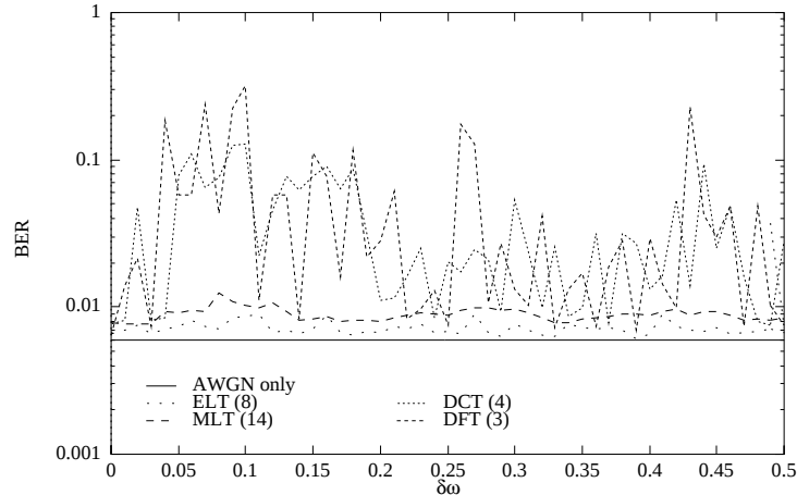
Figure 17: Excision in the presence of single-tone interference as a function of frequency, E_b/N_0 = 5 dB and JSR = 20 dB.
