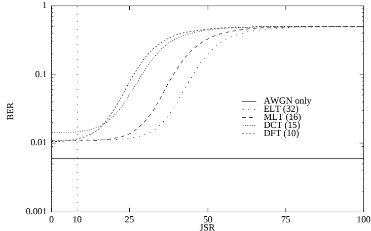
Figure 19: Excision in the presence of narrow-band Gaussian interference as a function of JSR, E_b/N_0 = 5 dB, \delta\omega = 0.126984 rad/sec and \rho = 0.1 .
