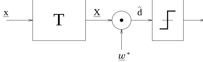
Figure 4: Receiver employing pre-correlation transform domain Wiener filtering.
