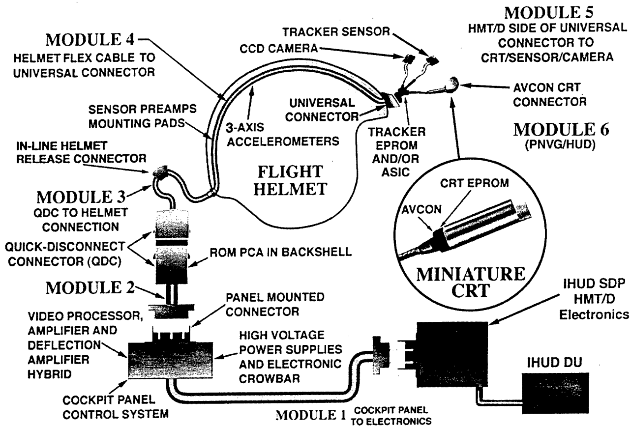
FIGURE 2 Schematic Diagram of HVI Wiring Interconnect
