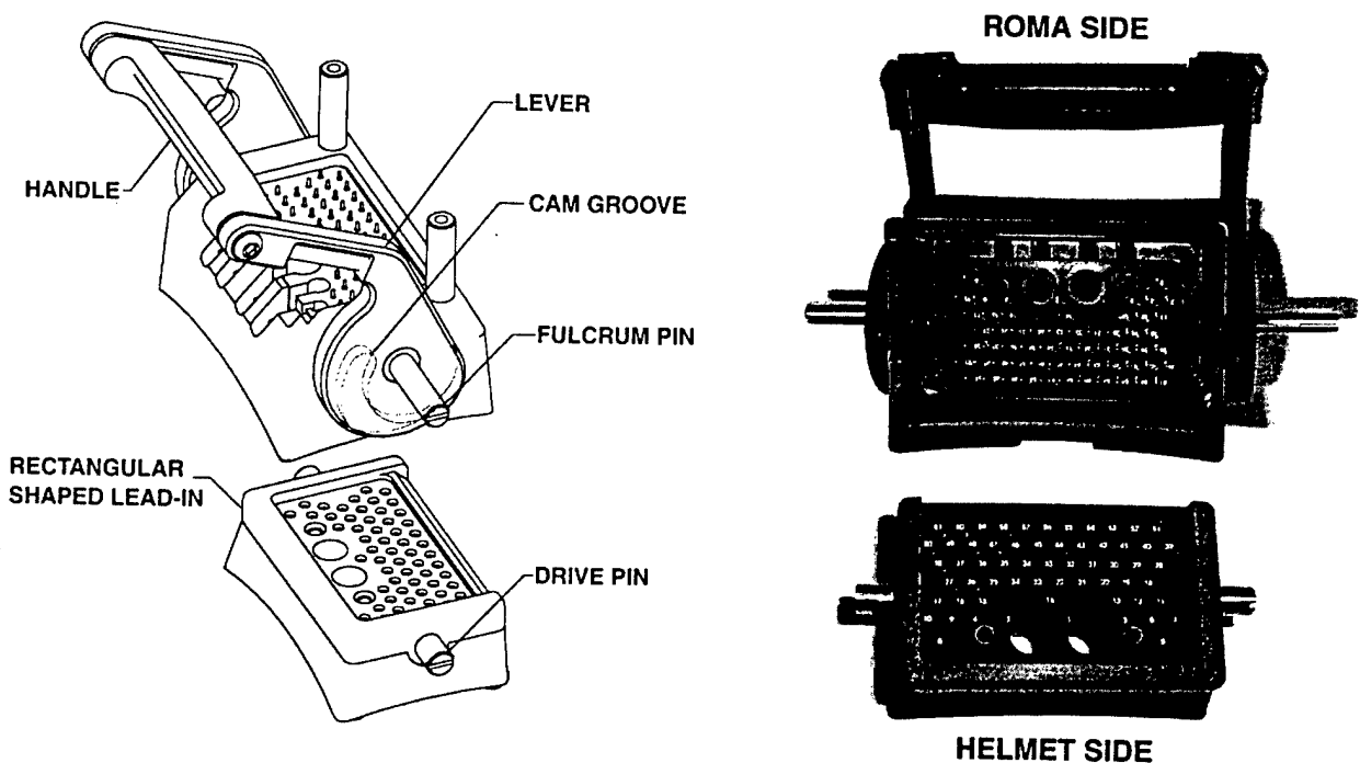
FIGURE 9 Universal Connector Installed in HGU-55/P Lightweight Helmet Shell
