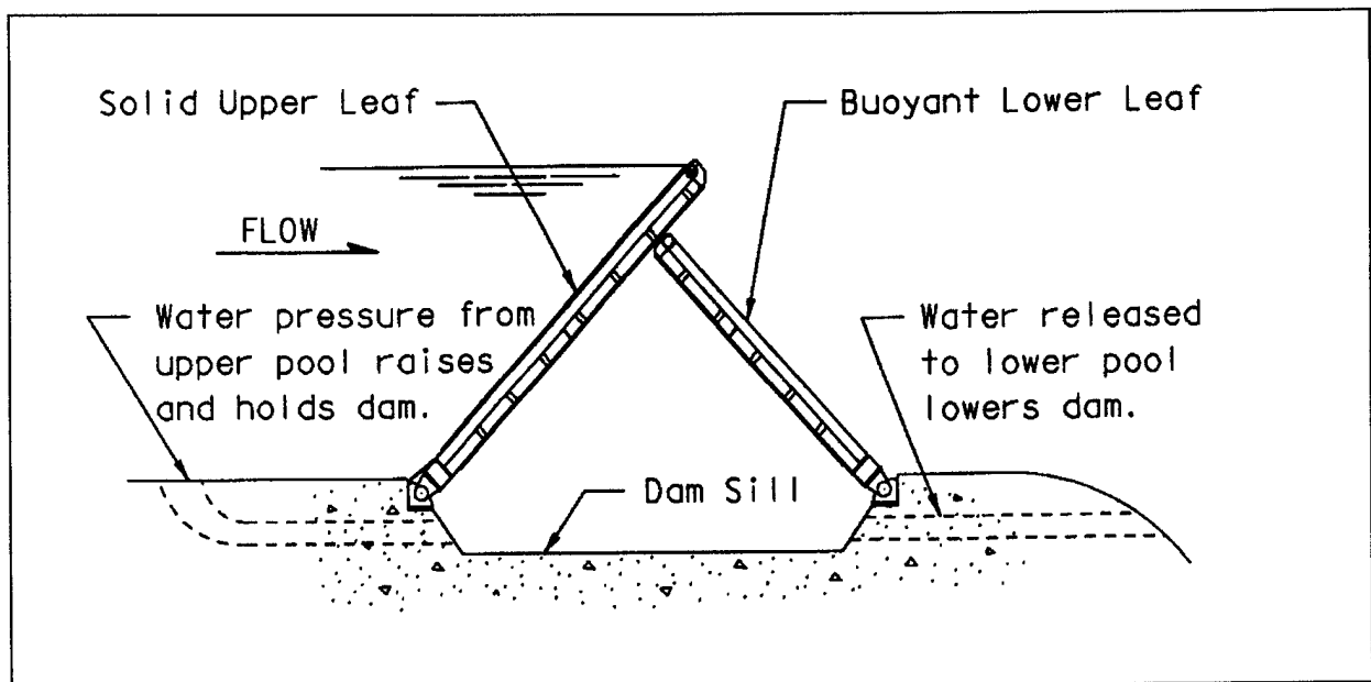
Figure 5-6. Bear trap gate
