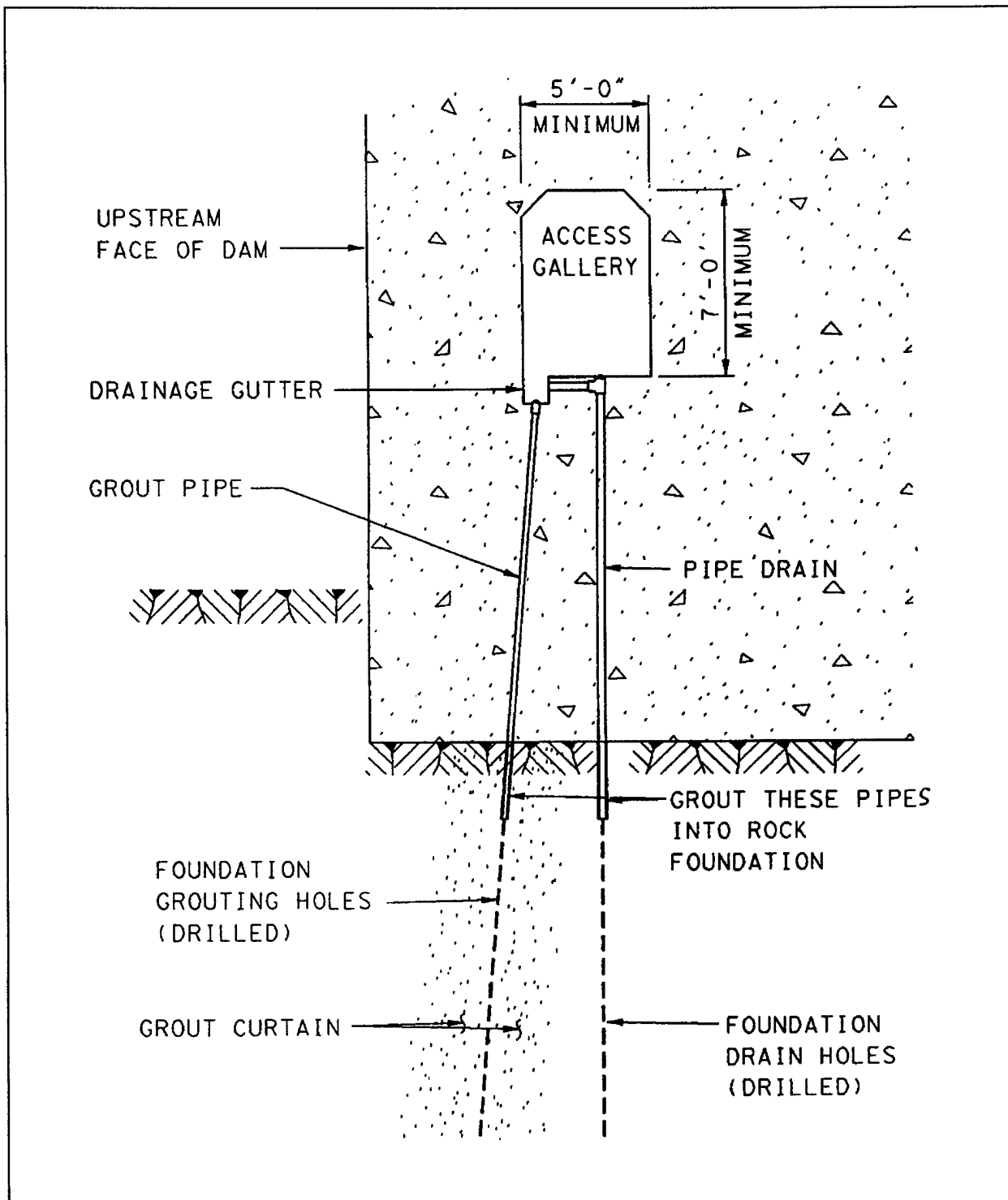
Figure 7-1. Typical grouting and drainage curtain
