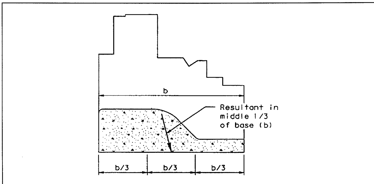
Figure 10-2. Location of resultant
