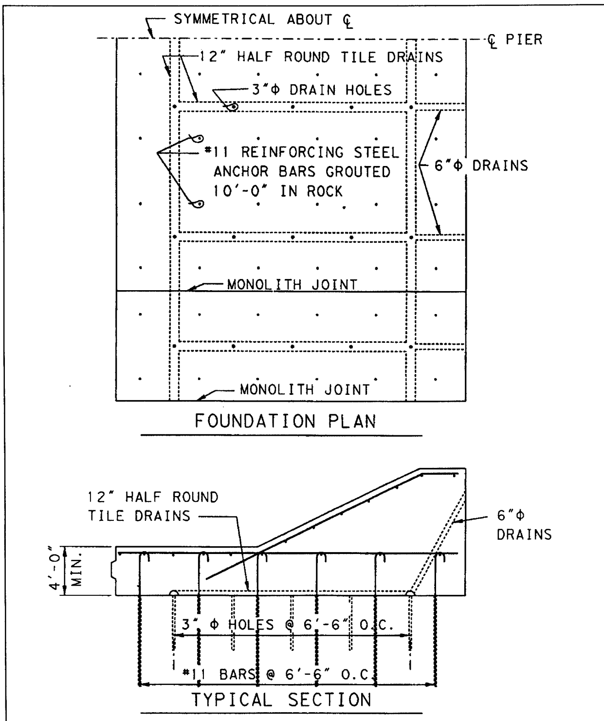
Figure 7-2. Stilling basin drainage and anchorage
