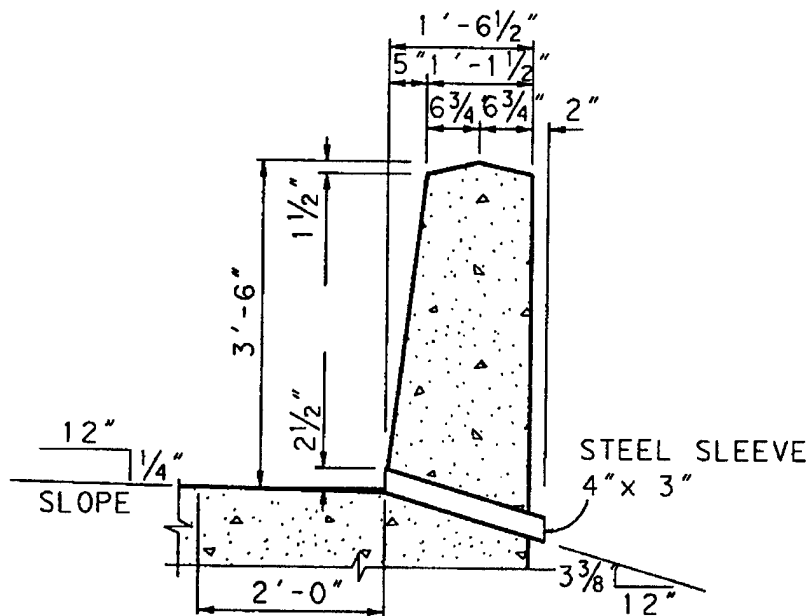
DRAIN SECTION (A)
