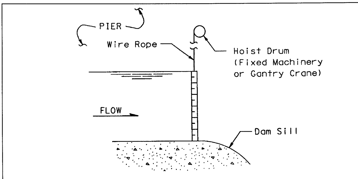
Figure 5-3. Vertical-lift gate
