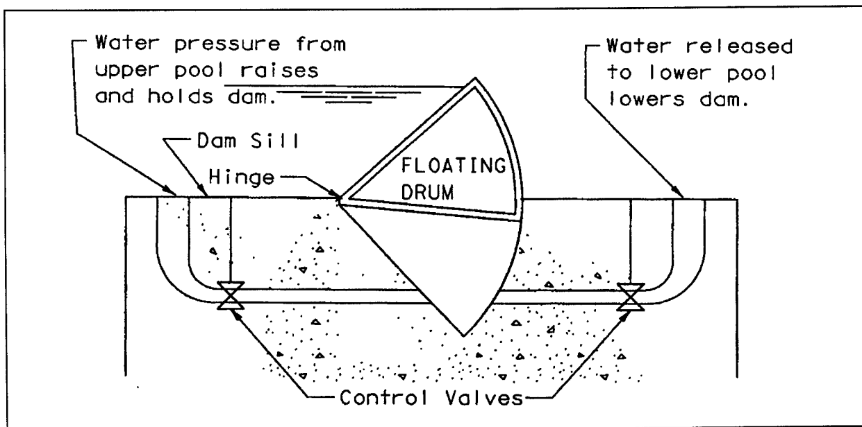
Figure 5-7. Drum gate
