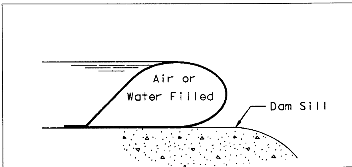
Figure 5-8. Inflatable rubber gate
