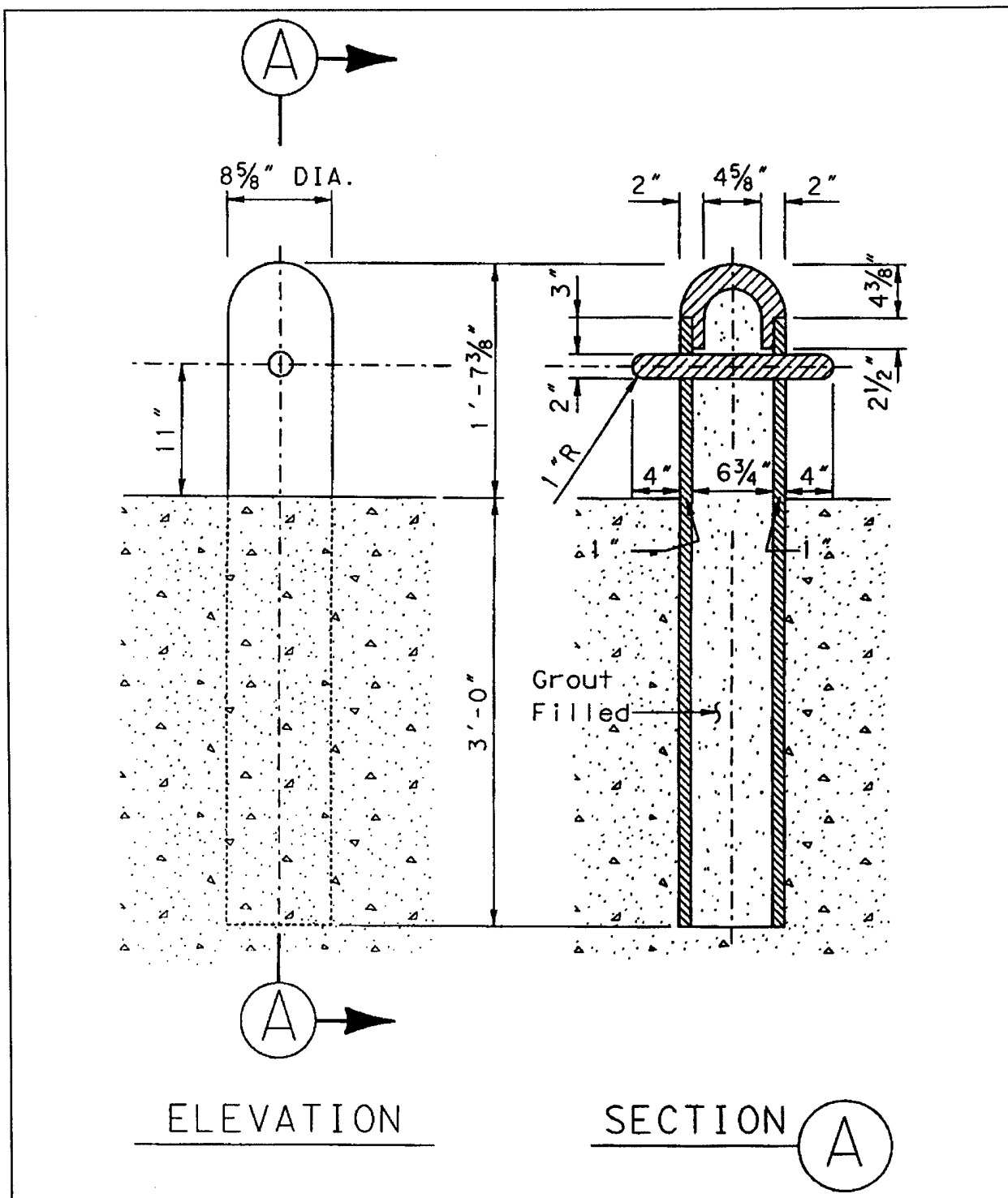
Figure 13-2. Check post detail
