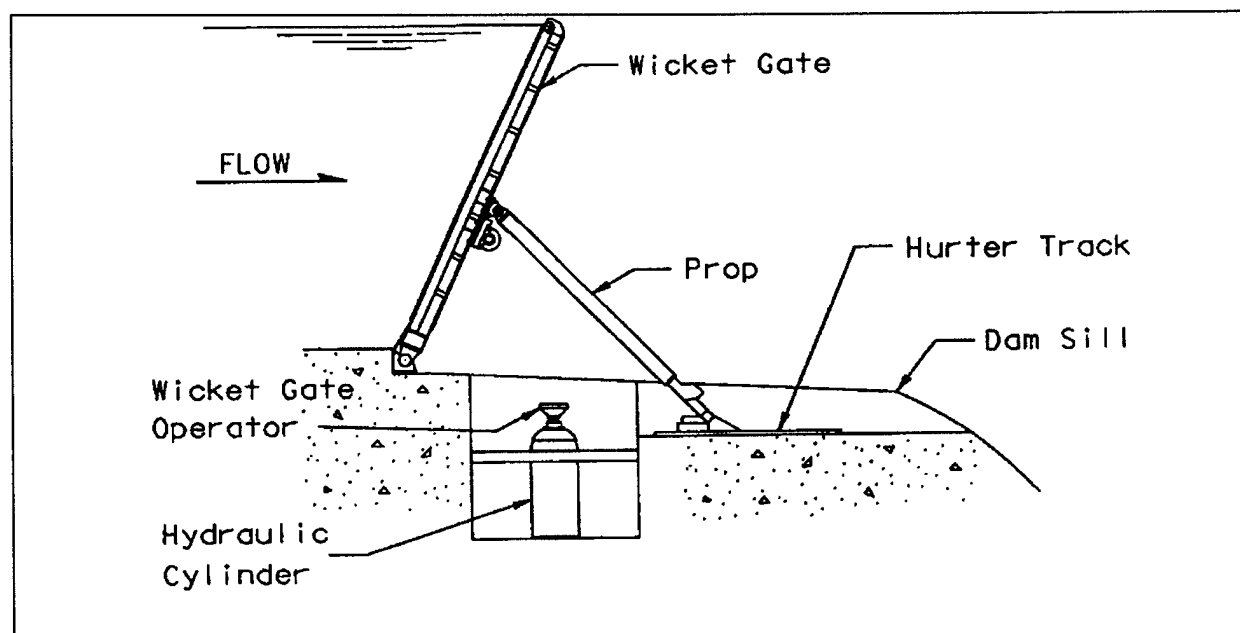
Figure 5-5. Wicket gate
