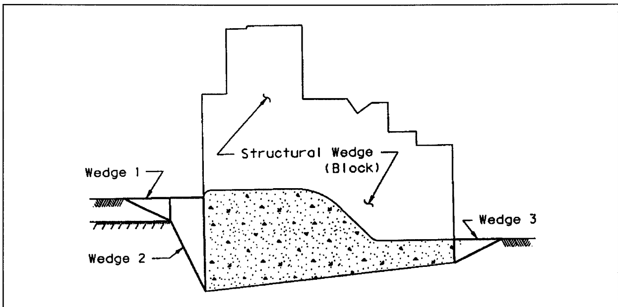
Figure 10-1. Wedge analysis model
