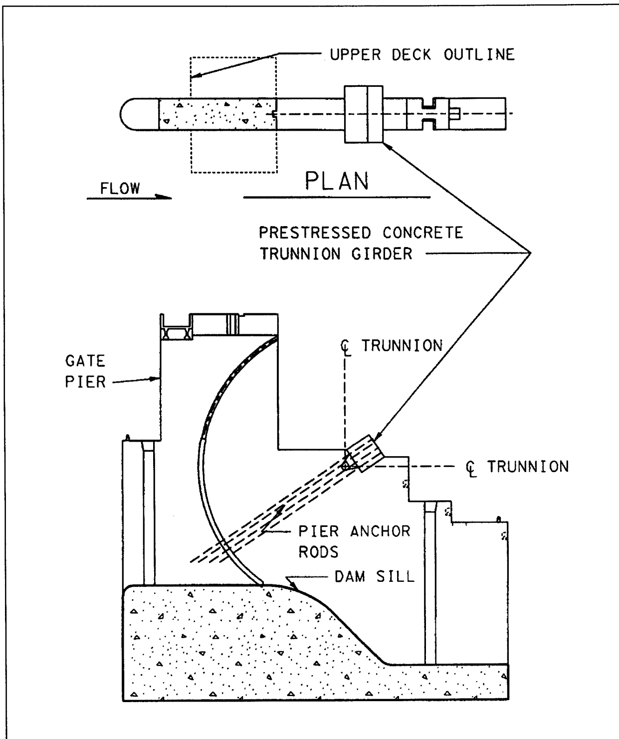
Figure 5-9. Prestressed concrete trunnion girder and anchor rods
