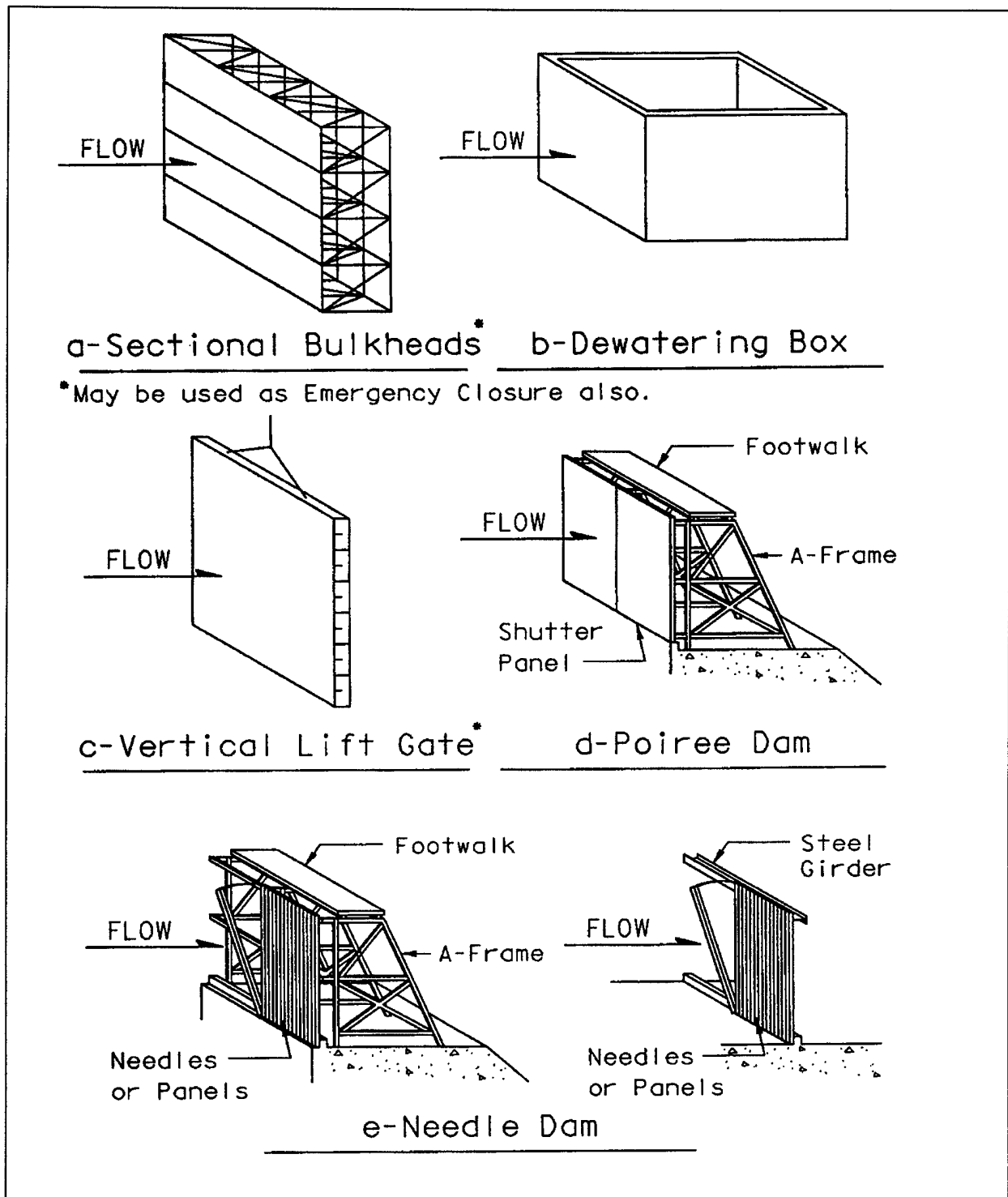
Figure 6-1. Maintenance closures
