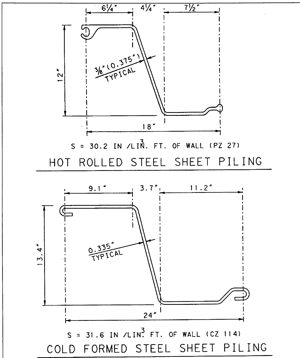
Figure 7-3. Steel sheet piling
