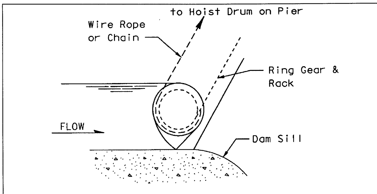
Figure 5-4. Roller gate
