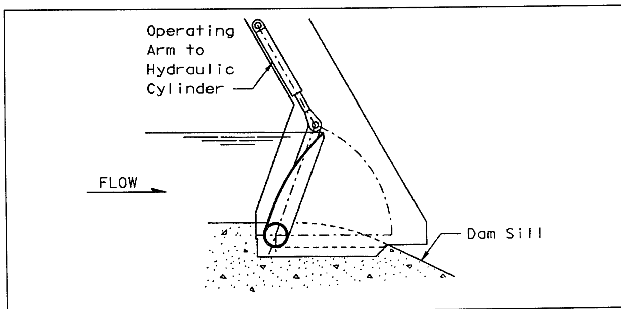
Figure 5-2. Hinged-crest gate
