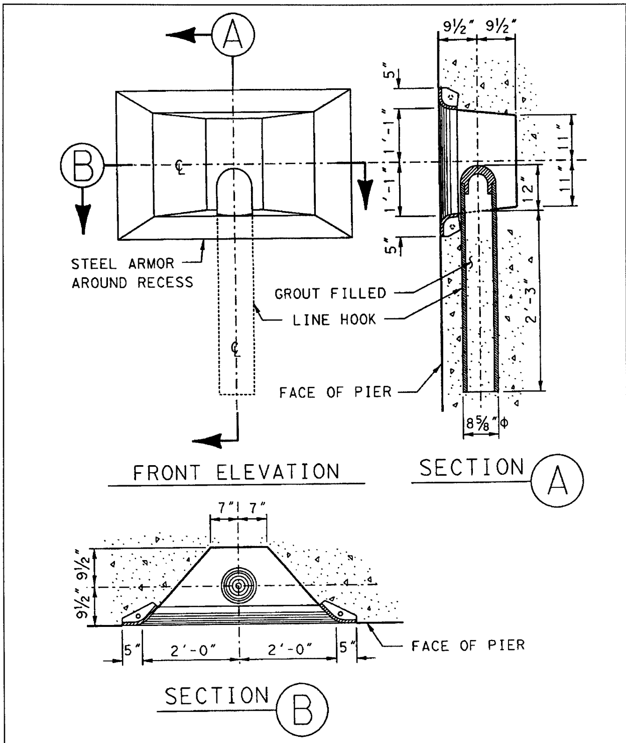
Figure 13-1. Line hook recess detail
