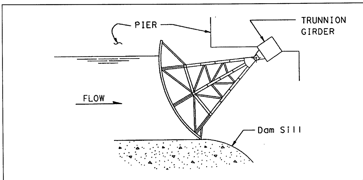
Figure 5-1. Tainter gate
