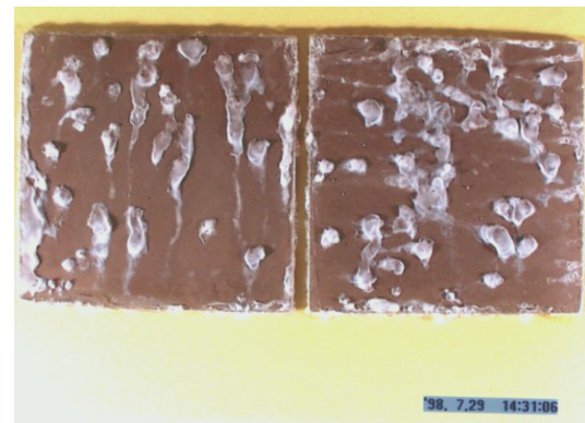
Figure 7. Hard Anodized after Salt Spray
