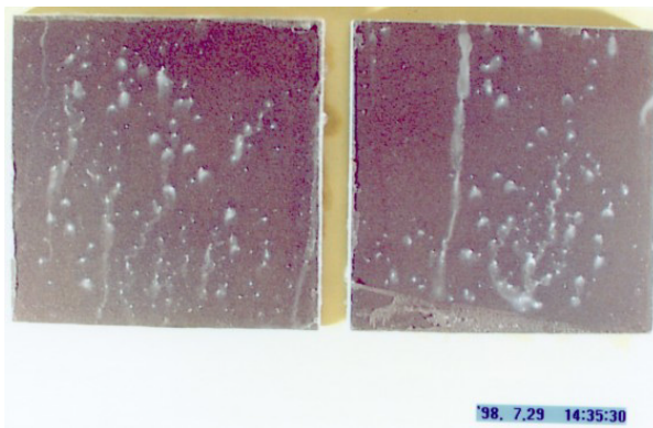
Figure 10. Teflon® after Salt Spray
