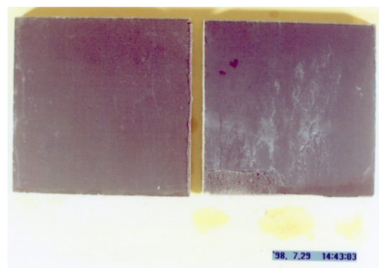
Figure 11. Tufram® after Salt Spray
