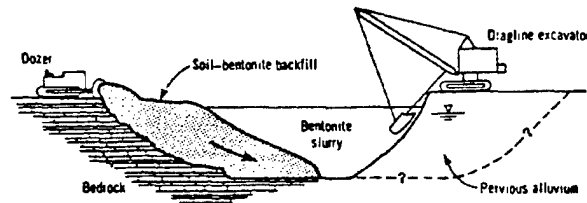
a. Soil bentonite cutoff
