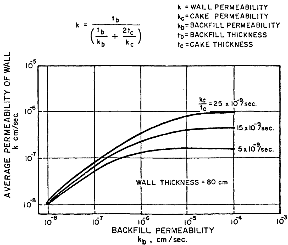
Figure 9-10. Permeability of a soil-bentonite slurry trench cutoff wall 80 cm thick for various values of backfill and filter cake permeability (courtesy of American Society of Civil Engineers 163 )
