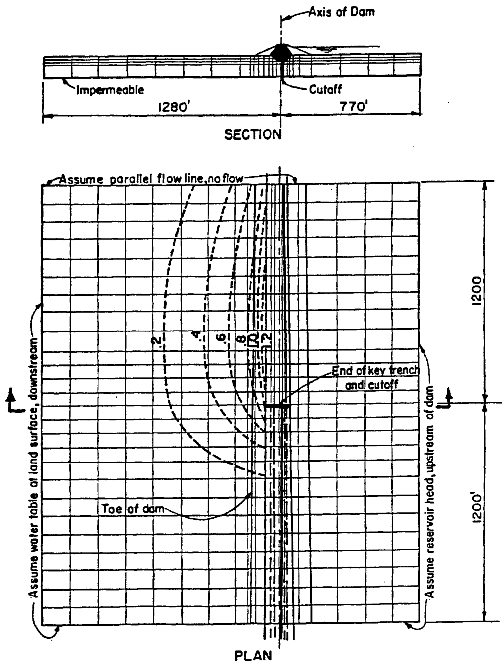
Figure B-24. Contours of exit gradient from three-dimensional finite element model study of Narrows Dam, Colorado (courtesy of American Society of Civil Engineers 217 )
