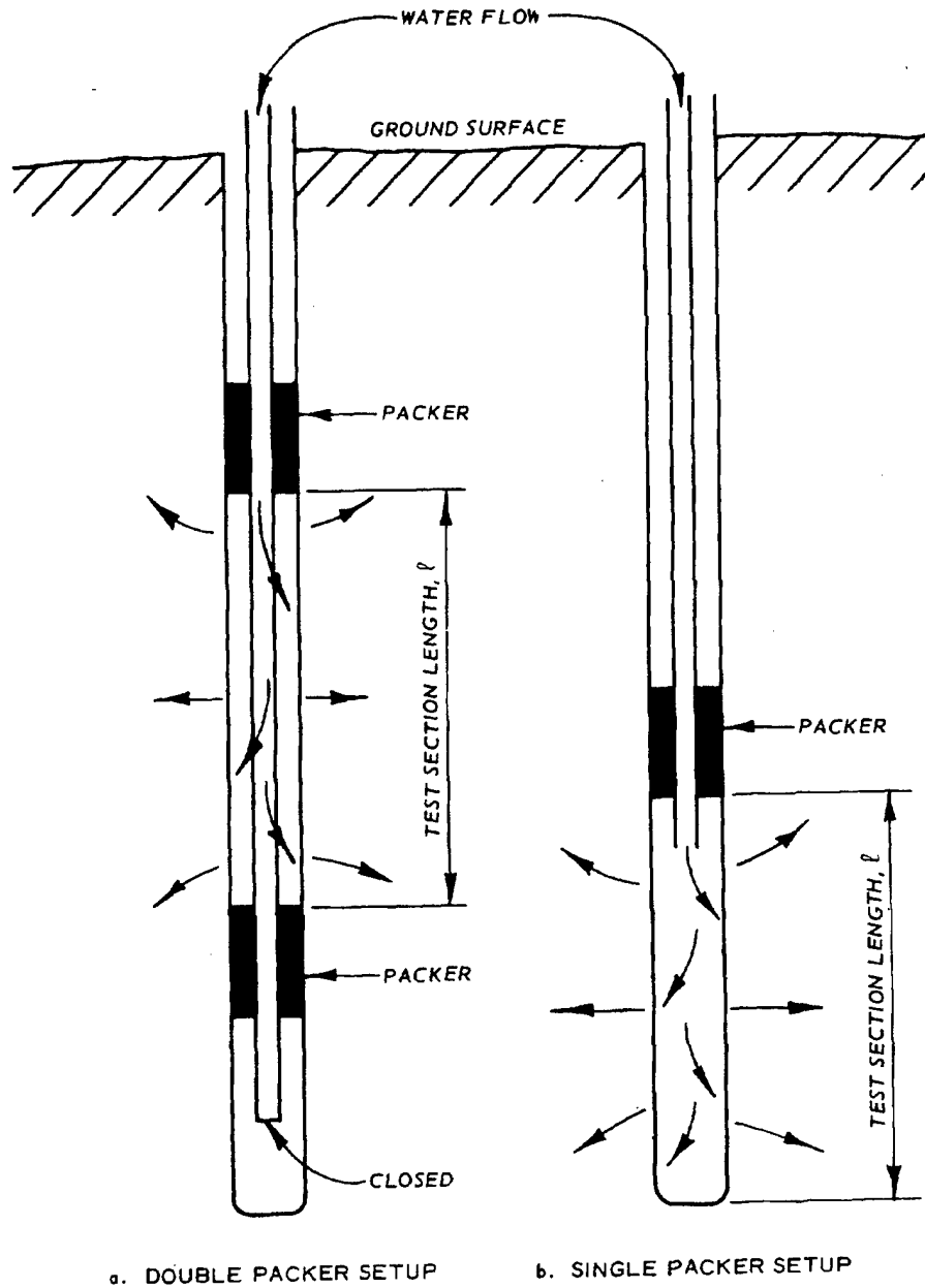
Figure C-1. Typical water pressure test setups (prepared by WES)
