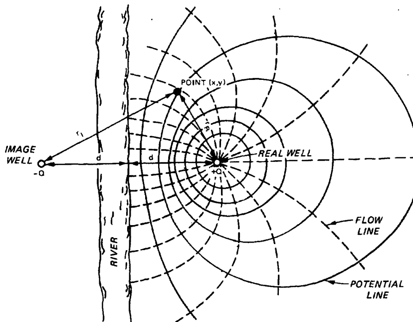
a. IMAGE WELL ANALYSIS OF DISCHARGE WELL NEAR RECHARGE BOUNDARY (RIVER)
