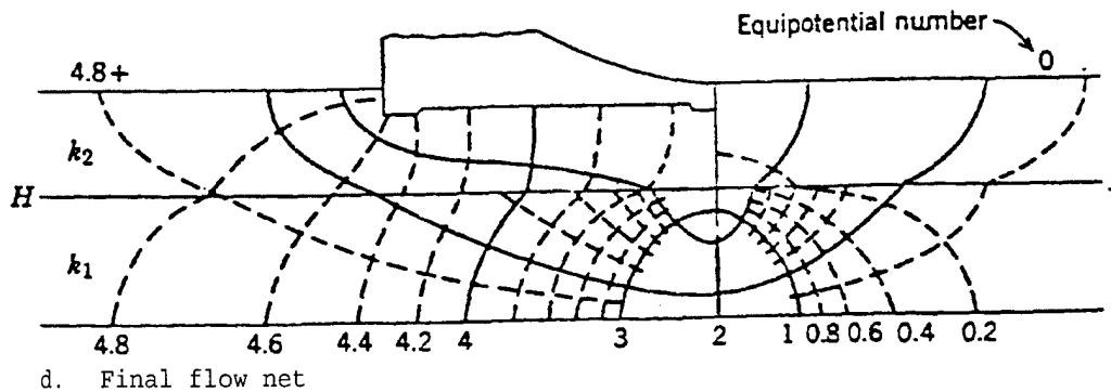
Figure 4-12. Flow net construction for a composite section (courtesy of John Wiley and Sons 155 )
