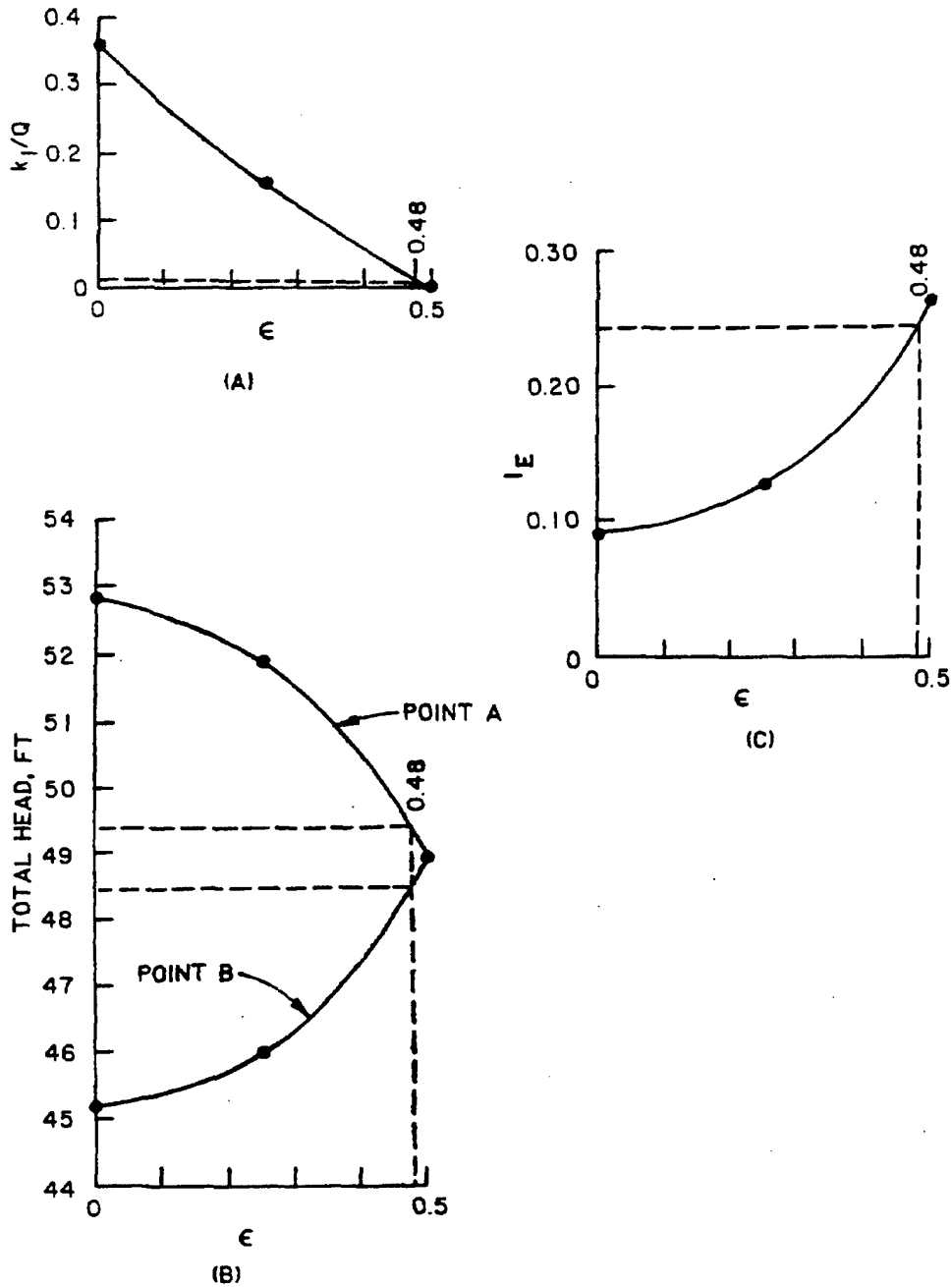
Figure B-20. \epsilon value plots for John H. Overton Dam and stilling basin (from U. S. Army Engineer District, St. Louis 112 )
