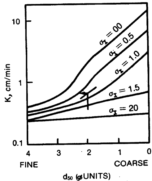
b. Coefficient of permeability versus median grain size
