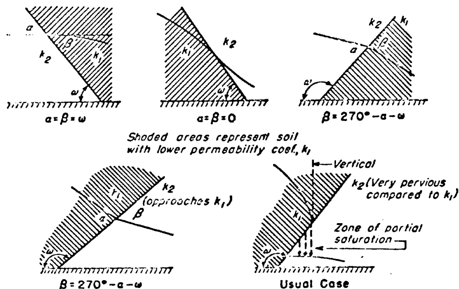
Figure 6-14. Transfer of line of seepage between regions of different permeability (courtesy of New England Waterworks Association 151 )
