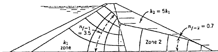
b. Completed flow net (correct)
