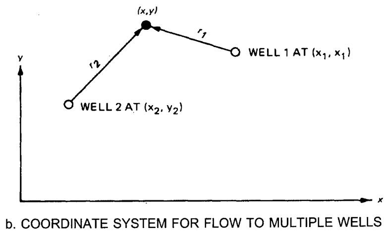
Figure 7-3. Flow to multiple wells (adapted from John Wiley and Sons 164 )
