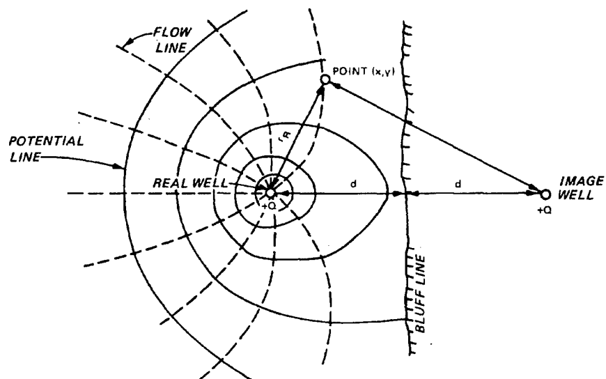
b. IMAGE WELL ANALYSIS OF DISCHARGE WELL NEAR IMPERMEABLE BOUNDARY (ROCK BLUFF)
