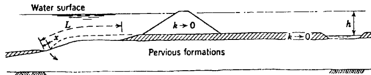
a. Cross section of dam
