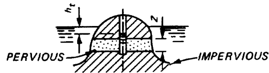
a. HORIZONTAL FLOW TO WELL
