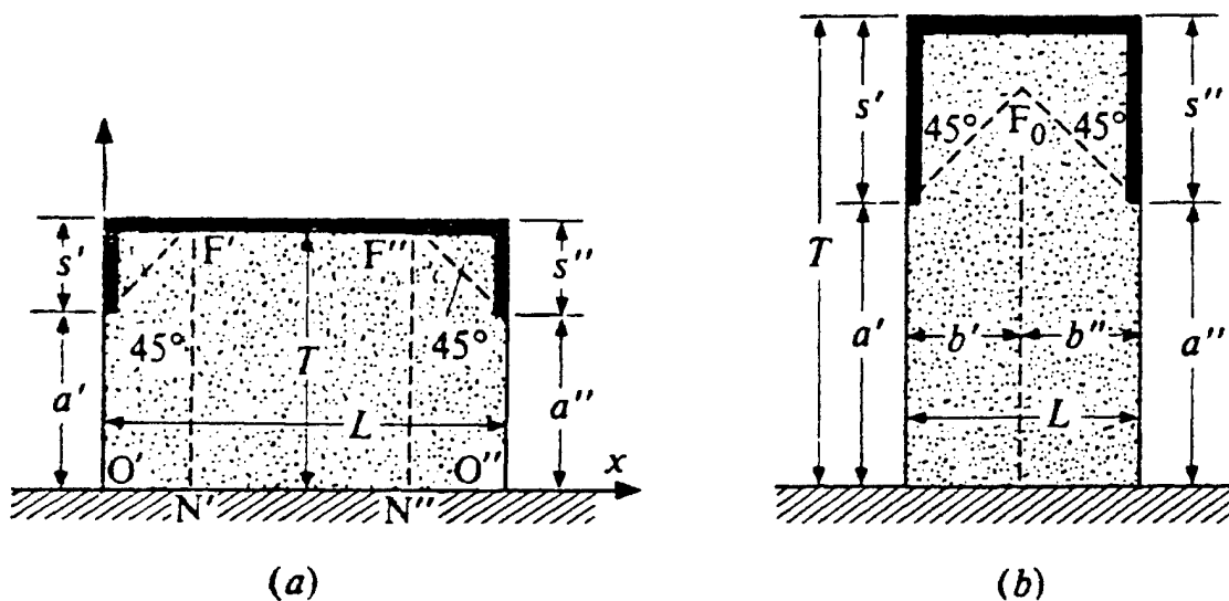
Figure B-11. Type VI fragment (courtesy of McGraw-Hill Book Company 181 )
