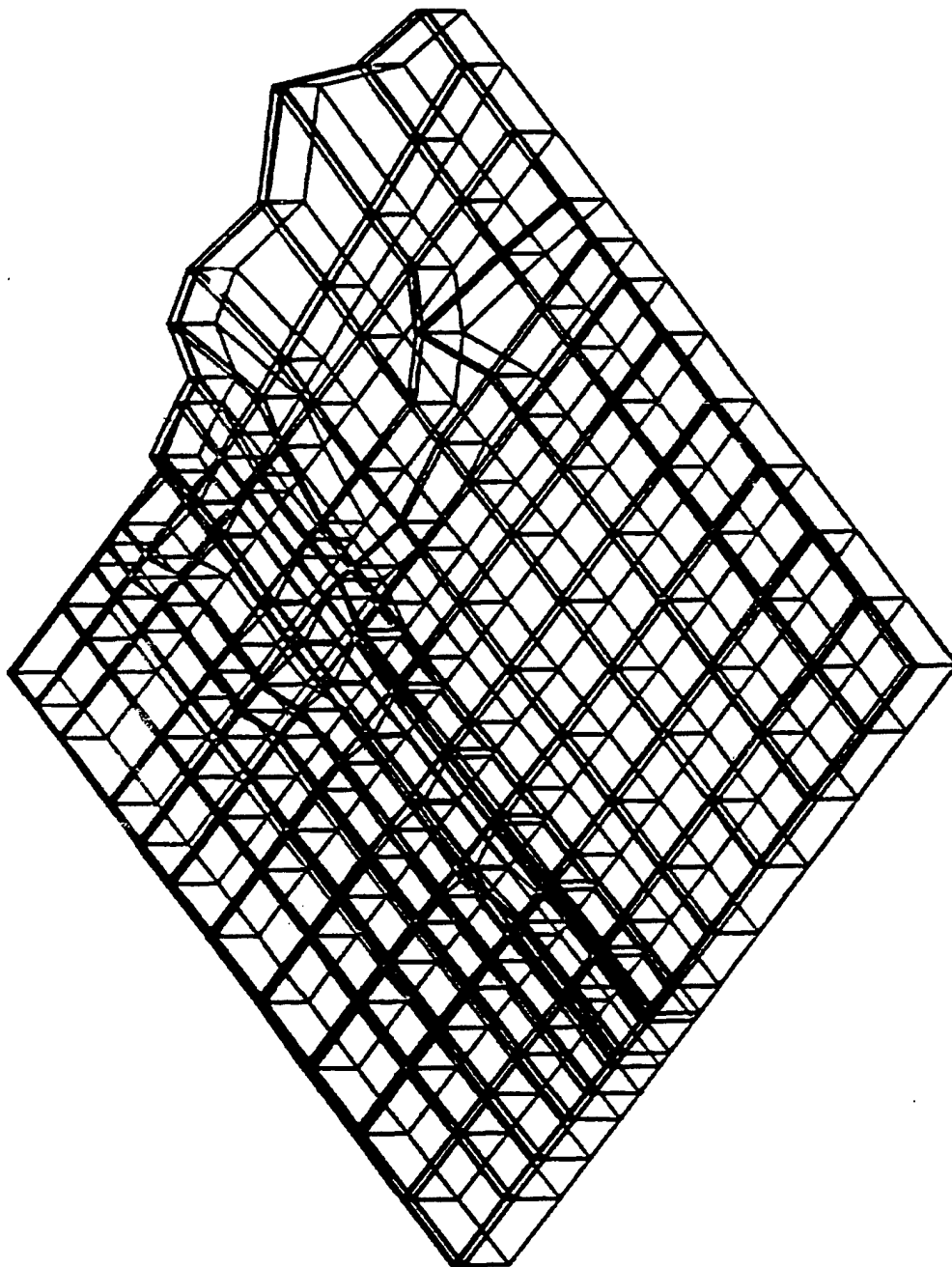
Figure B-26. Grid for three-dimensional finite element model study of Calamus Dam, Nebraska (courtesy of American Society of Civil Engineers 217 )
