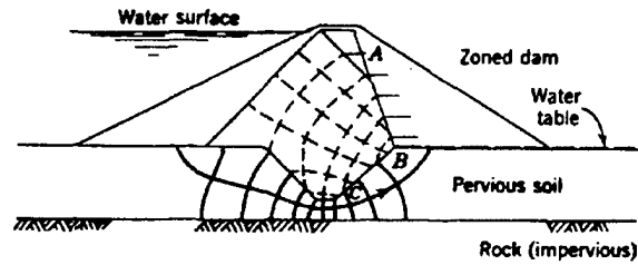
a. Partial cutoff
