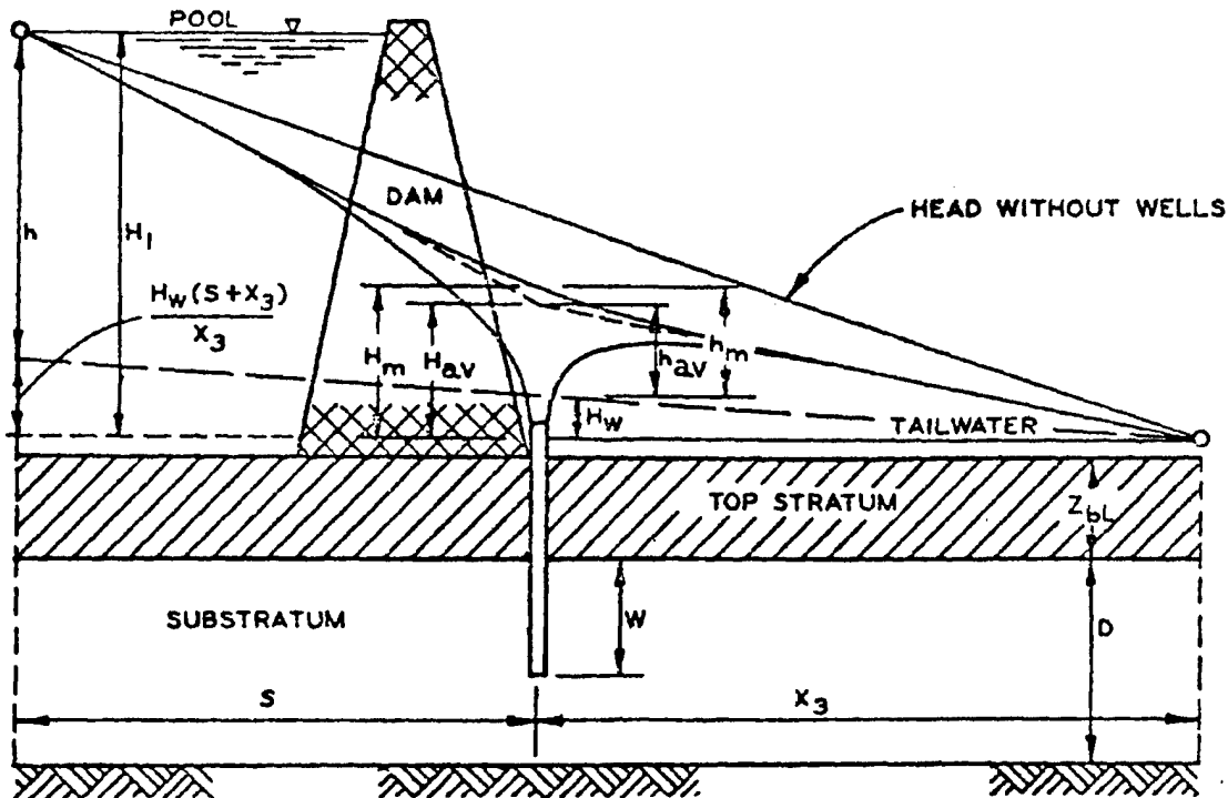
Figure 9-25. Design of relief wells (prepared by WES)
