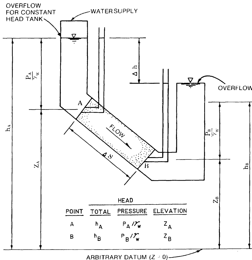
Figure 2-1. Darcy's law for flow through inclined soil column (prepared by WES)
