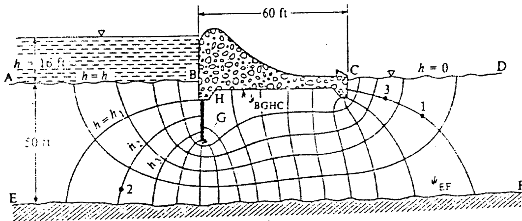
Figure 5-2. Gravity dam on pervious foundation of finite depth (courtesy of McGraw-Hill Book Company 181 )
