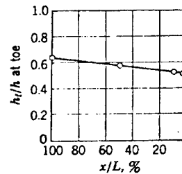
d. Uplift at toe
