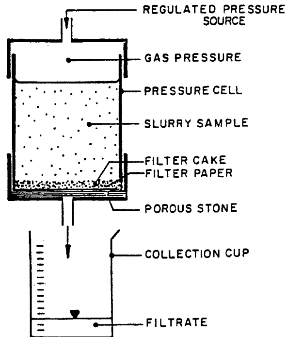
a. Schematic of filter press test apparatus
