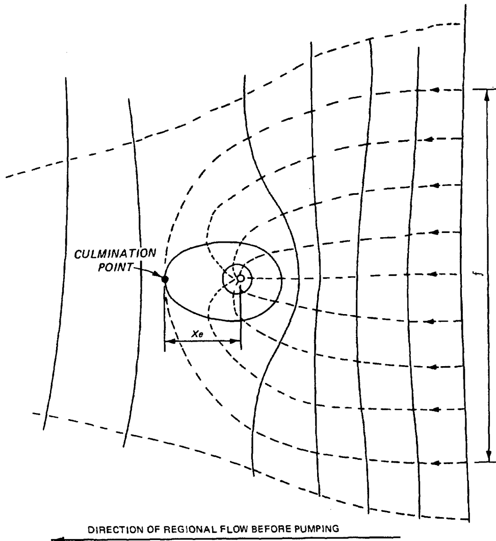
Figure 7-7. Superposition of well drawdown on regional gradient (courtesy of International Institute for Land Reclamation and Improvement 199 )
