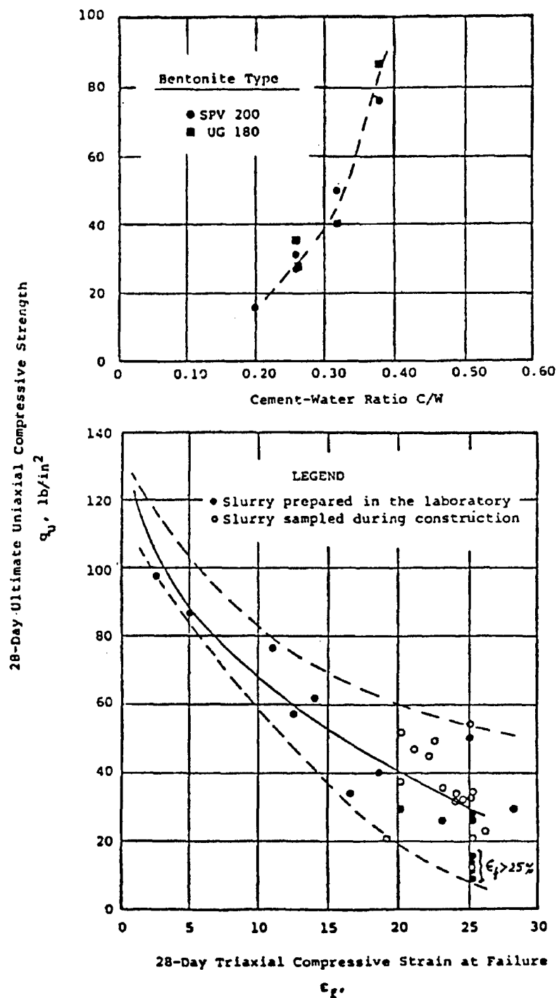
Figure 9-12. Strength and deformation characteristics of cement-bentonite slurries (courtesy of American Society of Engineers 223 )
