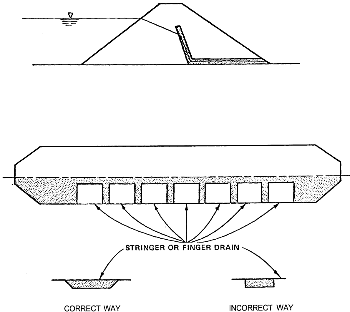
Figure 8-11. Use of stringers or finger drains as an alternative to a continuous horizontal drain (prepared by WES)
