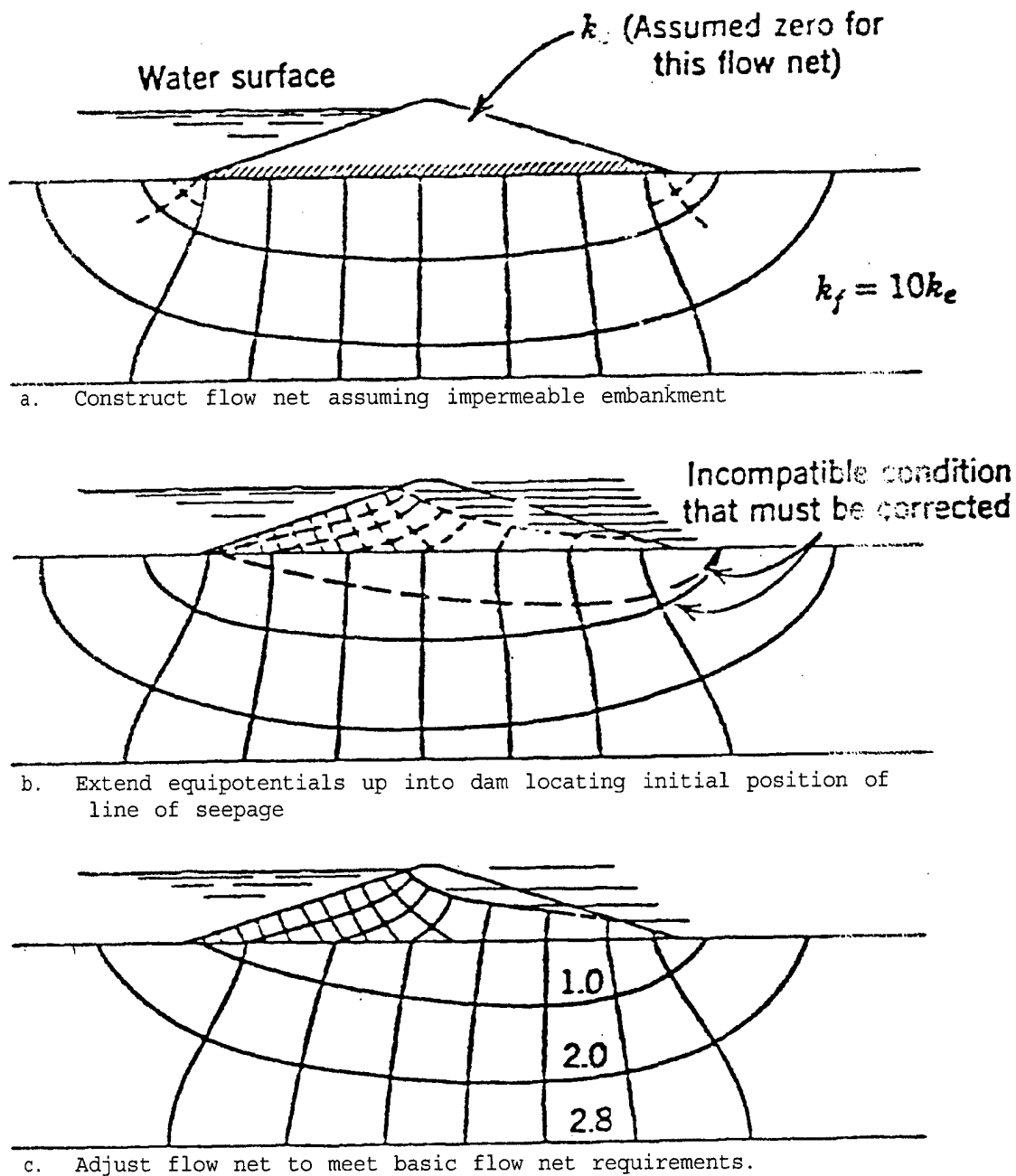
Figure 4-14. Flow net construction for an embankment on a foundation of higher permeability (courtesy of John Wiley and Sons 155 )
