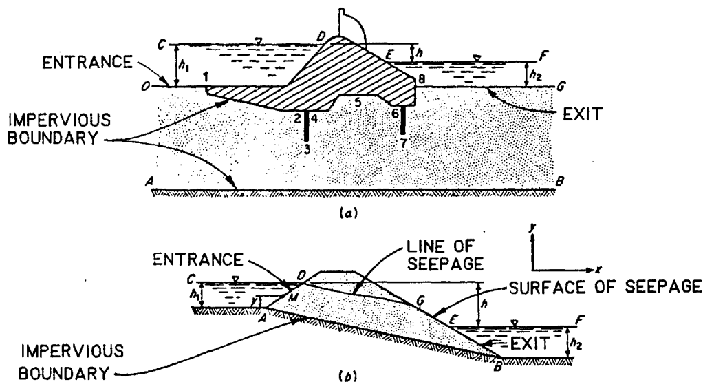
Figure 4-1. Examples of boundary conditions (courtesy of McGraw-Hill Book Company 180 )
