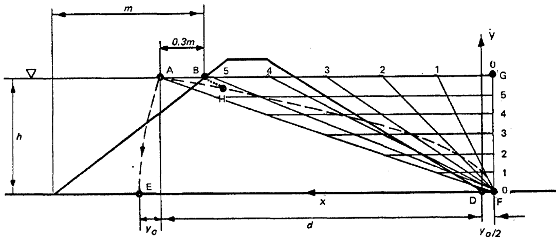
Figure 6-3. Construction of basic parabola (prepared by WES)
