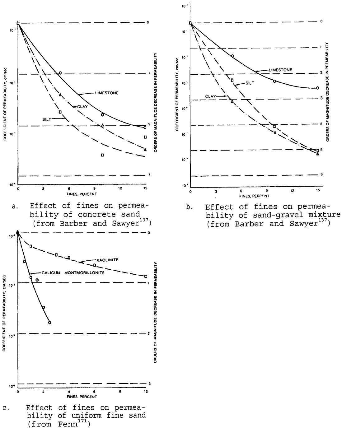
Figure 2-12. Influence of type and amount of fines on permeability of concrete sand, sand-gravel mixture, and uniform fine sand (prepared by WES)
