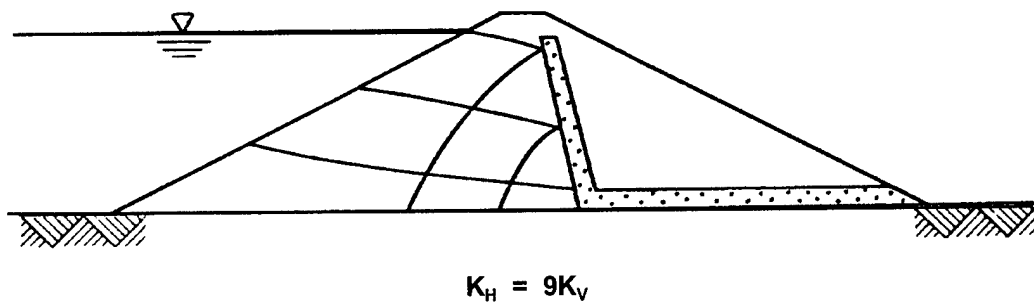
Figure 8-8. Effect of anisotropy of permeability on seepage through earth dam with and without an inclined drain (courtesy of John Wiley and Sons 155 )
