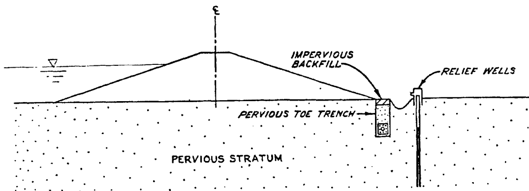
c. Trench drain used in conjunction with relief wells
