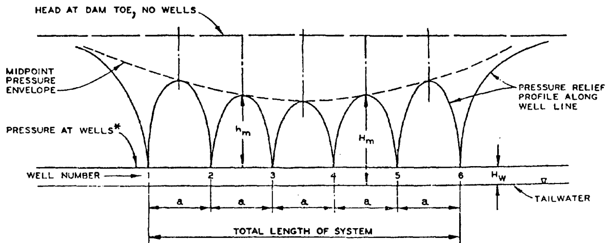
Figure 9-30. Variation of pressure relief along a finite line of relief wells (after EM 1110-2-1905)
