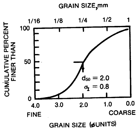
a. Grain size distribution
