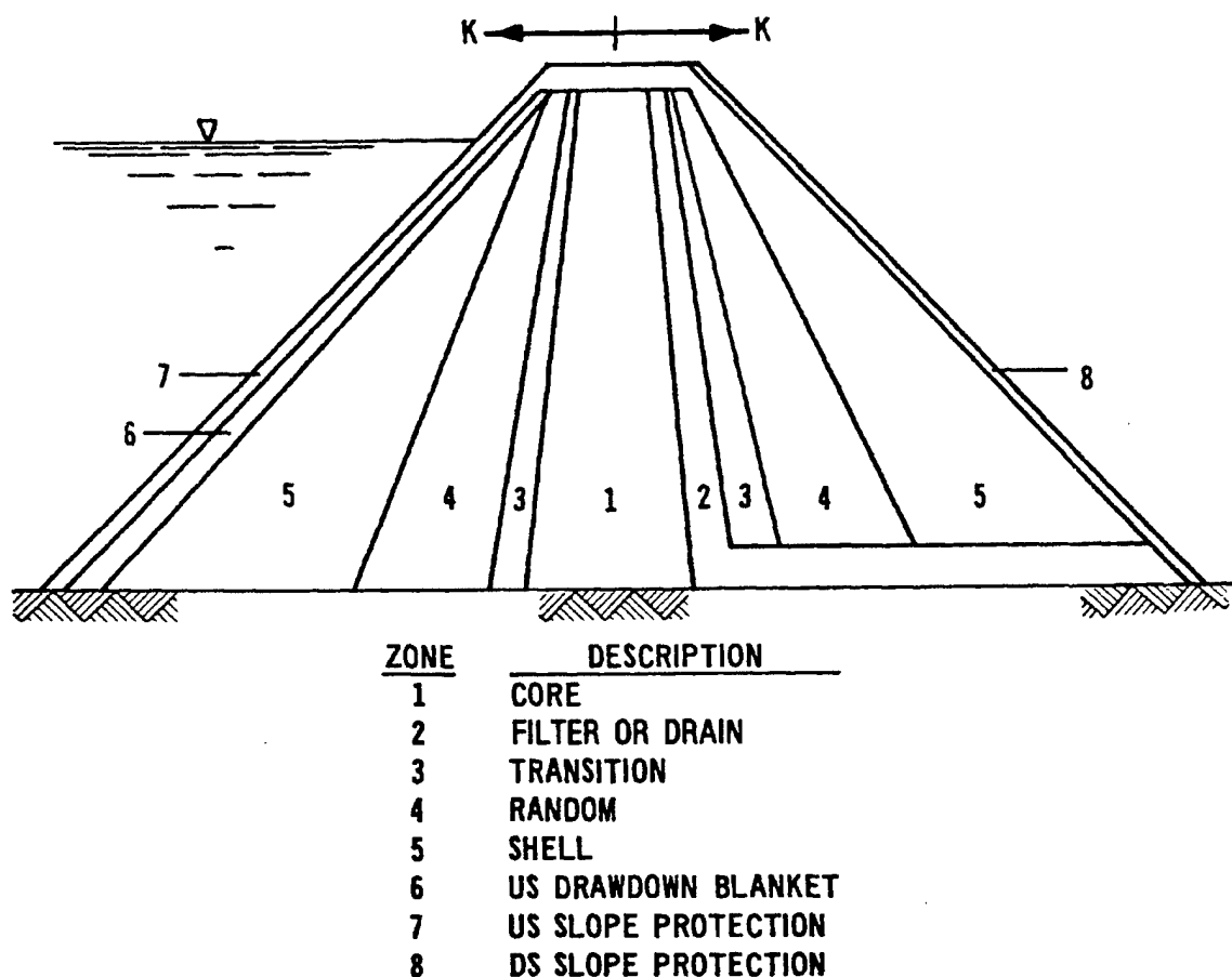
Figure 8-2. Different zones of an embankment (prepared by WES)
