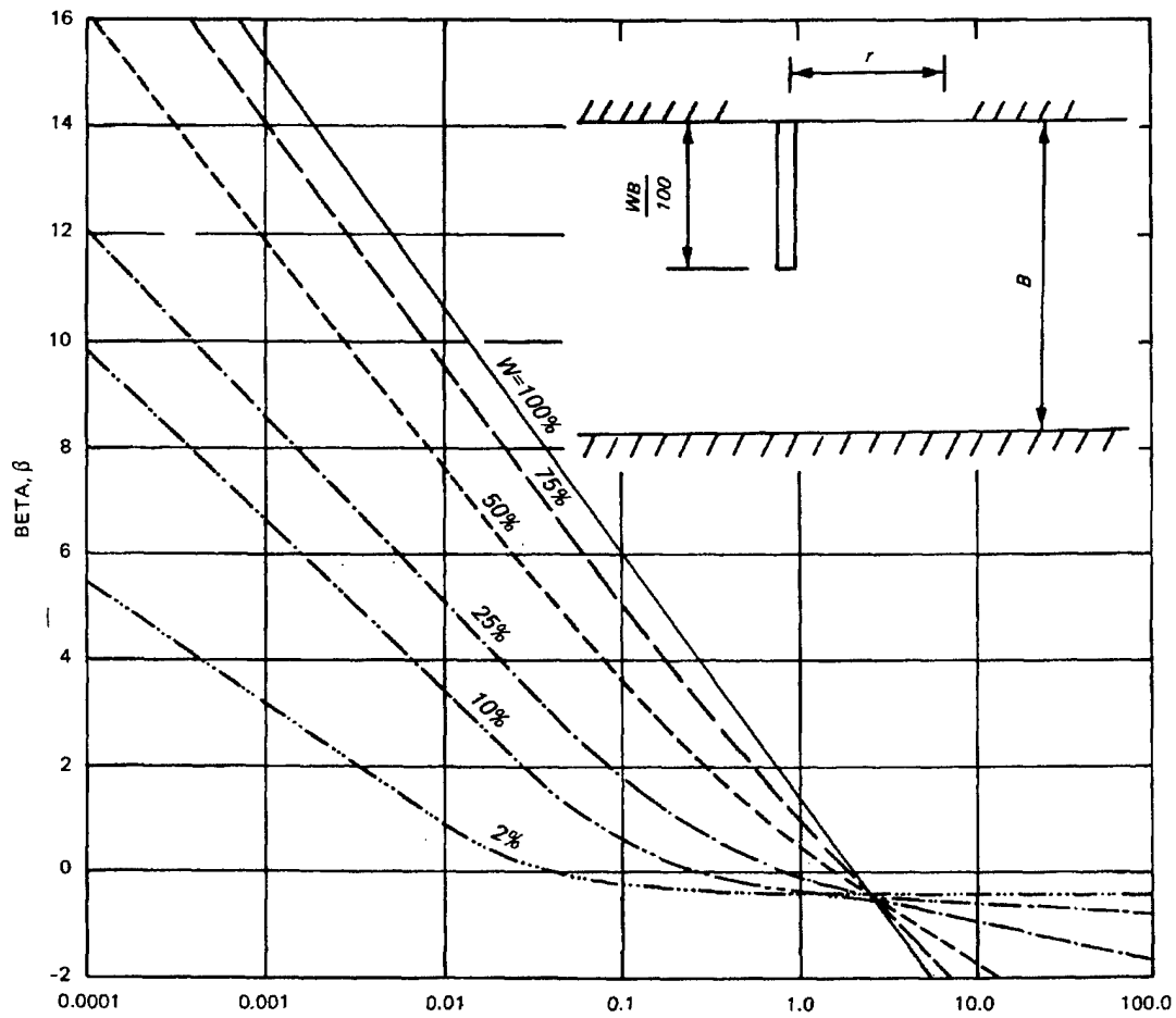
Figure 7-6. Beta function curve (from Warriner and Banks 124 )
