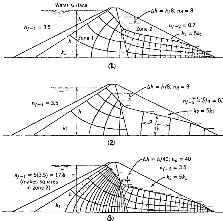
Figure 6-16. Three forms of one flow net (courtesy of John Wiley and Sons 155)
