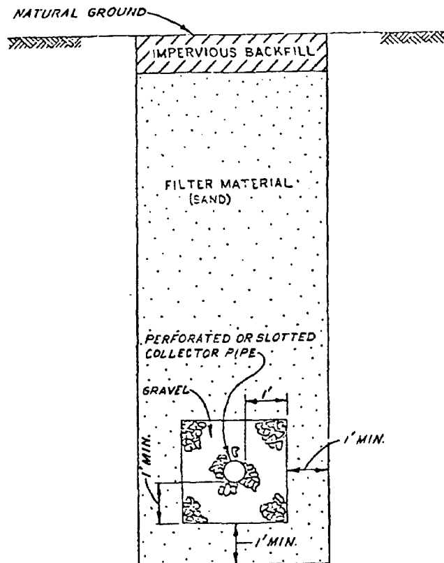
Figure 9-34. Trench drain with collector pipe (from EM 1110-2-1913)
