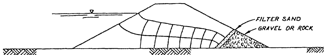
Figure 6-11. Homogeneous embankment on impervious foundation with a toe drain (from EM 1110-2-1913 11 )
