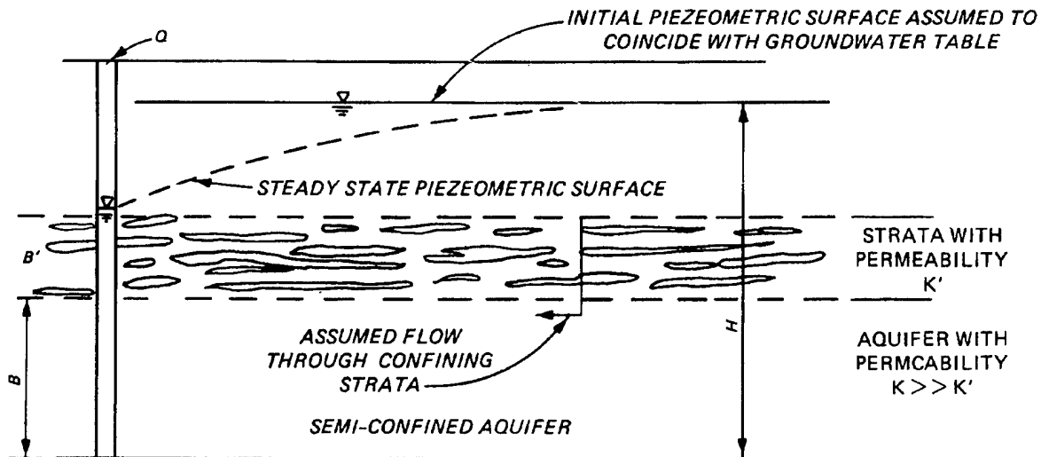
Figure 7-8. Flow to well with significant vertical flow through confining layer (courtesy of John Wiley and Sons 164 )
