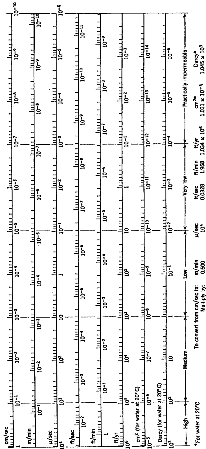
Figure 2-4. Permeability conversion chart (courtesy of John Wiley &amp; Sons, Inc. 201)
