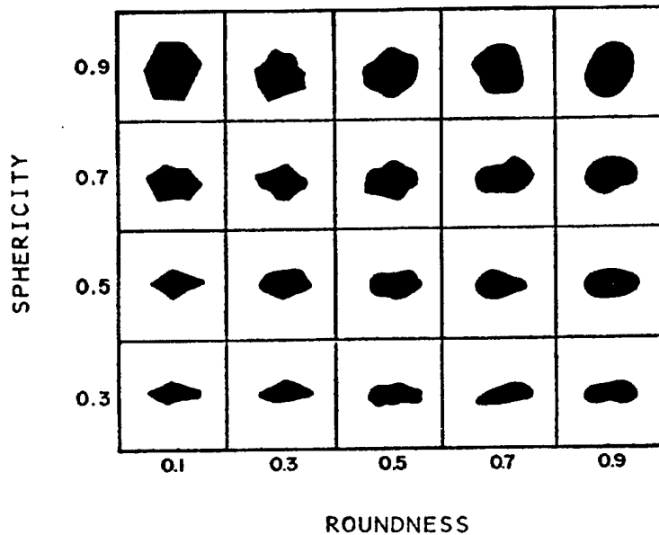
Figure 2-10. Krumbein and Sloss standard chart for visual estimation of sphericity and roundness of cohesionless soils (courtesy of W. H. Freeman and Company 198 )
