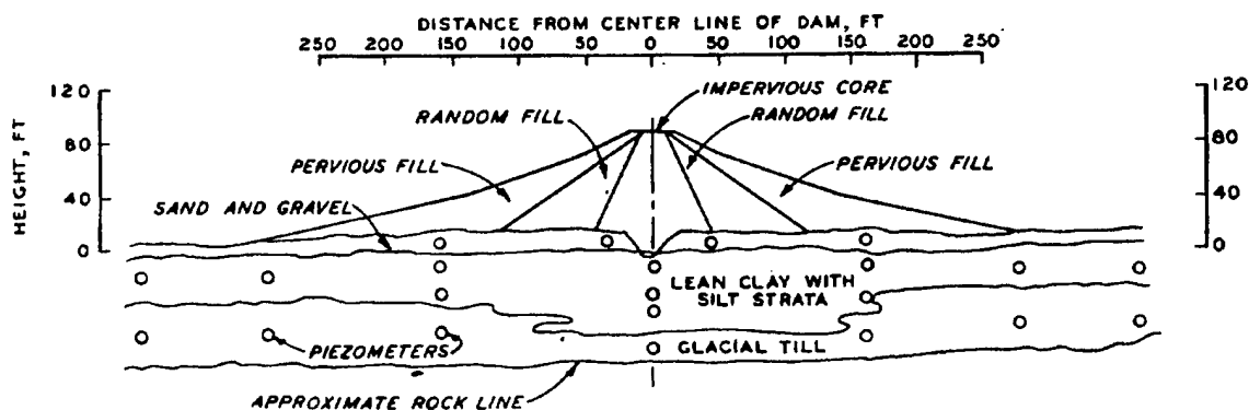
Figure 13-1. Example of foundation piezometer installation of Surry Mountain Dam (from EM 1110-2-1908)
