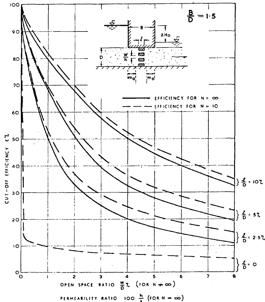
Figure 9-18. Cutoff efficiency versus open space ratio for imperfect cutoffs (courtesy of Butterworths, Inc. 129 )
