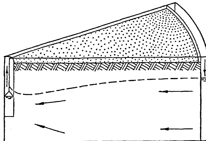
PARTIALLY PENETRATING WELL WITH A CIRCULAR SOURCE
