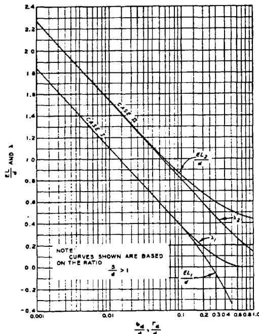
Figure 9-33. Design of toe trench drains for homogeneous, isotropic, pervious foundation, and for an impervious downstream top stratum 120 (from U. S. Army Engineer Waterways Experiment Station)
