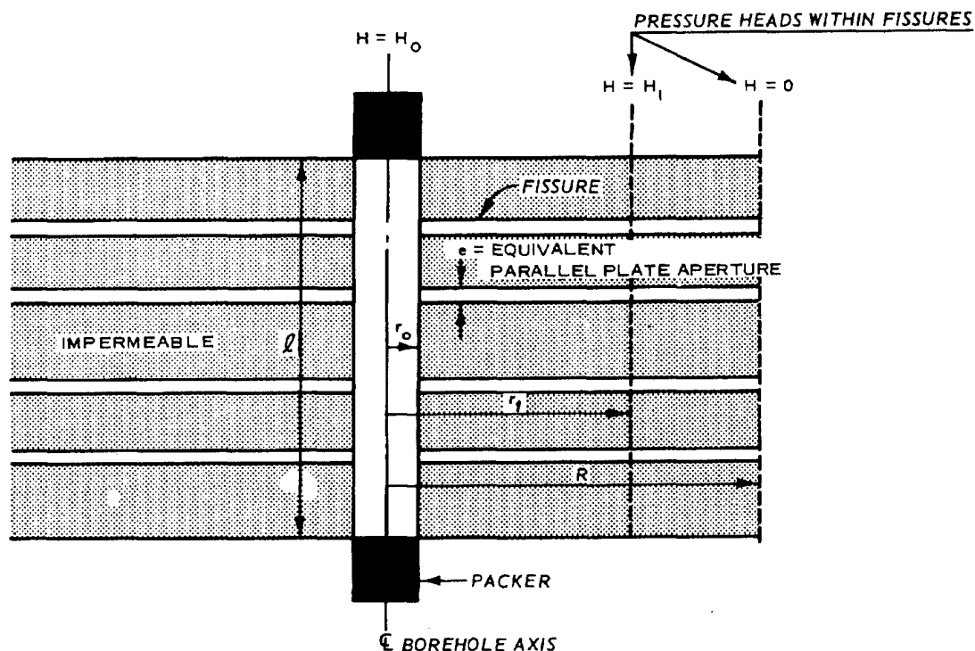
Figure C-3. Fissured-medium--radial flow (prepared by WES)
