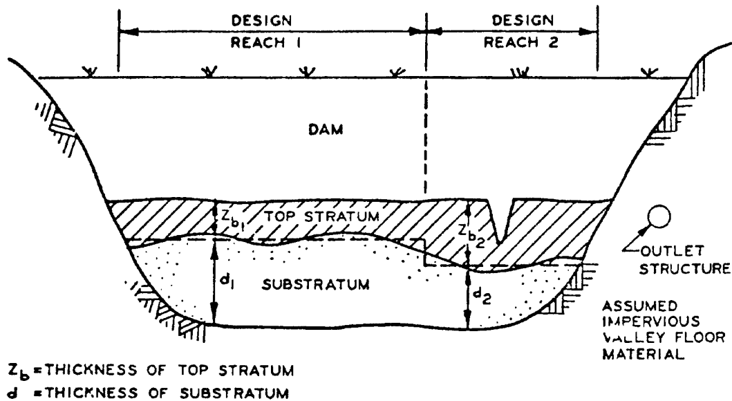
Figure 9-24. Profile of typical design reaches for relief well analysis (prepared by WES)
