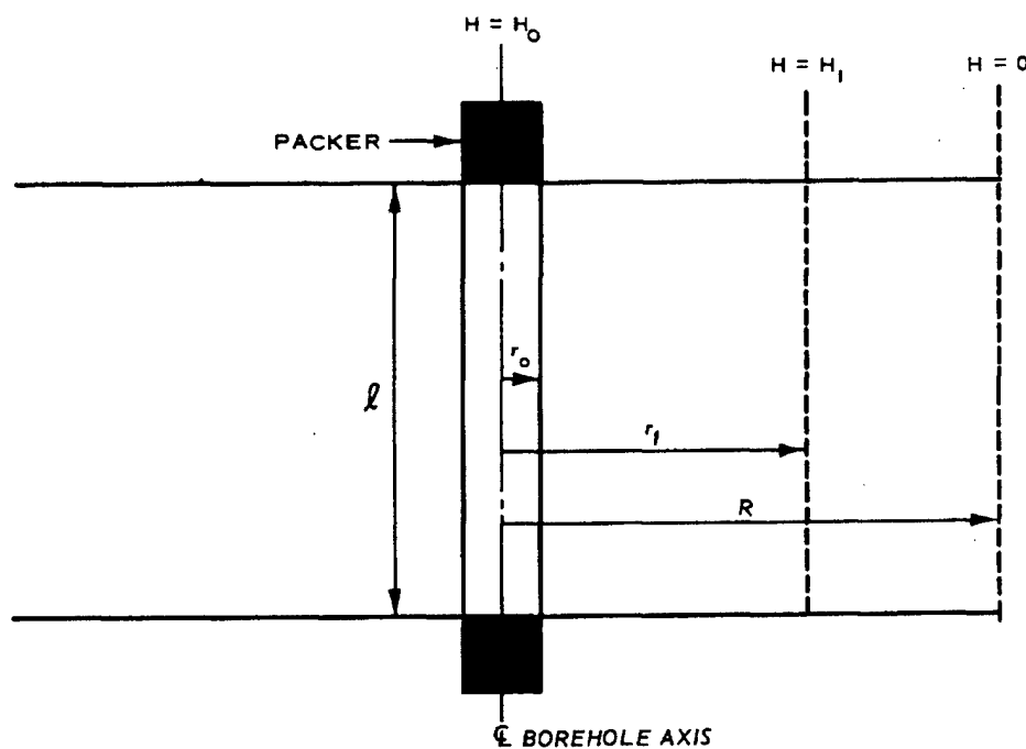
Figure C-2. Homogeneous isotropic material--radial flow (prepared by WES)
