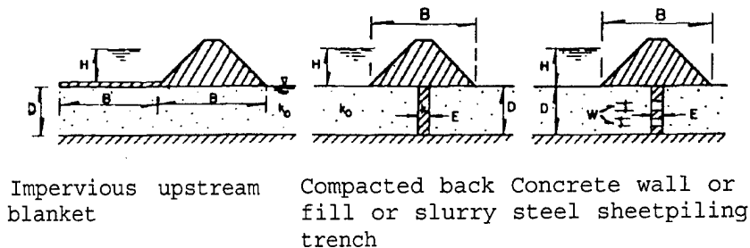
Figure 9-5. Rate of underseepage loss for impervious upstream blanket, compacted backfill trench or slurry trench, and concrete wall or steel sheetpiling with defects (courtesy of American Society of Civil
