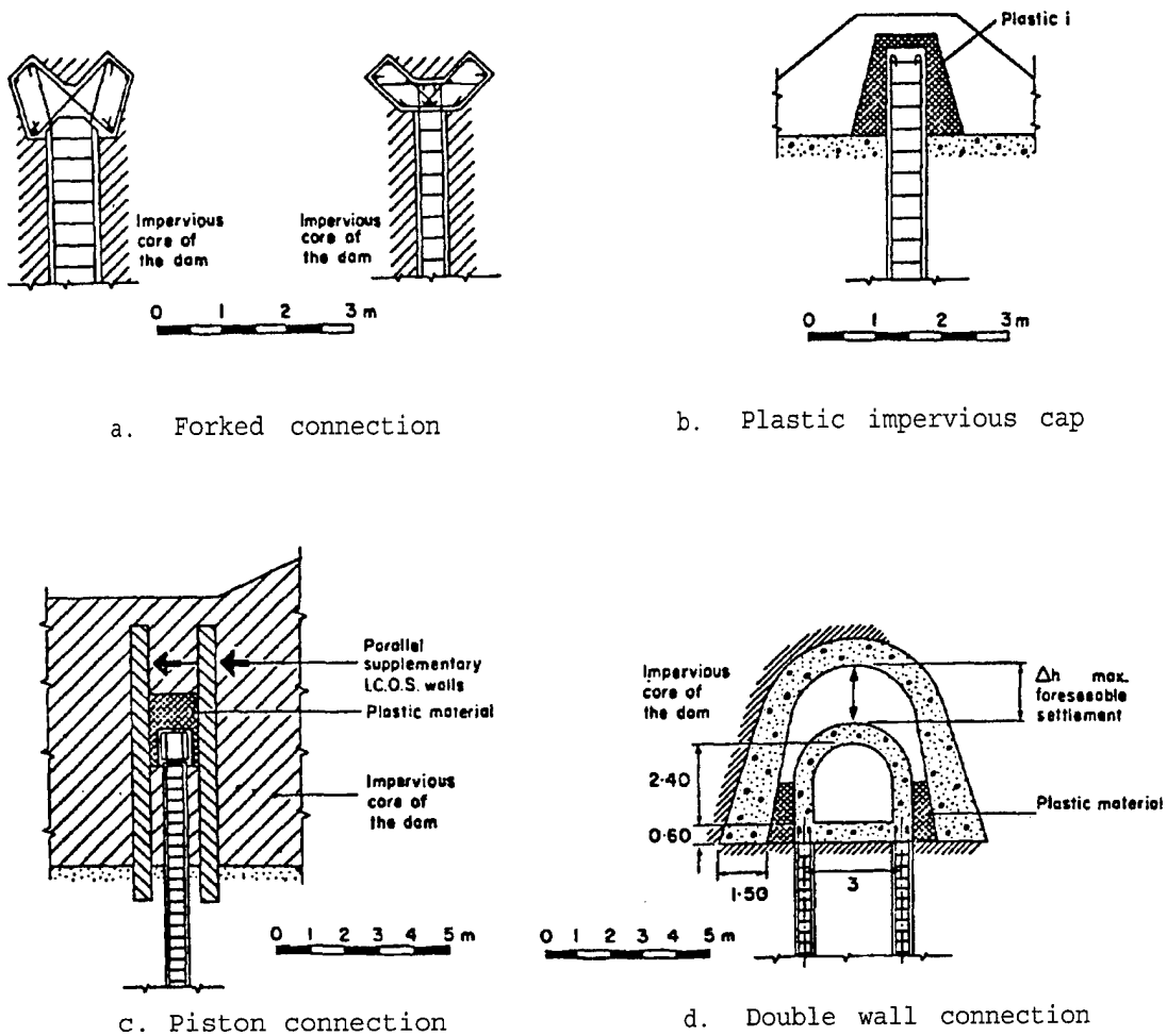
Figure 9-15. Connections between concrete cutoff wall and core of dam (courtesy of ICOS 182 )
