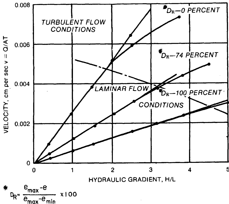
Figure 2-8. Determination of maximum hydraulic gradient for which laminar flow occurs for a fine sand (courtesy of American Society for Testing and Materials 147 )
