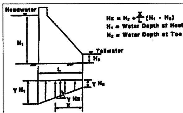
Figure 3-1. Uplift distribution without foundation drainage
