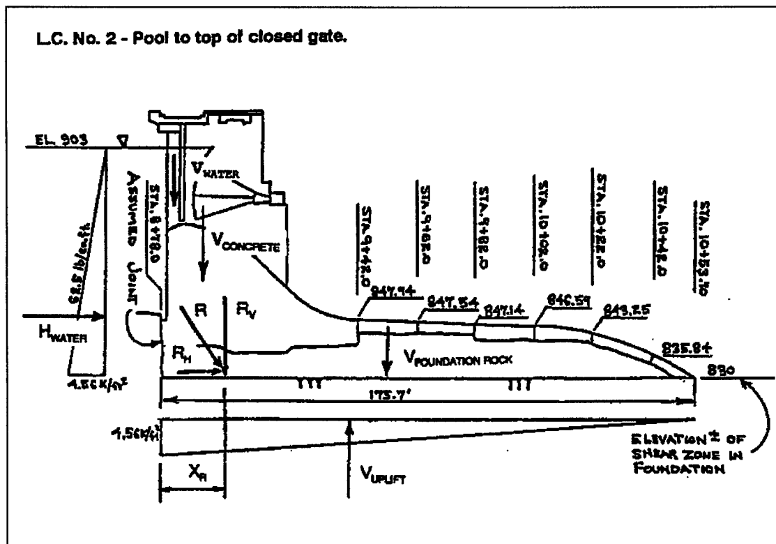
Figure 8-2. Free body diagram, R_v = resultant of vertical forces, R_h = resultant of horizontal forces, and X_R = distance from heel to resultant location on sliding plane
