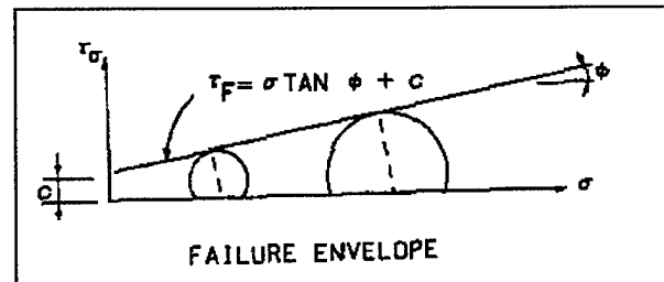
Figure 4-3. Failure envelope
