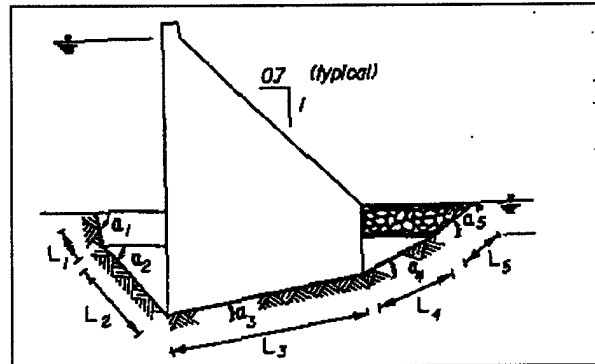
Figure 4-4. Geometry of structure foundation system
