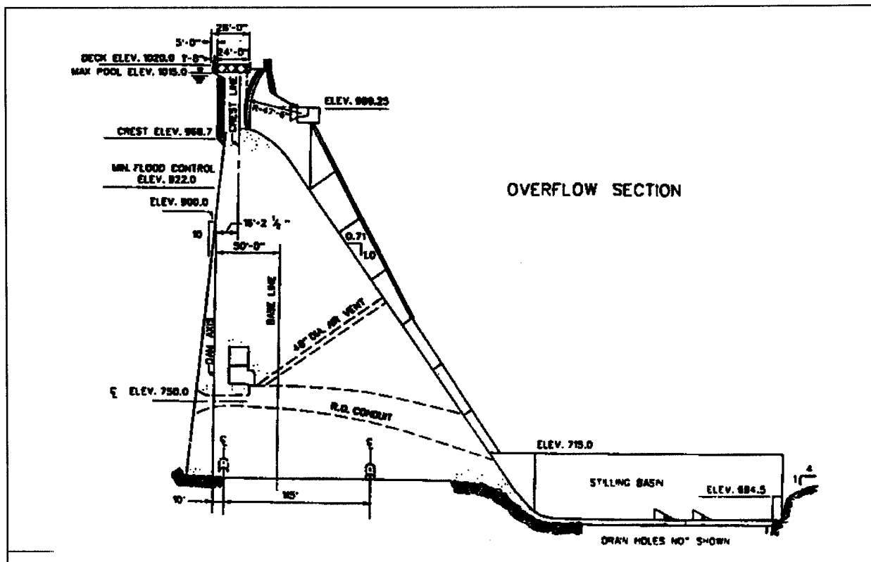
Figure 2-1. Typical dam overflow section
