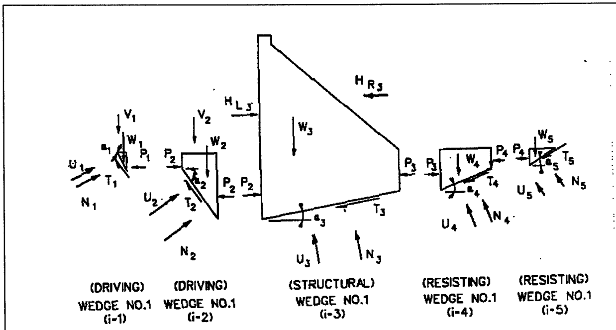
Figure 4-5. Dam foundation system, showing driving, structural, and resisting wedges
