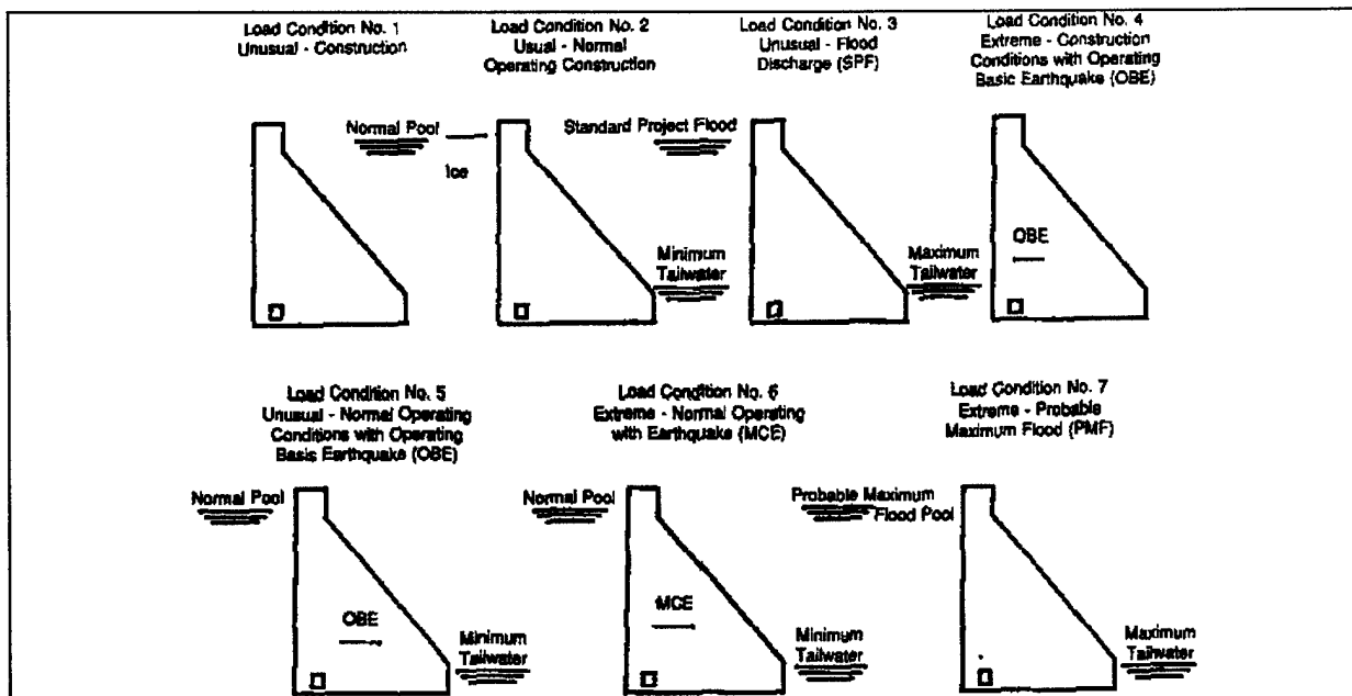
Figure 4-1. Basic loading conditions in concrete gravity dam design
