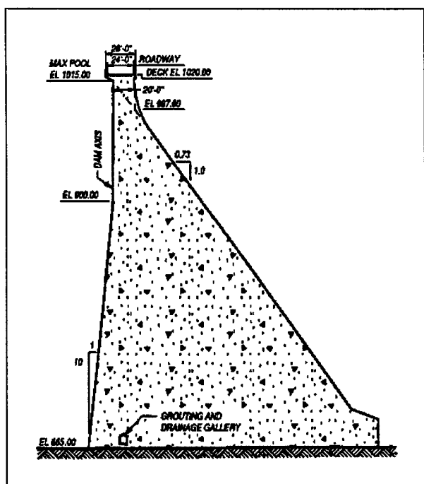
Figure 2-2. Nonoverflow section
