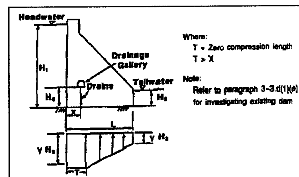
Figure 3-5. Uplift distribution cracked base with drainage, zero compression zone extending beyond drains
