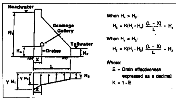
Figure 3-2. Uplift distribution with drainage gallery
