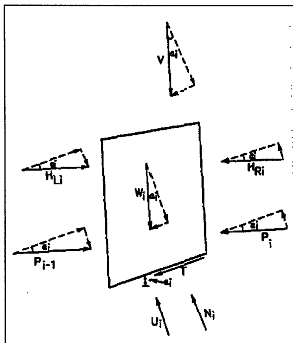
Figure C-4. Free body diagram of the i th wedge
