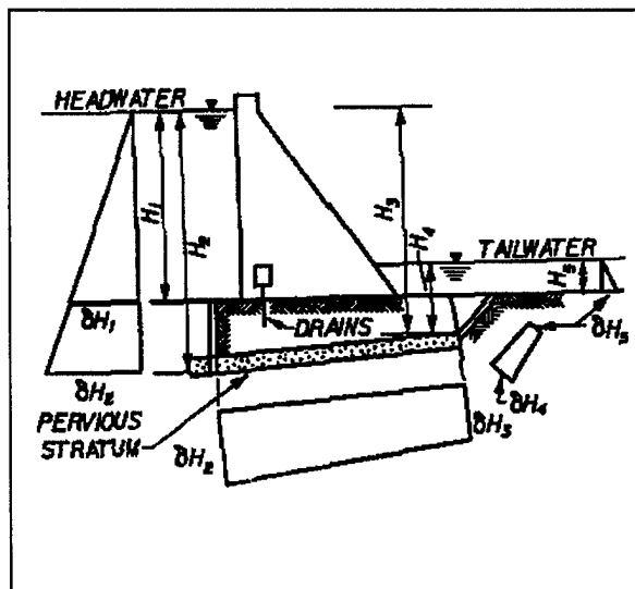
Figure 3-9. Effect along foundation seams or faults if material is pervious and pervious zone is intercepted by base of dam or by impervious fault
