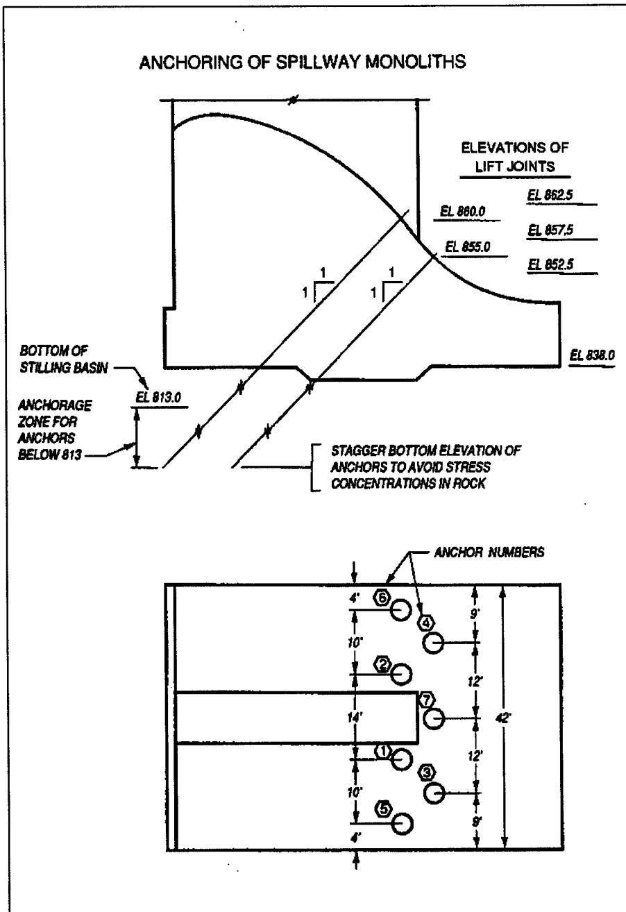
Figure 8-3. Location of anchors
