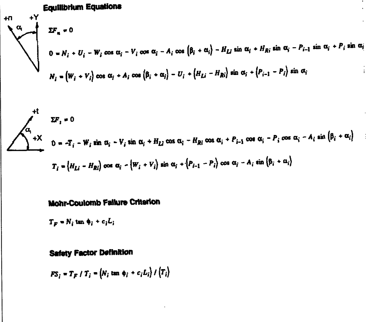
Figure C-7. Derivation of the general equation for a wedge containing an anchor force (Sheet 1 of 3)
