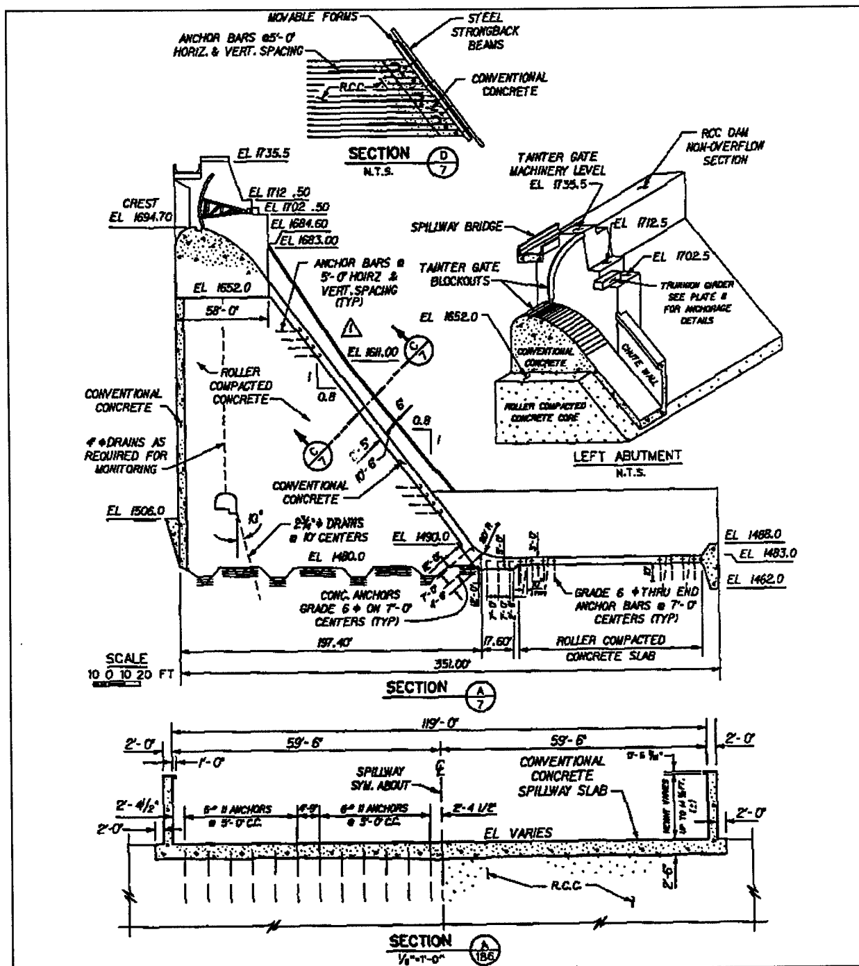
Figure 9-6. RCC spillway details
