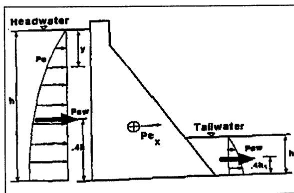
Figure 3-10. Seismically loaded gravity dam, nonoverflow monolith
