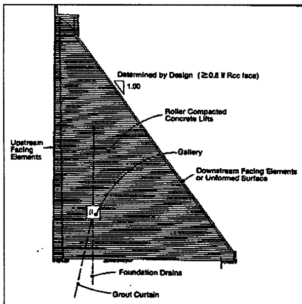
Figure 9-1. Typical RCC dam section
