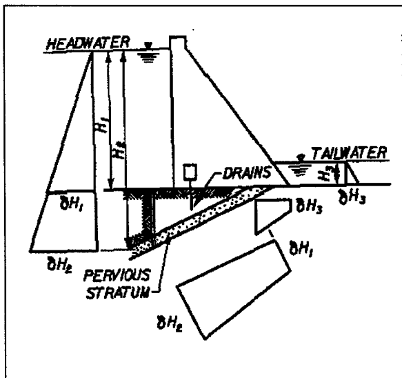
Figure 3-8. Development of dangerous uplift pressure along foundation seams or faults
