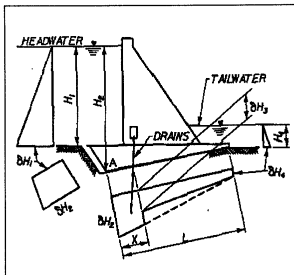
Figure 3-6. Uplift pressure diagram. Dashed line represents uplift distribution to be considered for stability computations
