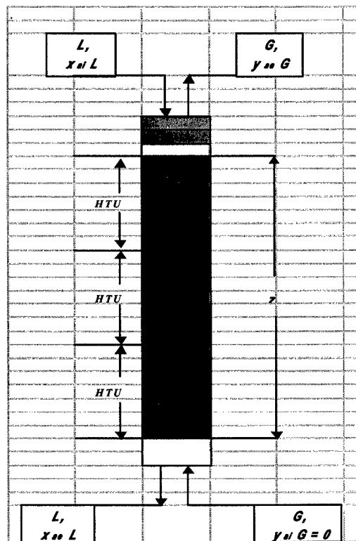
Figure D-1. Random "dumped" packed tower.
