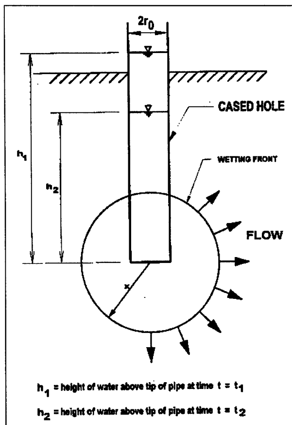
Figure 11-4. Falling-head standpipe percolation test after Schmid (1967)
