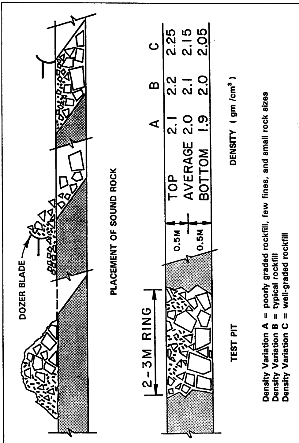
Figure 10-2. Placement of sound rockfill and resulting density variation (after Cooke 1980)
