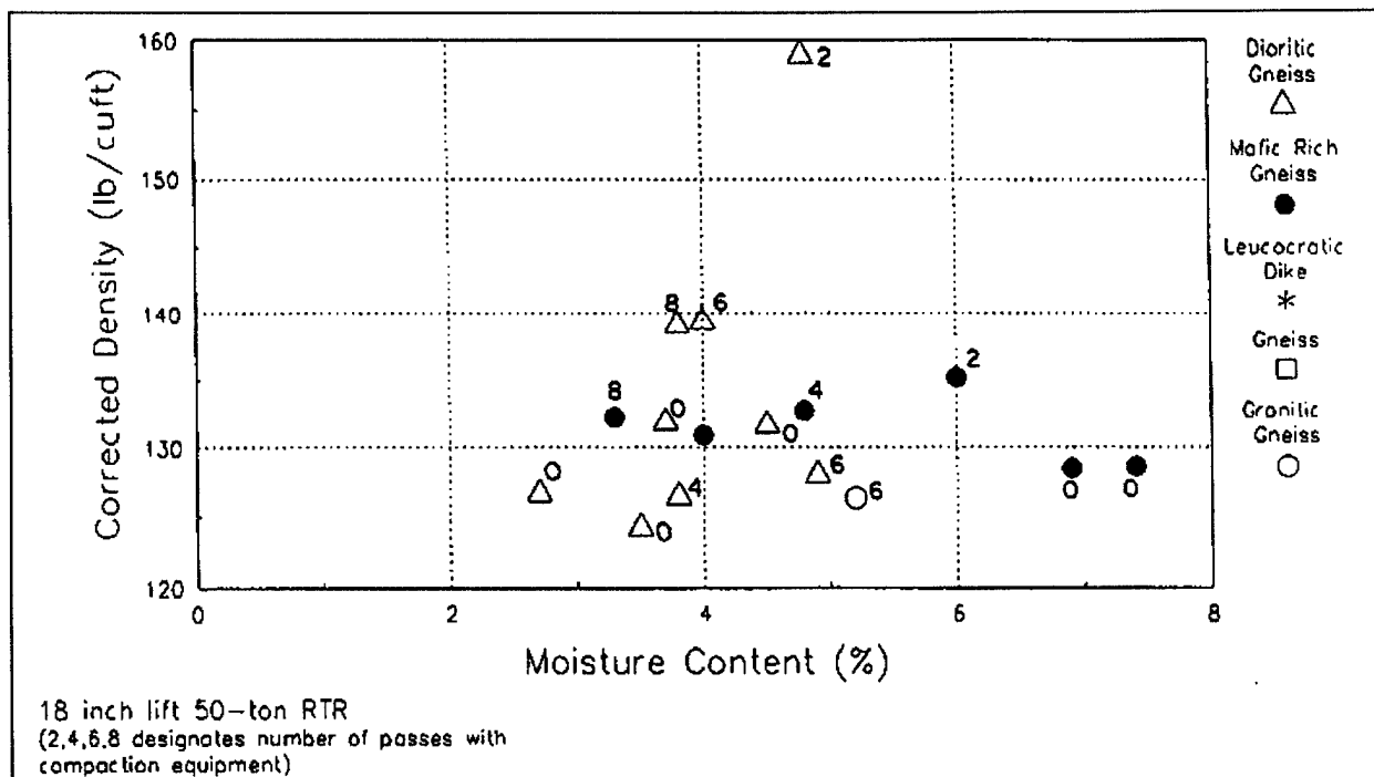
Figure 12-18. Corrected in situ densities, 45.7-cm (18-in.) lift, 45.4-metric ton (50-ton) rubber-tired roller, Seven Oaks Dam materials
