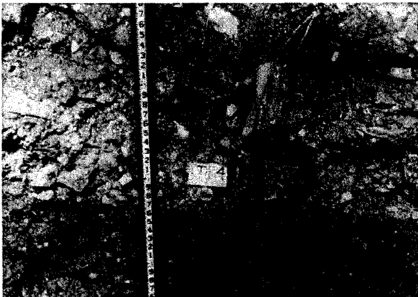
Figure 12-21. Photographs of rockfill containing appreciable fines, Cerrillos Dam test fill No. 4 inspection trench
