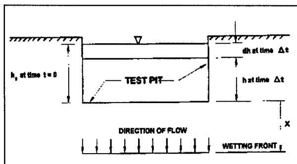
Figure 11-3. Open-pit percolation test after Justo (1991)
