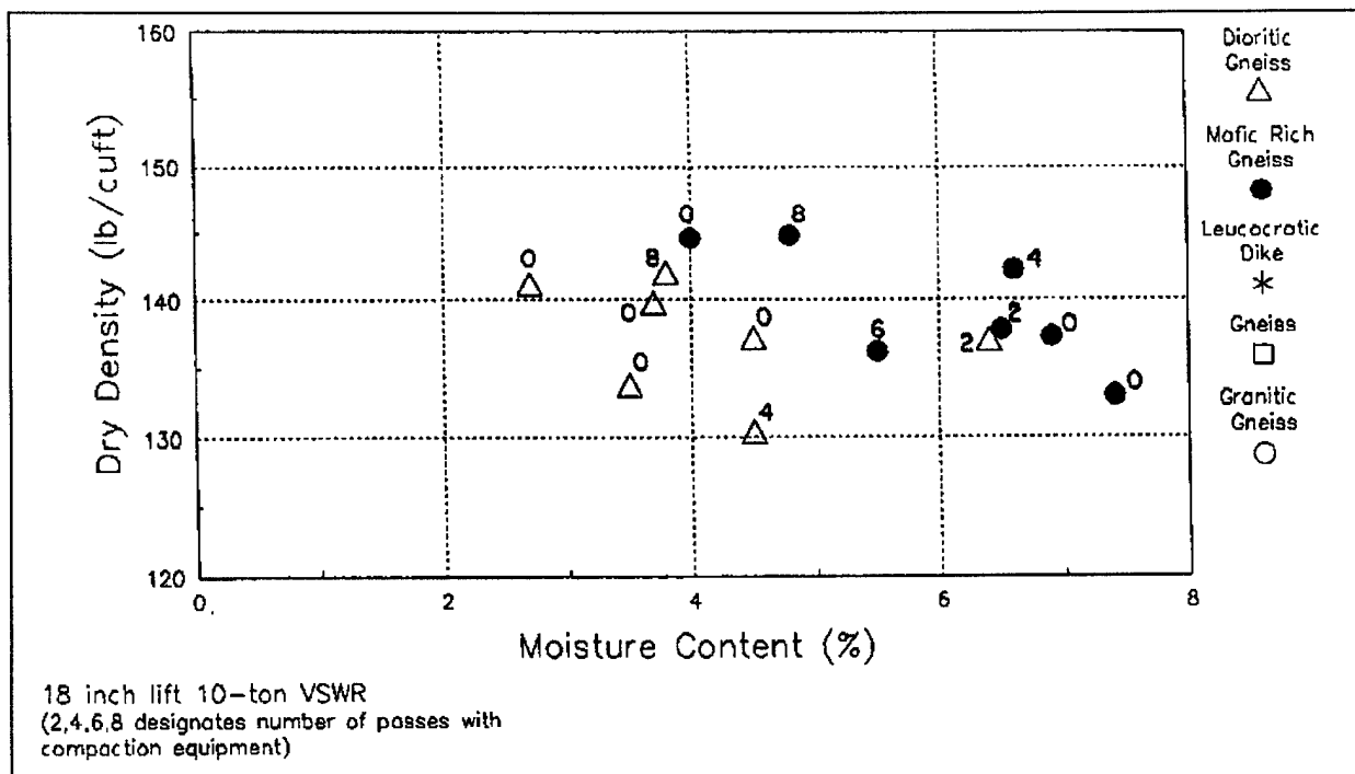
Figure 12-13. In situ density tests, 45.7-cm (18-in.) lift, 9.1-metric ton (10-ton) vibratory roller, Seven Oaks Dam materials
