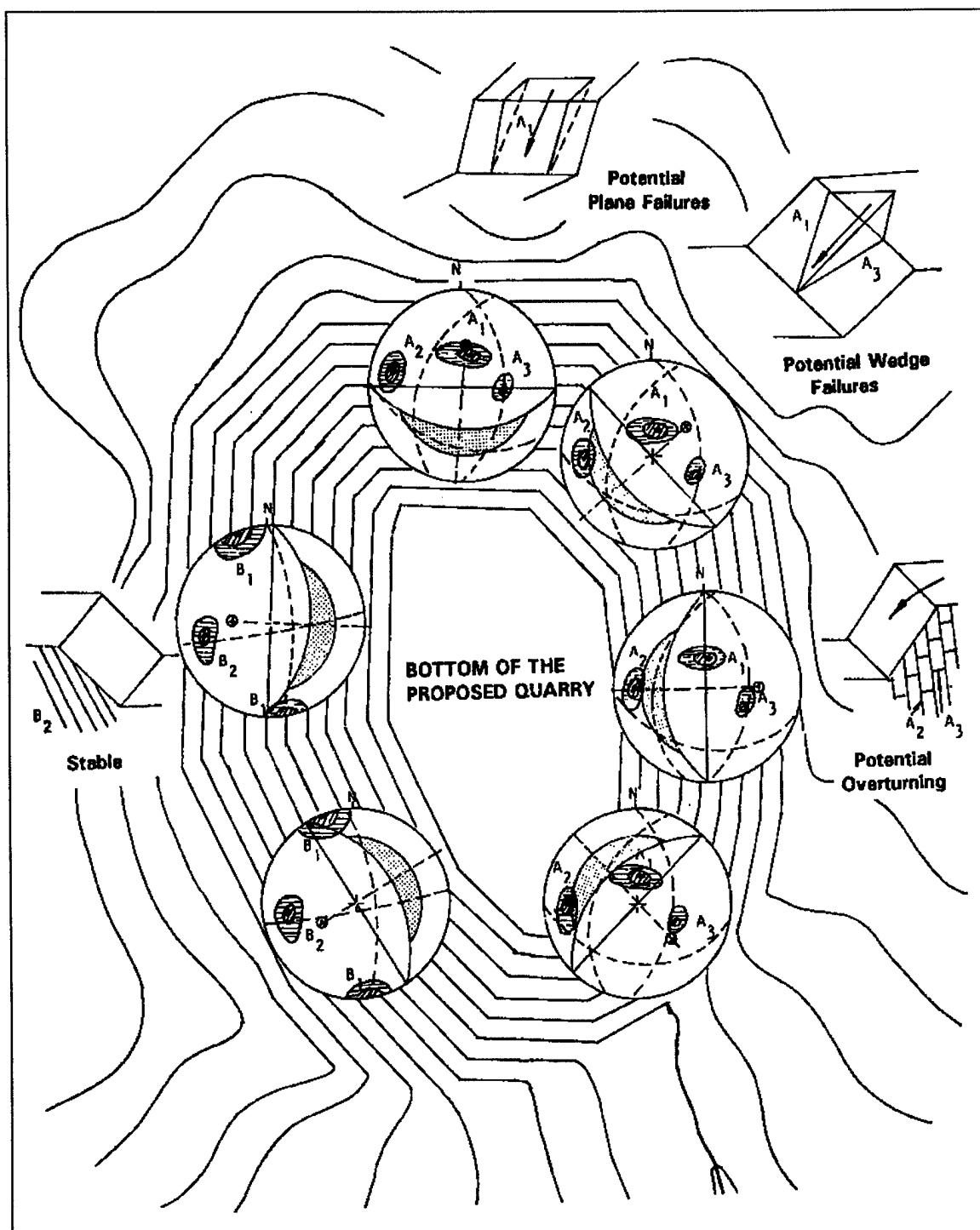
Figure 6-2. Example of a graphical slope stability evaluation of a proposed excavation (after Hoek and Bray 1981)
