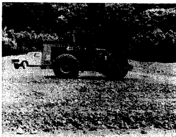
Figure 10-4. A 9.1 mg (10-ton) vibratory roller at work on the Cerrillos Dam test fill
