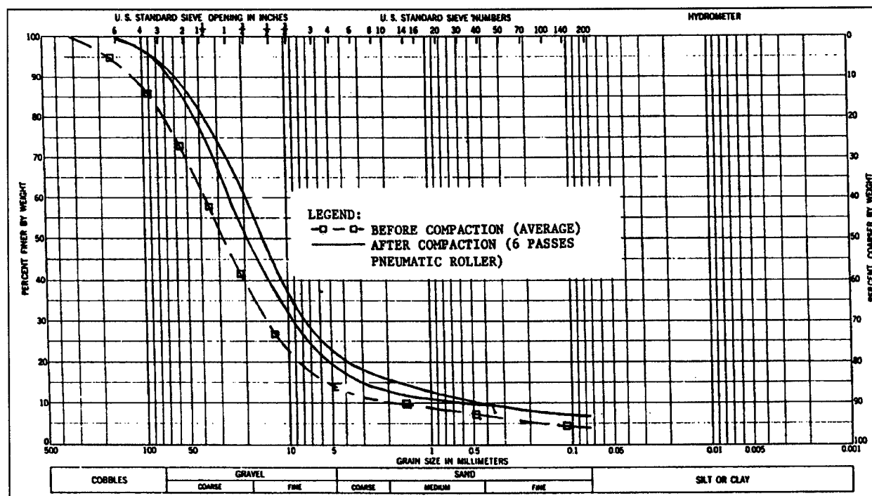
Figure 12-9. Before and after-compaction gradations after 6 passes of the pneumatic roller, quarry-run siltstone, Cerrillos Dam
