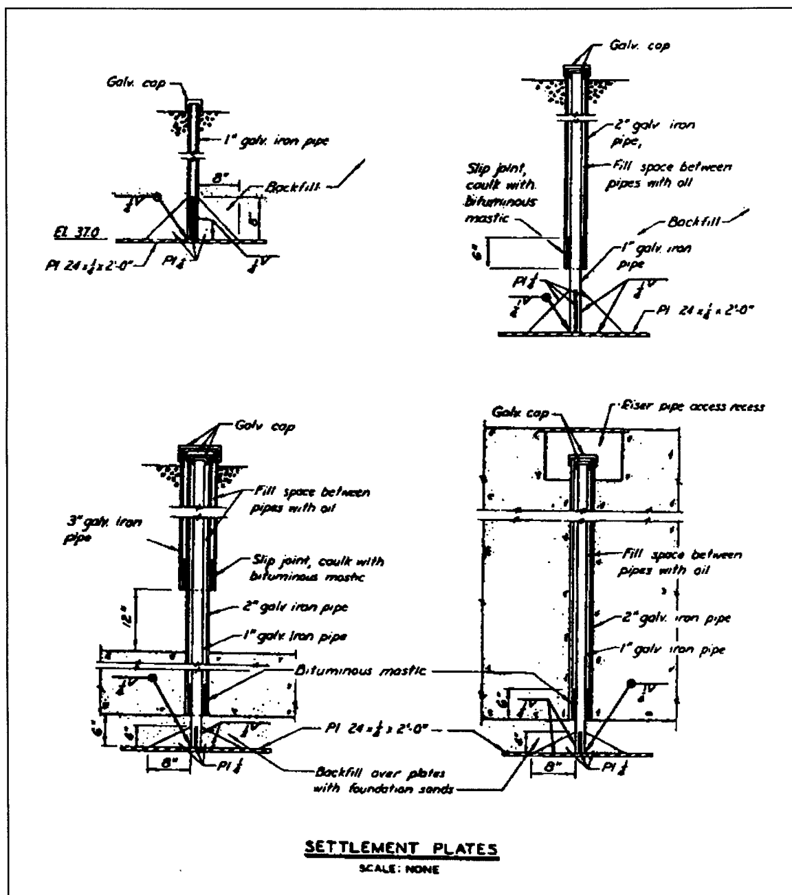
Figure 10-1. Typical settlement plates (from EM 1110-2-1908, Part 2)
