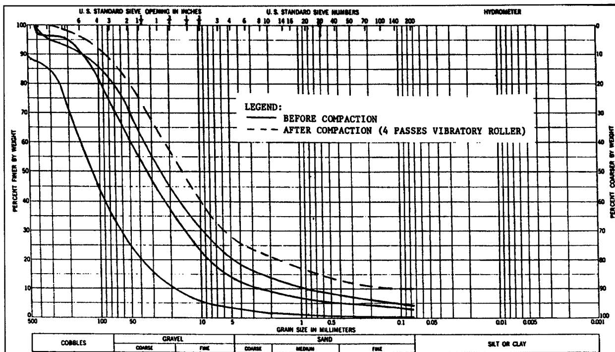
Figure 12-8. Before and after-compaction gradations after 4 passes of the vibratory roller, quarry-run siltstone, Cerrillos Dam
