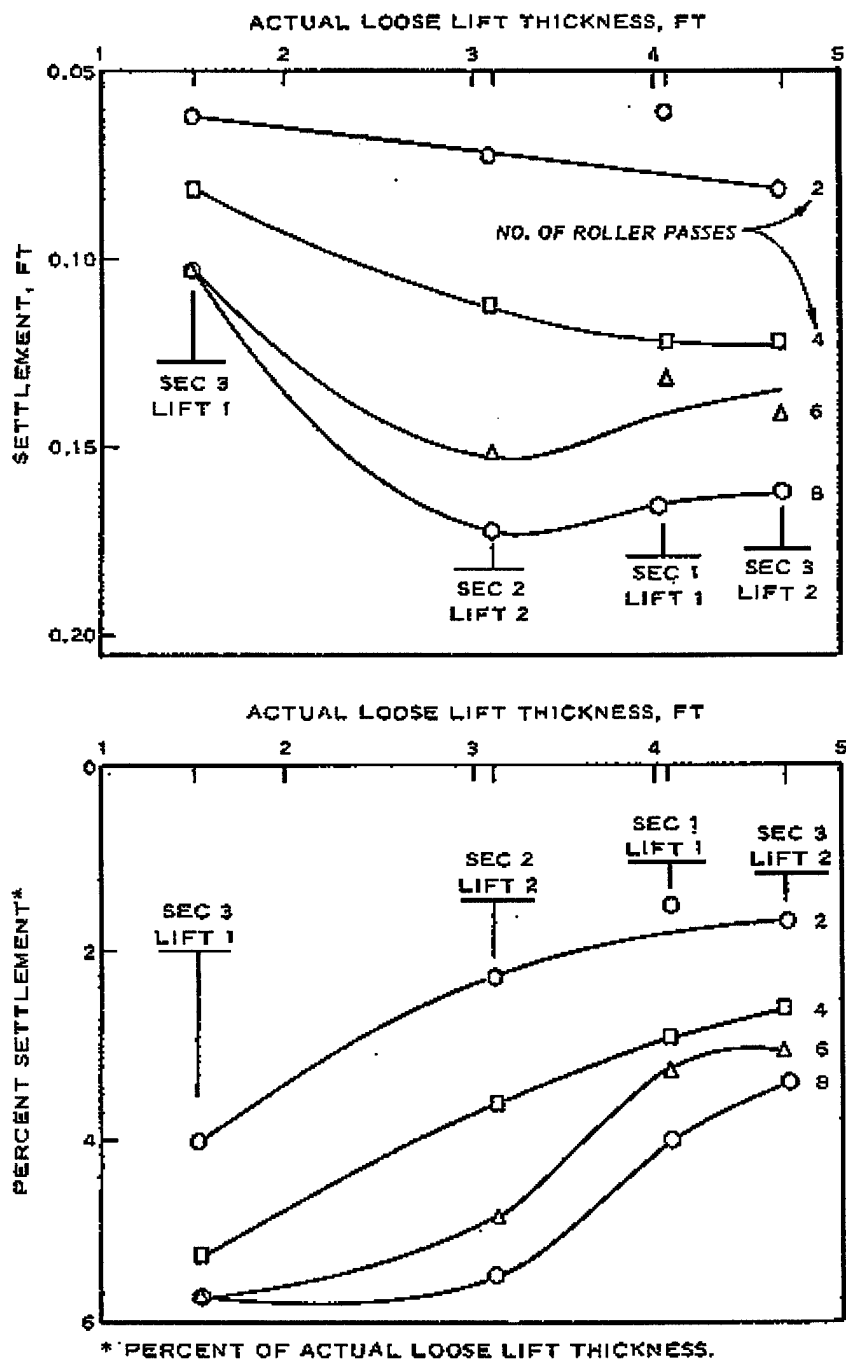
Figure 12-7. Percent settlement versus actual loose-fit thickness, Laurel Dam test fill
