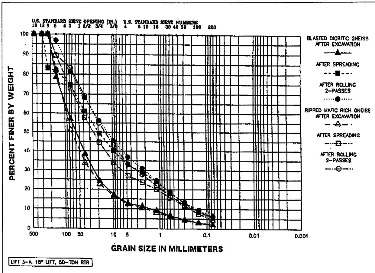
Figure 12-12. Change in gradation after 2 passes of 45.4-metric ton (50-ton) rubber-tired roller, 45.7 cm (18-in.) lift, Seven Oaks Dam materials
