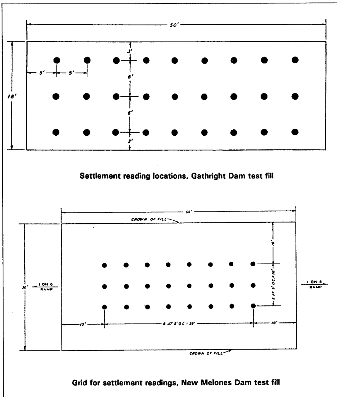
Figure 11-1. Example settlement grid layouts
