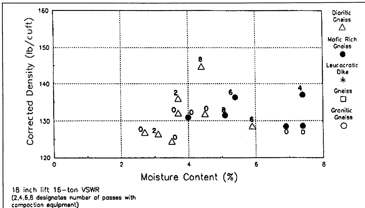
Figure 12-17. Corrected in situ densities, 45.7-cm (18-in.) lift, 14.5-metric ton (16-ton) vibratory roller, Seven Oaks Dam materials
