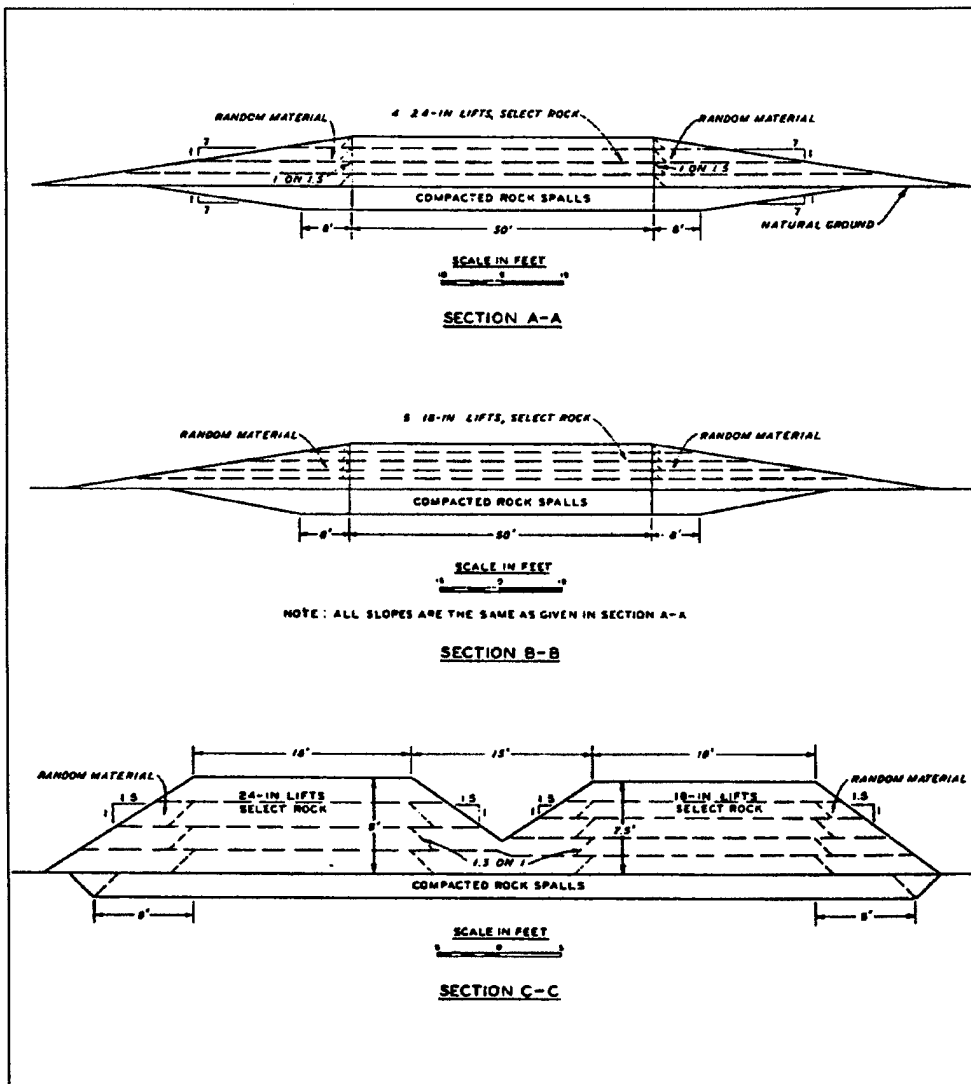
Figure 9-7. Gathright Dam, profiles of the test fills
