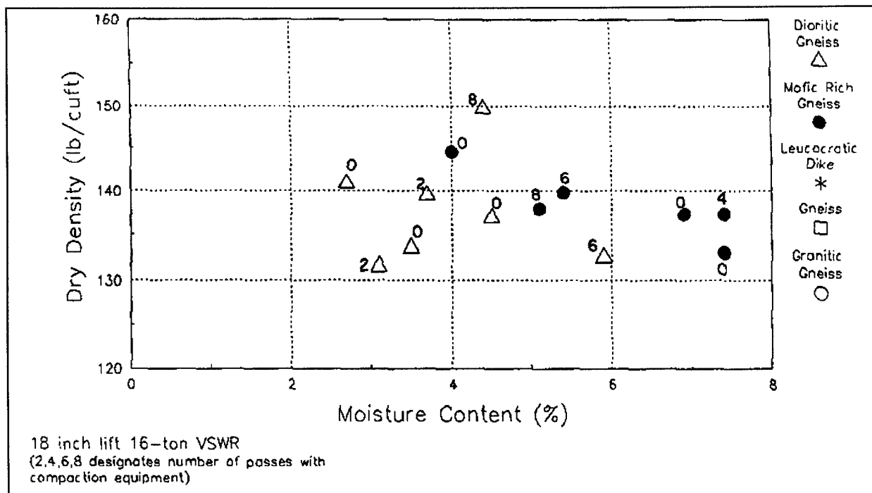
Figure 12-14. In situ density tests, 45.7-cm (18-in.) lift, 14.5-metric ton (16-ton) vibratory roller, Seven Oaks Dam materials
