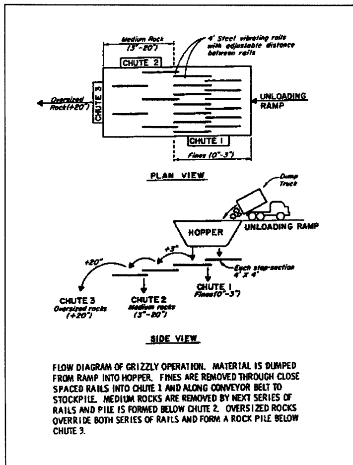
Figure 6-10. Flow diagram of a grizzly operation
