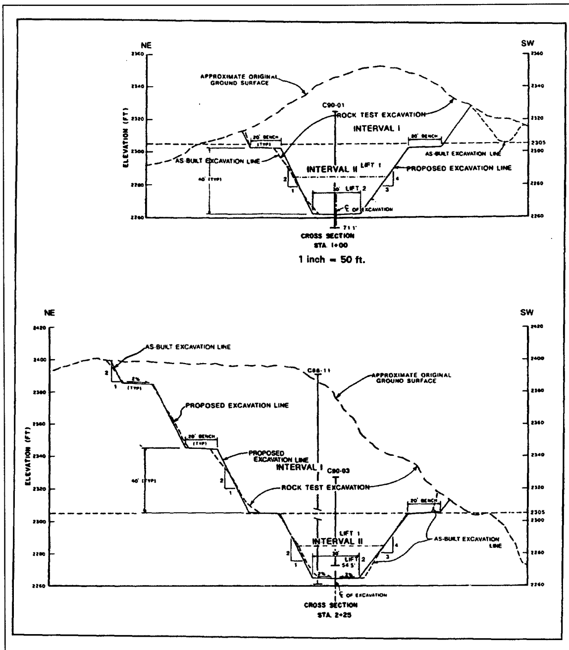
Figure 6-5. Additional sectional views of single quarry shown in Figure 6-3
